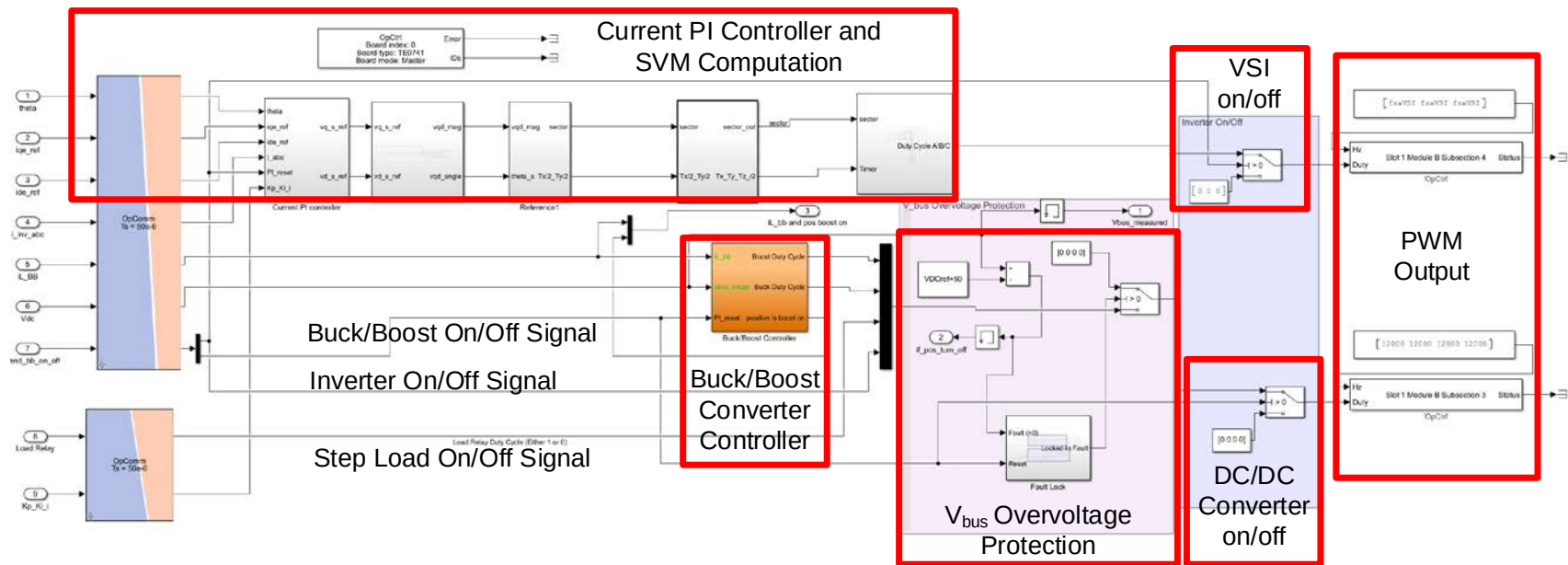
Figure 54. SM_INVERTER_AND_CONVERTER Subsystem
