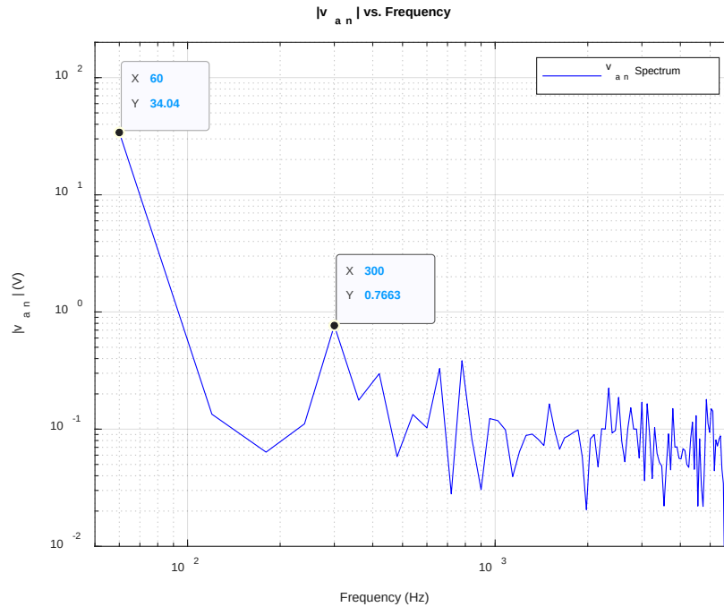
Figure 80. Step Load Decrease – |v_{an}| versus Frequency
