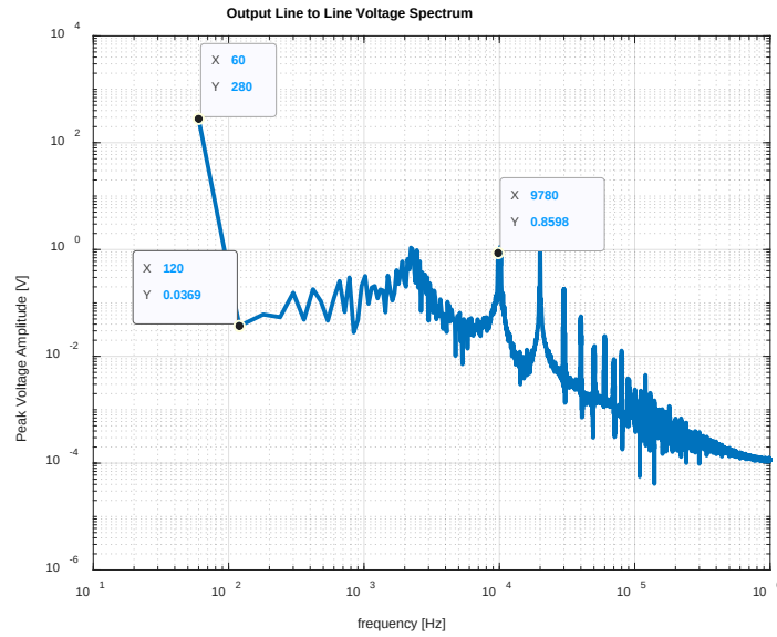
Figure 45. Multi-Step Simulated Load V_{LL} Spectrum, 200V rms , PWM
