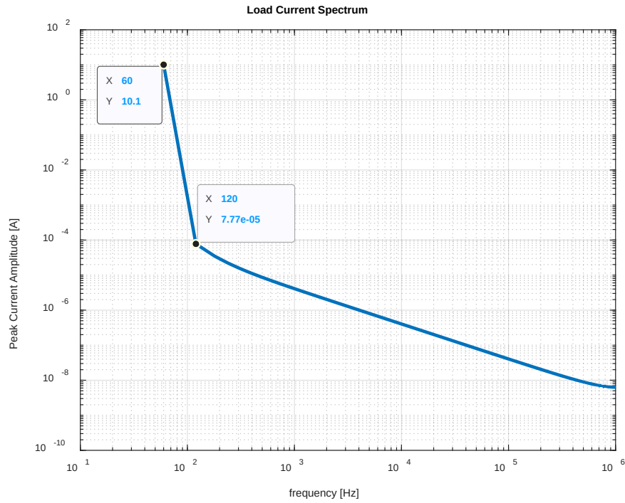
Figure 34. Multi-Step Simulated Load Current Spectrum, 200V rms , Ideal
