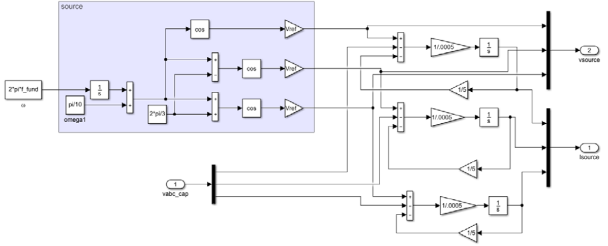
Figure 15. Grid Source Model
