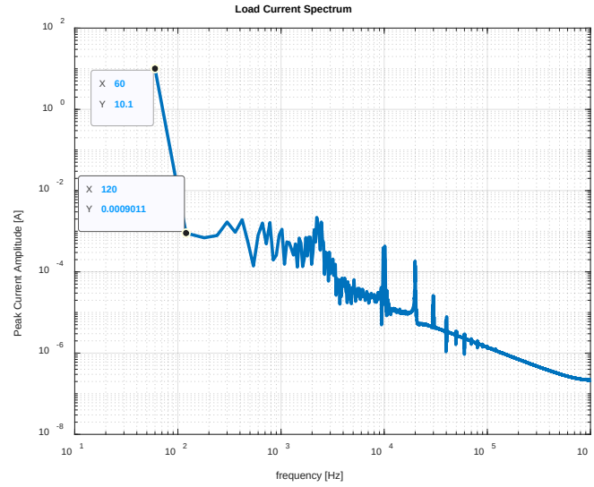
Figure 44. Multi-Step Simulated Load Current Spectrum, 200V rms , PWM
