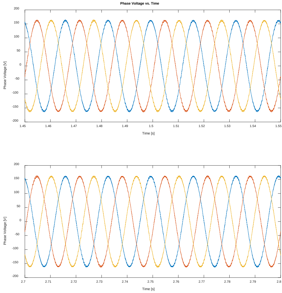
Figure 43. Multi-Step Simulated AC V_{PH} versus Time for First and Second Load Steps, 200V rms , PWM
