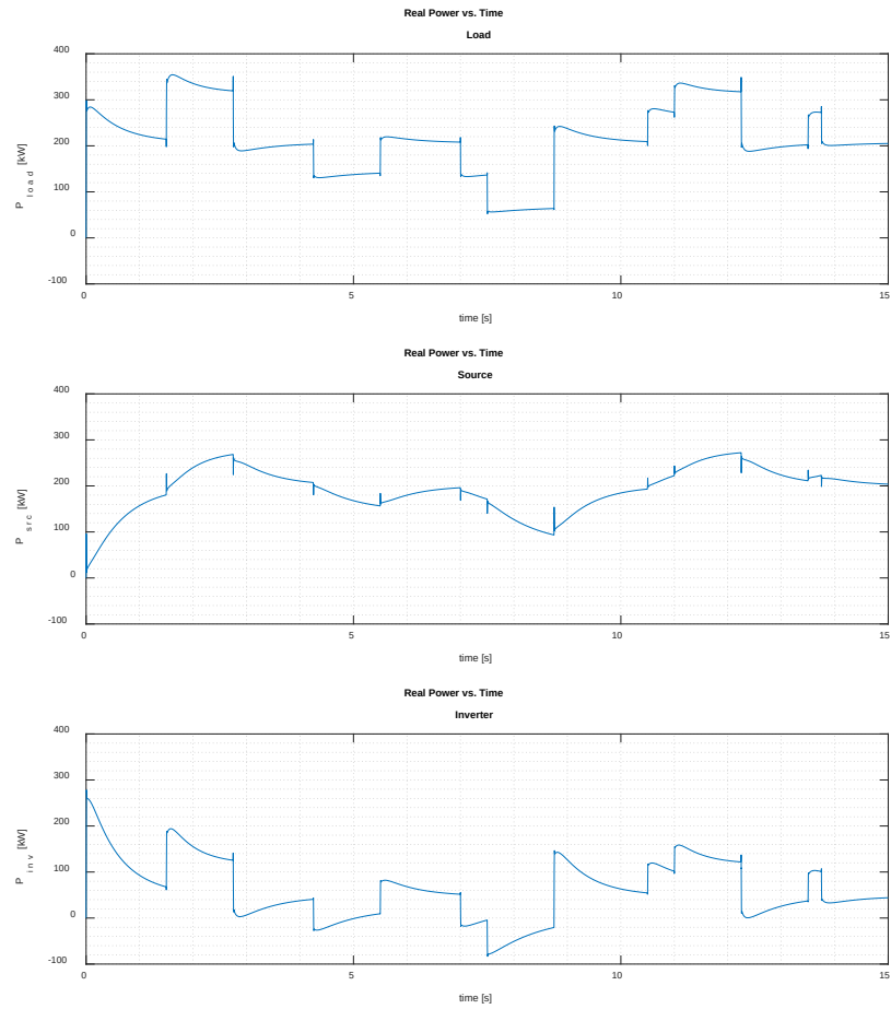
Figure 49. Multi-Step Simulated P versus Time, 440V rms , Ideal VSI, 1rad/s LPF
