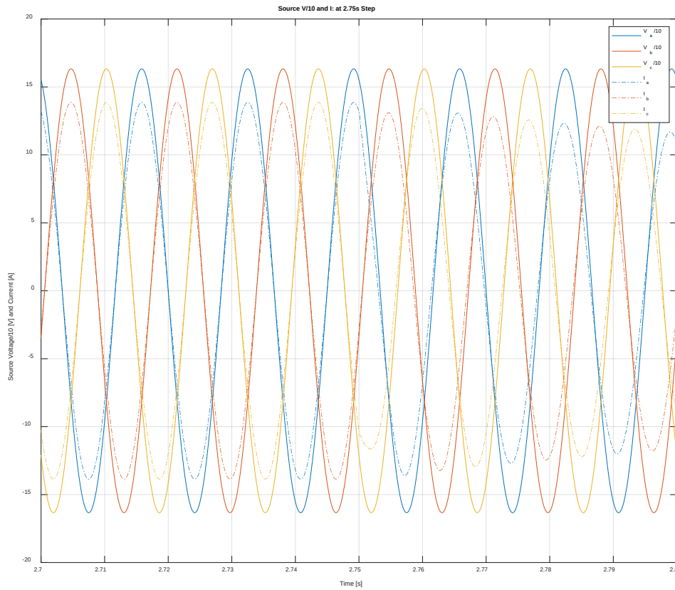
Figure 33. Multi-Step Simulated V/10 and Current versus Time, 200V_{rms} , Ideal, 2.75s Step
