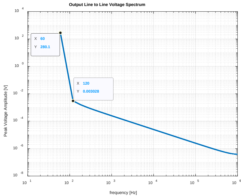
Figure 35. Multi-Step Simulated Load V LL Spectrum, 200V rms , Ideal
