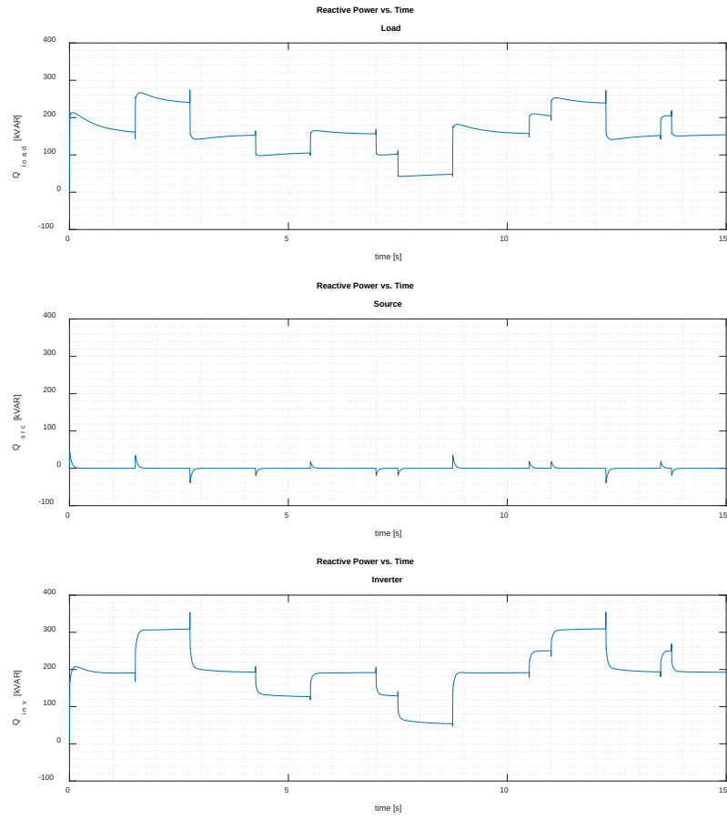
Figure 50. Multi-Step Simulated Q versus Time, 440V_{rms} , Ideal VSI, 1\text{rad/s} LPF
