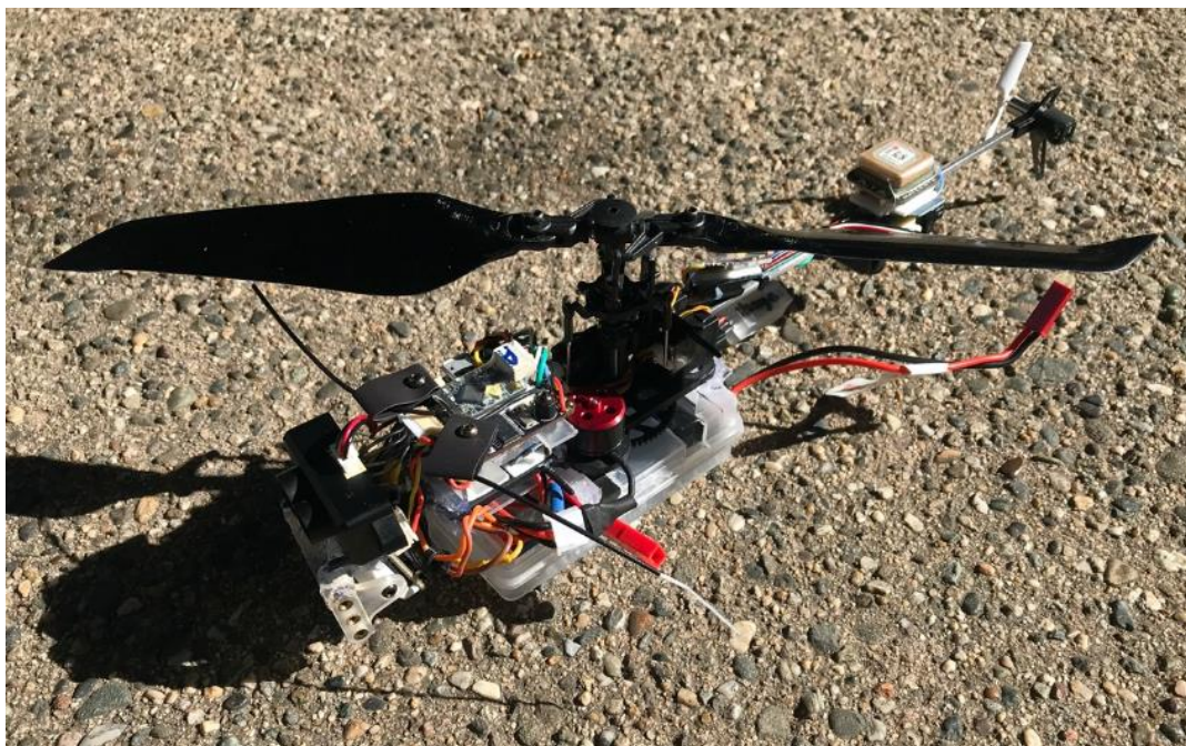
Figure 38. FRC COTS Drone Prototype (Side Angle View).
