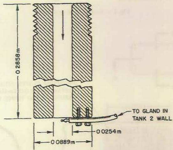
Fig. 4 - Sectional view of straight nozzle
