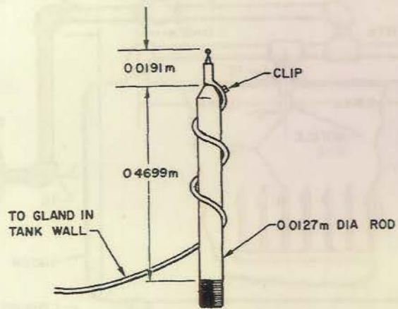
Fig. 3 - Thermocouple fixture
