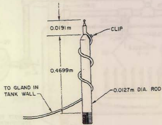
Fig. 3 - Thermocouple fixture
