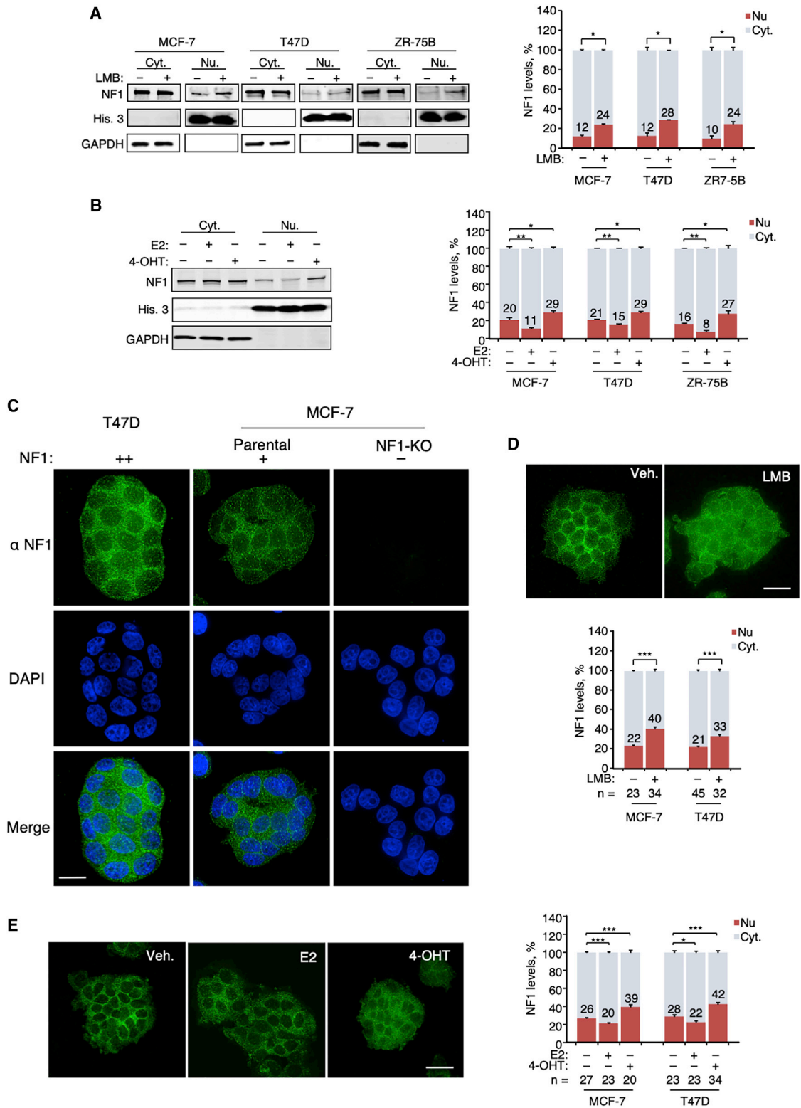
Figure 4. ER Ligand-Mediated Nuclear Accumulation of Neurofibromin
