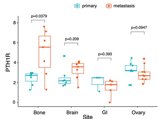
Fig. 3. PTH1R levels are particularly high in bone metastases. PTH1R mRNAs in paired primary vs metastasis in different organs were analyzed. PTH1R levels are particularly high in bone metastasis.
