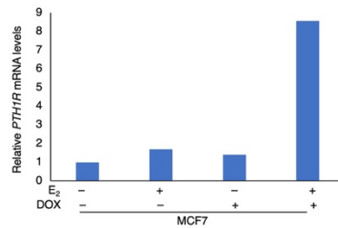
Fig. 1. PTH1R expression was highly induced after NF1-depletion in MCF-7 cell. MCF-7 cells carrying a DOX-inducible shRNA against NF1 were seeded in E2-deprived medium to which either vehicle or E2 was added. mRNA samples were made, and PTH1R levels were measured by qPCR.
