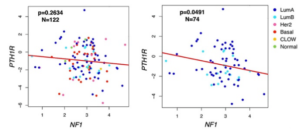
Fig. 2. Inverse correlation between NF1 and PTH1R levels in CPTAC prospective breast cancer database. Note the negative Pearson correlation is only statistically significant when luminal tumors were considered.
