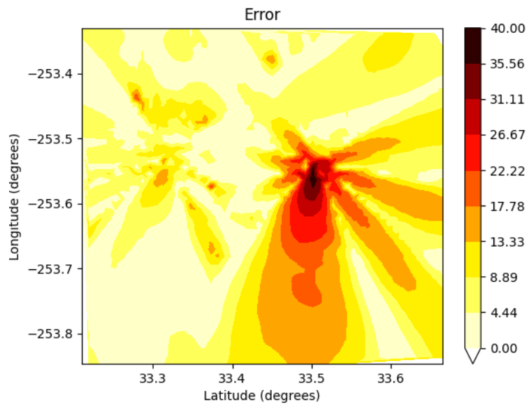
Figure 36: Double jammer ANN EMI environment prediction error.
