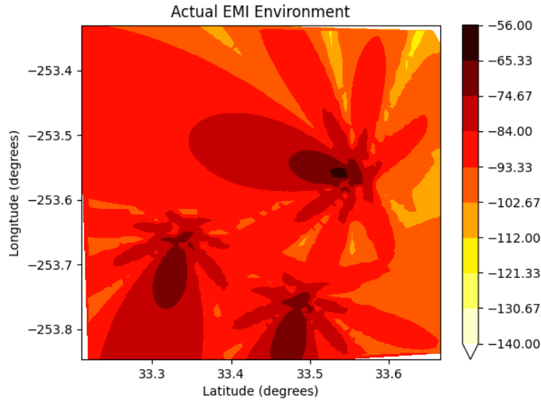
Figure 40: Triple Jammer Truth EMI.
