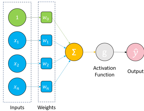
Figure 7: Perceptron Graphical Representation
