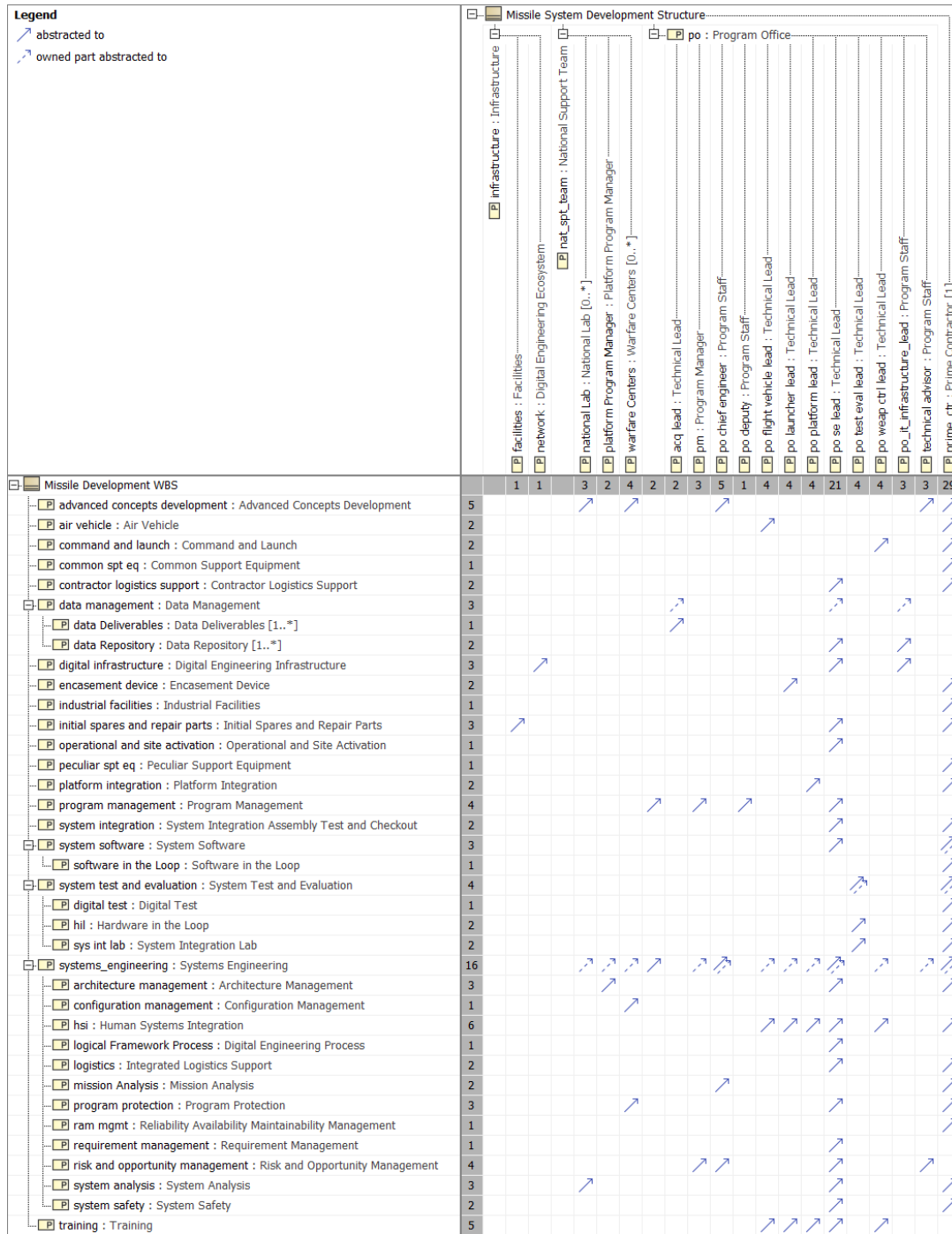
Figure 45. MBSE Framework Implementation to Logical Structure Mapping
