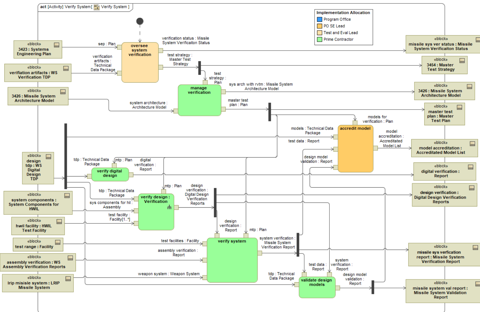
Figure 44. Activity Verify System with Implementation Allocations
