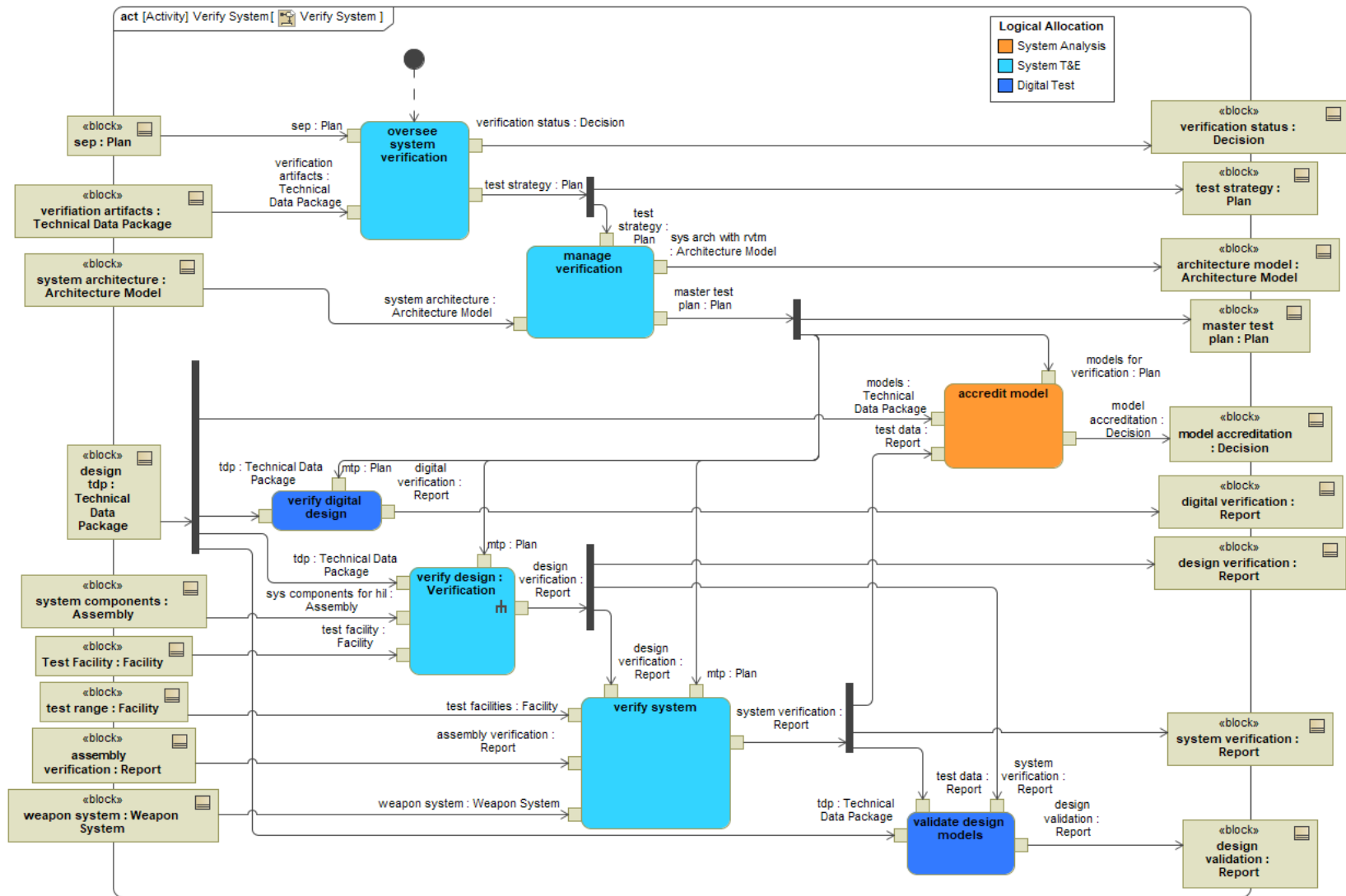
Figure 38. Activity Verify System with Logical Allocations
