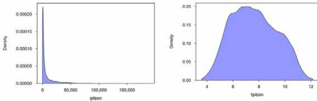
Figure 6. Logarithmic (log) Transformation Example 101
