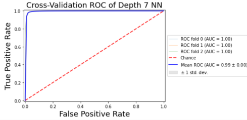
(a) 0% probability of measurement error
