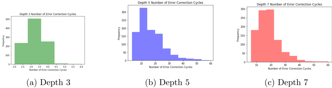
Figure 32: Distribution of number of error correction cycles for depths 3, 5, and 7
