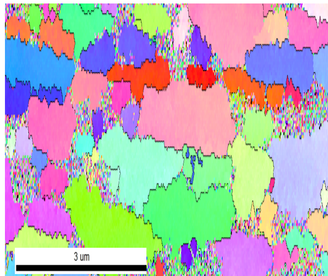
Fig. 31 EBSD map of the Al with significant noise caused by precipitate phases
