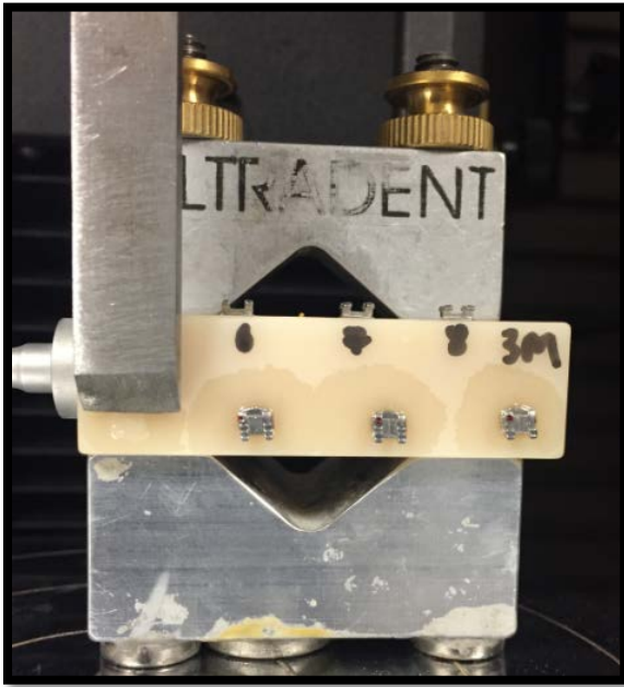
Figure 17: Increasing Force Applied until Bond Failure
