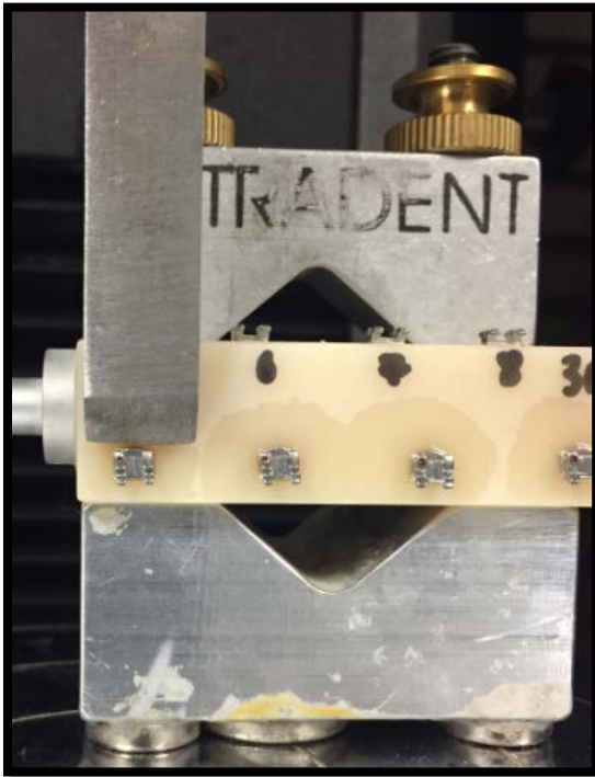
Figure 15: Instron Blade Lined Up Flush with Bracket Base
