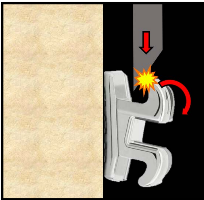
Figure 24: Incorrect Force Application: Instron Crosshead Applying Torqueing Force
