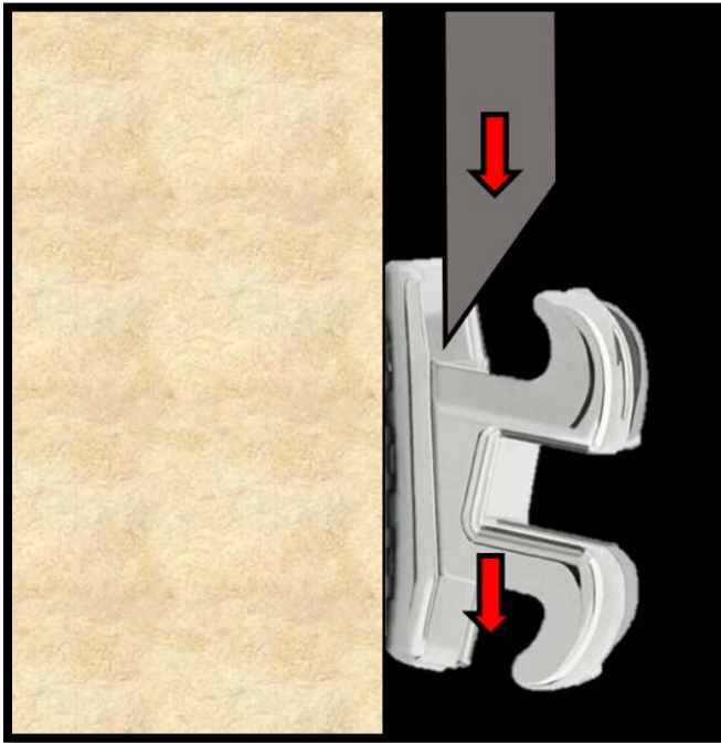
Figure 23: Correct Force Application: Instron Crosshead Applying Shearing Force
