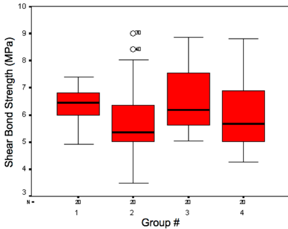
Figure 19: Shear Bond Strength Box Plot
