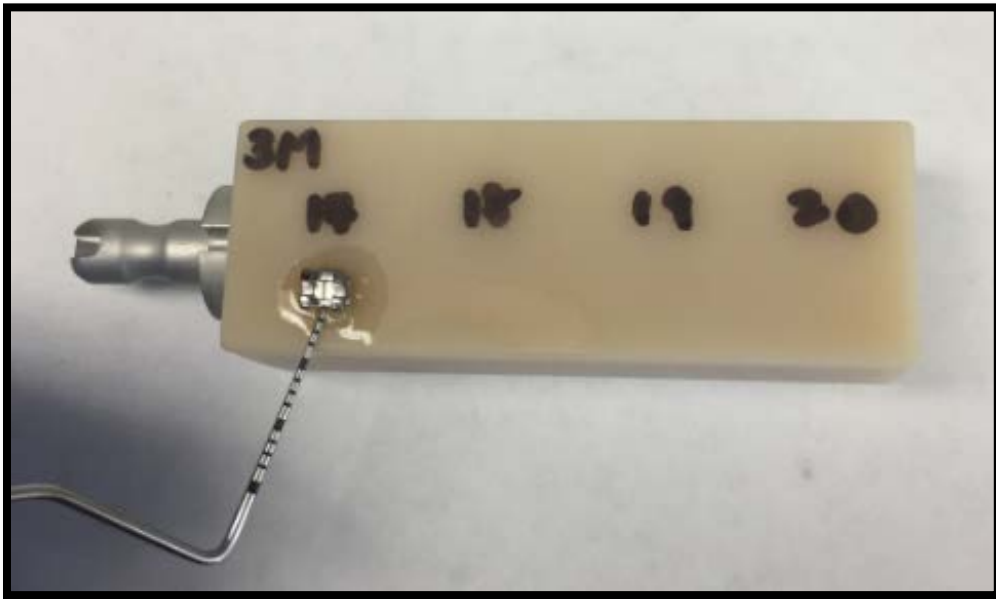
Figure 11: Bracket Placed on PMMA Surface and Excess Adhesive Composite Removed
