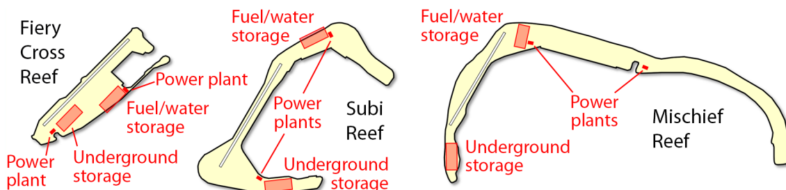
Figure 3. Locations of Underground Facilities and Power Plants
