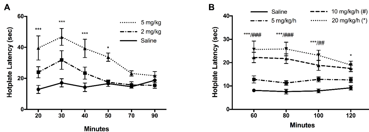
Figure 2.4. Effects of intravenous ketamine bolus and infusion on hotplate latency. A) Ketamine increased antinociception up to 50 min after a 5 mg/kg bolus injection. B) Ketamine 20 mg/kg/h induced significant antinociception through 120 min after the completion of a 1-h infusion. Ketamine 10 mg/kg/h induced antinociception through 100 min. Data are shown as mean \pm SEM. (* p < .05 , **/### p < .01 ; ***/#### p < .001 vs. saline; n = 8 per bolus group; n = 16 per infusion group).
