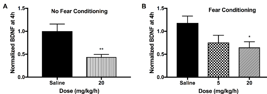
Figure 3.3. Effect of ketamine infusion on brain-derived neurotrophic factor (BDNF). BDNF was measured 2h after the conclusion of a ketamine infusion. A) Ketamine infusion (20 mg/kg/h x 2h) significantly decreased plasma BDNF concentration in rats that did not undergo fear conditioning. B) Ketamine infusion (20 mg/kg/h x 2h) significantly reduced plasma BDNF concentration among rats that experienced fear conditioning. Data are shown as mean \pm SEM (* p < 0.05 , ** p < 0.01 , n = 10-12 per group).
