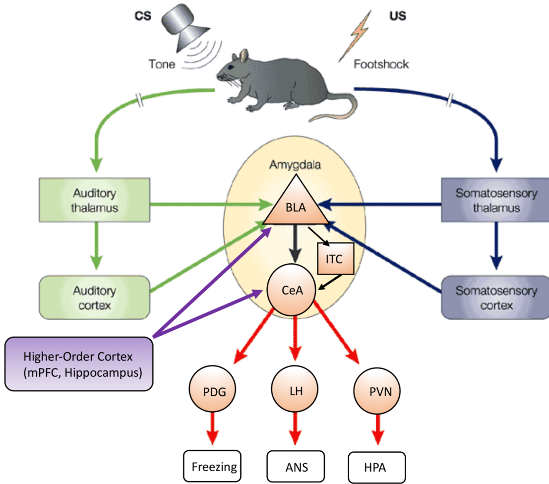
Figure 1.2 Neural Circuits during fear conditioning. CS and US stimuli converge onto the basolateral nucleus of the amygdala (BLA). Information is then transmitted to the intercalated cells (ITC) and central nucleus of the amygdala (CeA), which project to regions responsible for fear behaviors and physiologic responses (PDG: periaqueductal grey area, LH: lateral hypothalamus, PVN: paraventricular nucleus of hypothalamus, ANS: autonomic nervous system, HPA: hypothalamic-pituitary-adrenal axis). Higher-order cortex structures (mPFC: medial prefrontal cortex and hippocampus) also regulate amygdala dependent fear conditioning and behavioral response. Adapted from [80]
