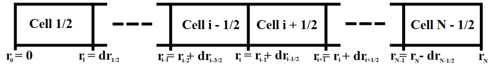
Figure 4. Visual representation of the finite volume indexing scheme used in this discretization of the neutron diffusion equation.
