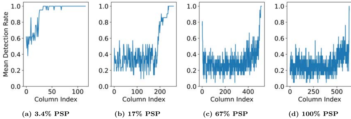
Figure 19. XPlorer Column Detection Rates. This data for the DVXPlorer’s response to the 771\text{cd}/\text{m}^2 stimulus shows that once 3.4% of columns were stimulated in (a), the left-most columns began responding to fewer stimuli. As a larger fraction of the array was stimulated, parts (b), (c), and (d) show fewer columns responding to every stimulus, and the diminished columns responding to fewer stimuli resulting in a progressively lower detection rate.
