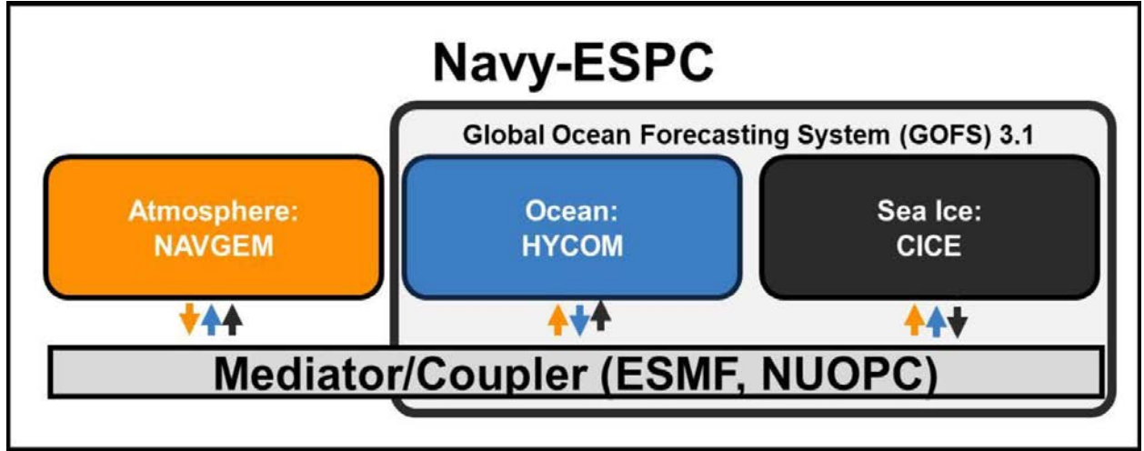
Figure 1 — Illustration of coupling between components of the Navy ESPC model. Reproduced from [2]
