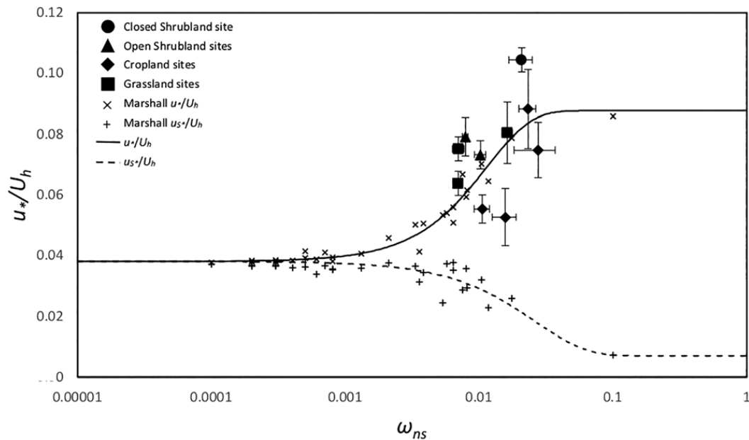
Figure 6. Profile-based u_*'/U_h plotted against normalized shadow, \omega_{ns} for the National Wind Erosion Network sites April through September 2018. Uncertainty (standard deviation) in profile estimates of u_*'/U_h is shown in the vertical error bars. Uncertainty (standard deviation) in \omega_{ns} is shown in the horizontal error bars. The u_*'/U_h (solid line) and u_{s*}'/U_h (dashed line) represent an idealized curve of the equations from the albedo model. The data Chappell and Webb (2016) used to calibrate the albedo model, from Marshall (1971) is also plotted. With a drag partition applied, Marshall's shear stress data shows a strong relationship between measured shear stresses (scaled by U_h ) and \omega_{ns} and trends with the albedo model.
