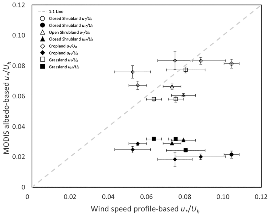
Figure 5. MODIS albedo-based u_*/U_h and u_{s*}/U_h plotted against wind speed profile-based u_*/U_h for the JER sites and the National Wind Erosion Network sites April through September 2018. Uncertainty (standard deviation) in MODIS estimates is shown in the vertical error bars. Uncertainty (standard deviation) in wind speed profile-based estimates is shown in the horizontal error bars. The 1:1 line shows the relation between MODIS albedo-based and wind speed profile-based estimates, revealing that the latter most closely estimates the u_*/U_h at the sites.
