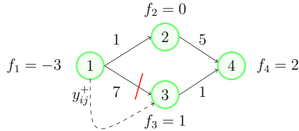
Figure 10. Disrupted Arc not Restored
