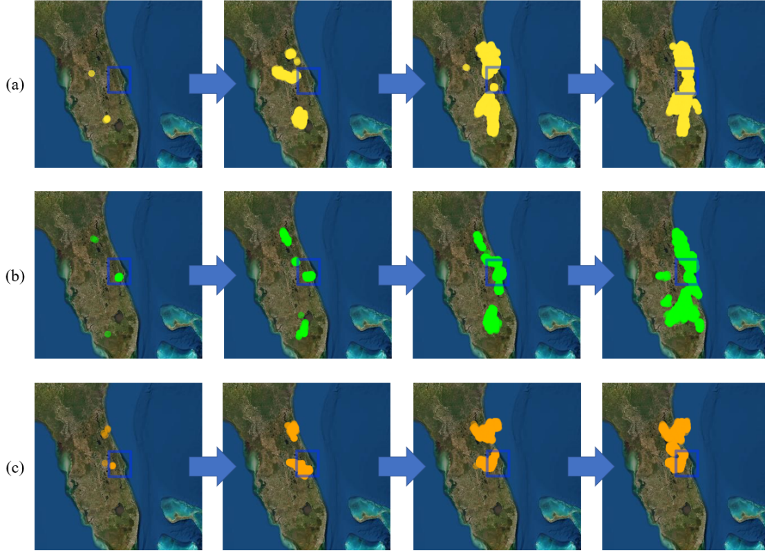
Figure 4.2. Examples of storms merging over time. For each subfigure (each row of images), CODAS has assigned all visible data to the same macrocluster. The blue box indicating MERLIN sensors, included for reference, measures 45.1 NM by 52.9 NM.
