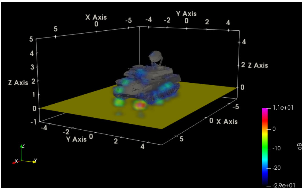
Fig. 45 ParaView HH SAR for 30° azimuth-inc on ZSU, radar view
