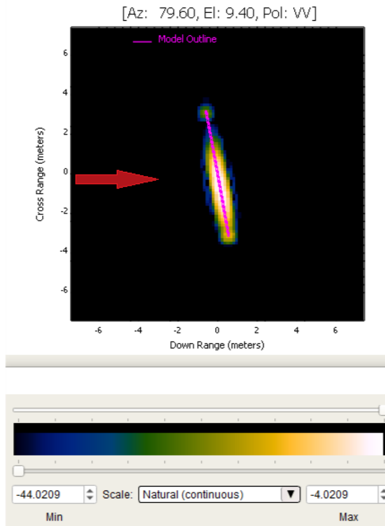
Fig. 21 Catalus VV SAR image (dB) of free-space twisted line at 79.6^\circ azimuth with radar from left
