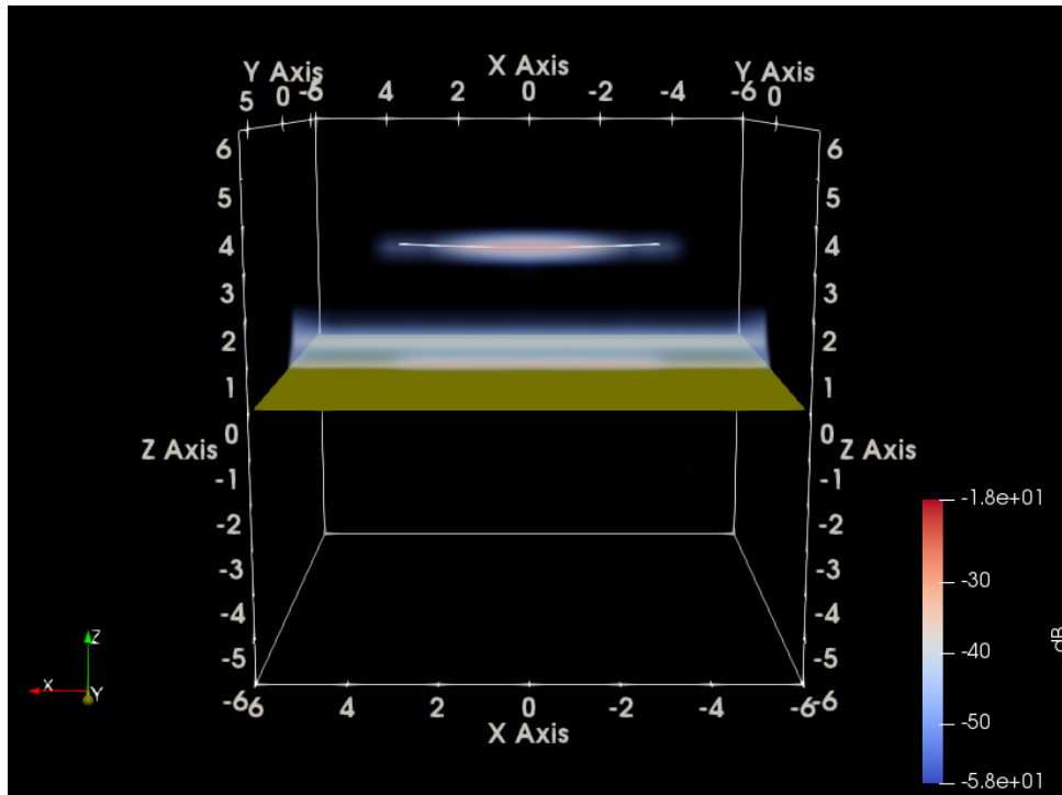
Fig. 14 ParaView 89.6° azimuth-inc HH radar-view image from twisted line (overlaid) over ground
