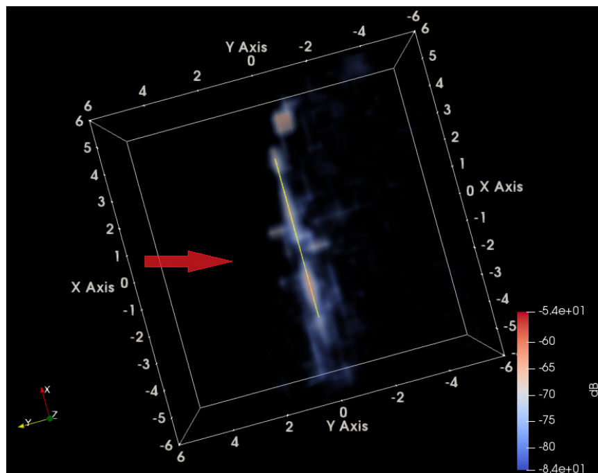
Fig. 26 ParaView HH SAR of twisted line over ground with 74.6^\circ azimuth-inc, top down
