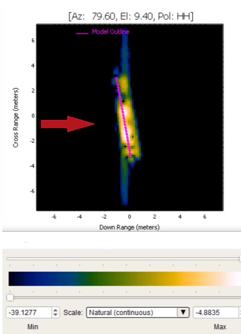
Fig. 22 Catalus HH SAR image (dB) of twisted line over ground at 79.6^\circ azimuth with radar from left
