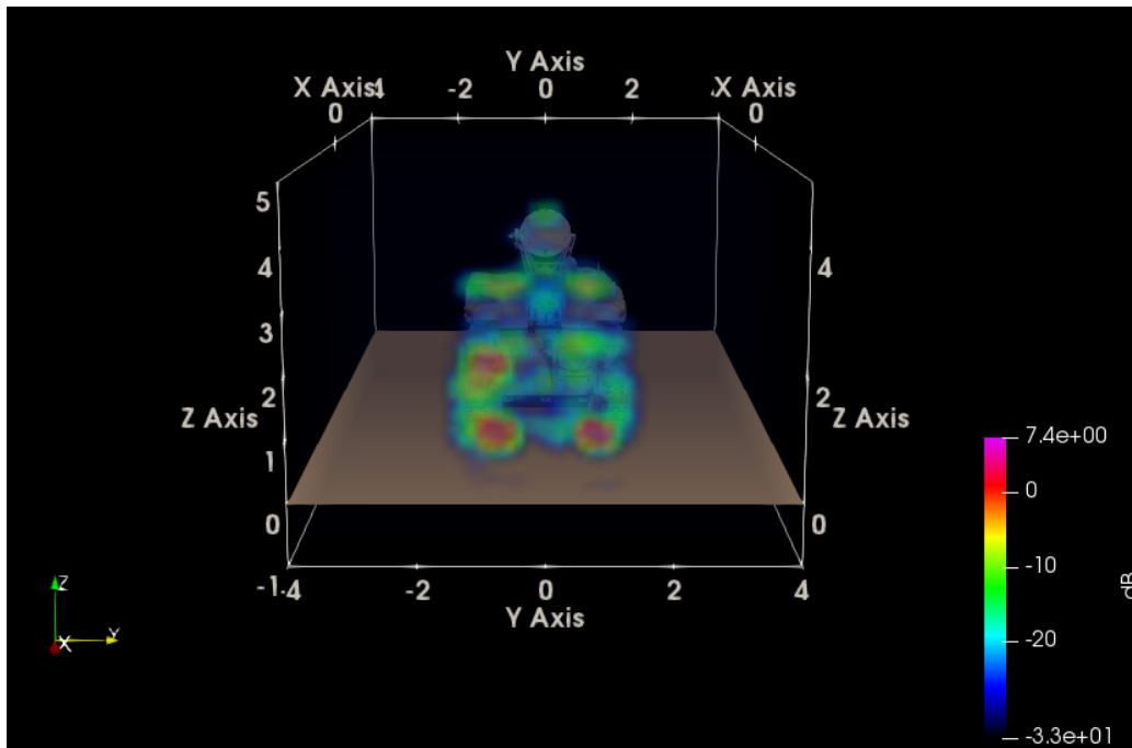
Fig. 47 ParaView VV SAR for 0° azimuth-inc on ZSU, radar view
