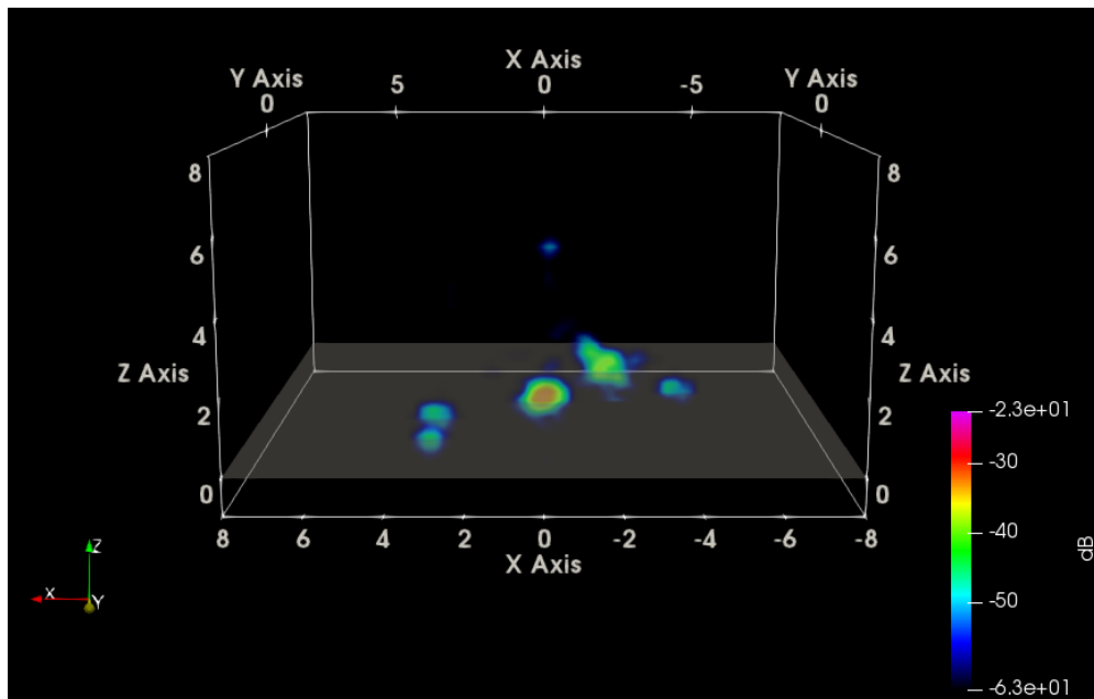
Fig. 60 Radar-view HH SAR of five boulders with rough ground RMS bump height = 10 cm
