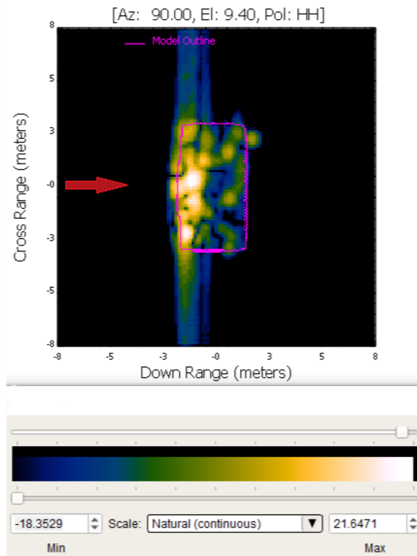
Fig. 29 Catalus free-space HH SAR (dB), broadside-inc against ZSU
