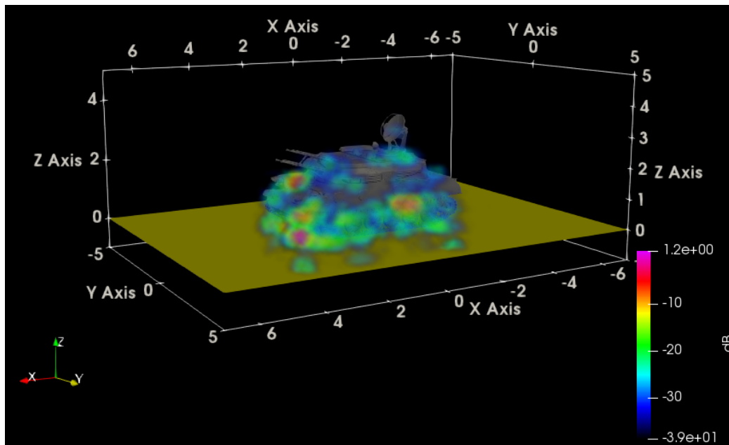
Fig. 39 ParaView HH SAR; 60° azimuth-inc (dB) on ZSU over flat ground, radar view
