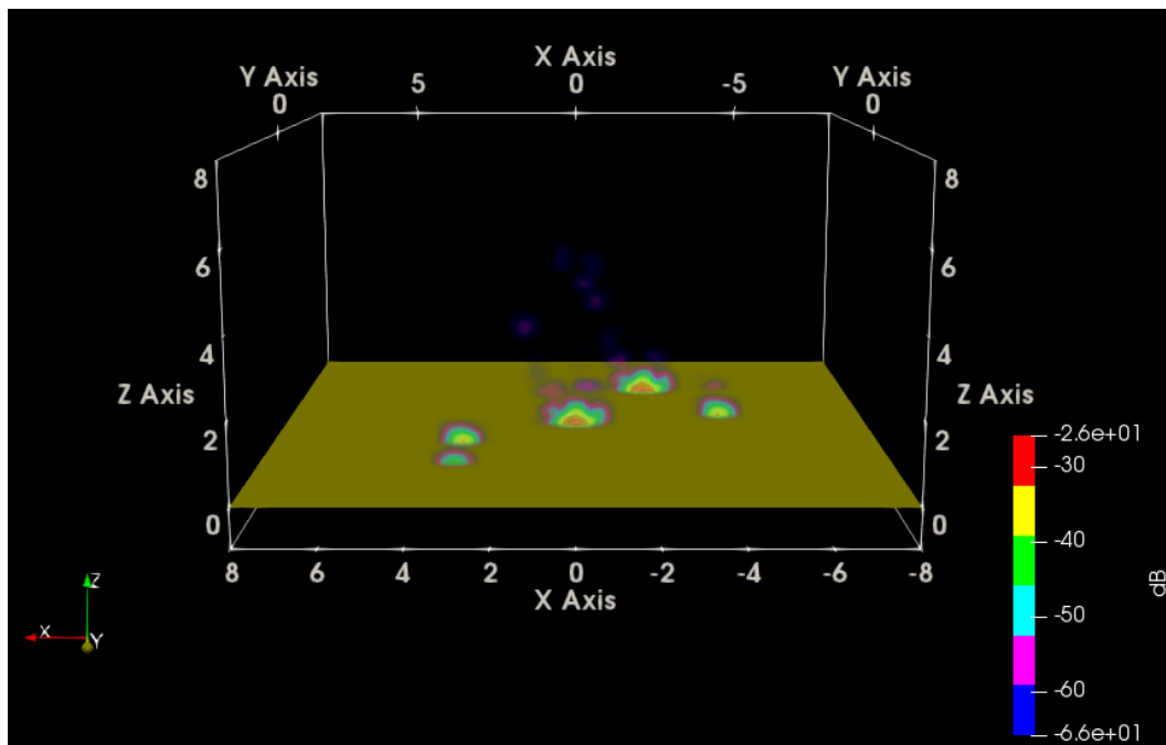
Fig. 52 ParaView HH SAR of boulder field, radar view
