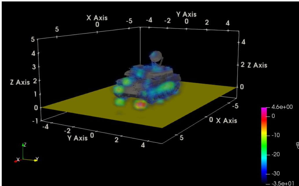
Fig. 46 ParaView VV SAR for 30° azimuth-inc on ZSU, radar view
