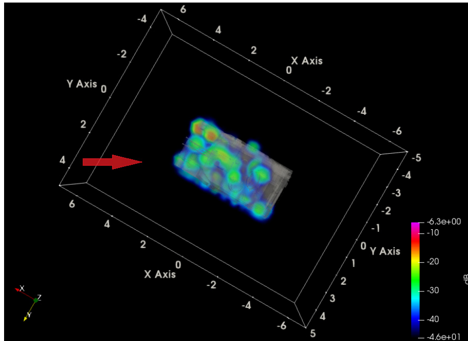
Fig. 42 ParaView HH SAR for 30° azimuth-inc on ZSU in free space, top-down view
