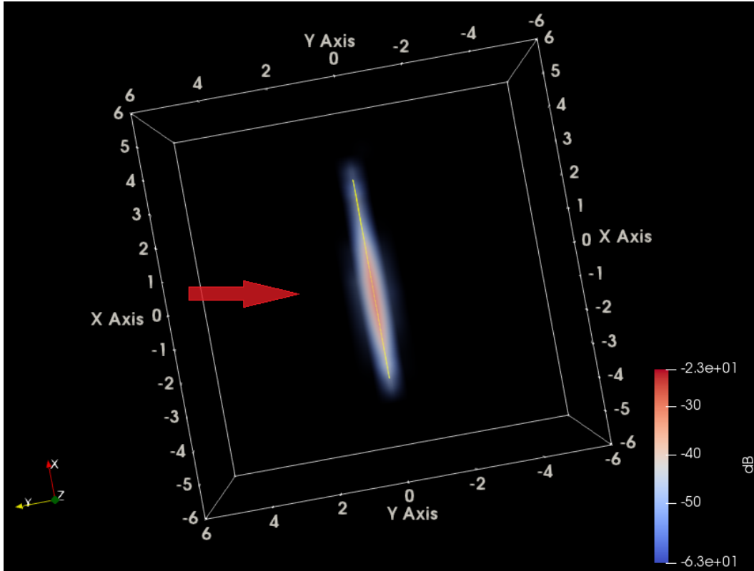
Fig. 23 ParaView HH image of twisted line at 79.6^\circ azimuth-inc, top down, tilted toward radar
