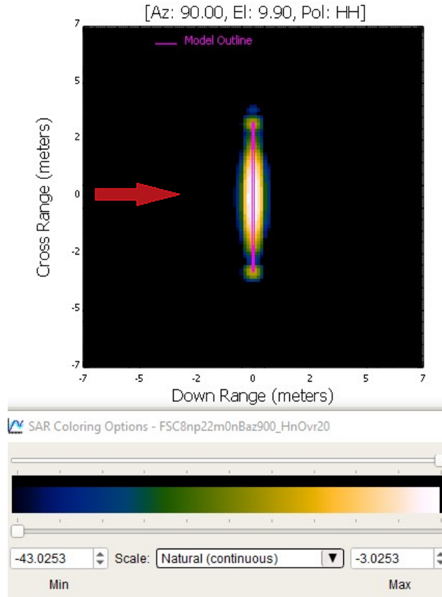
Fig. 12 Catalus 89.6° azimuth-incidence (inc) HH SAR image (dB) from twisted line in free space with radar from left
