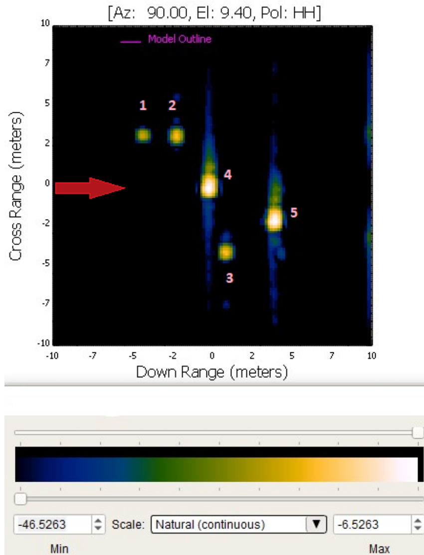
Fig. 55 Catalus HH SAR of boulder field over ground
