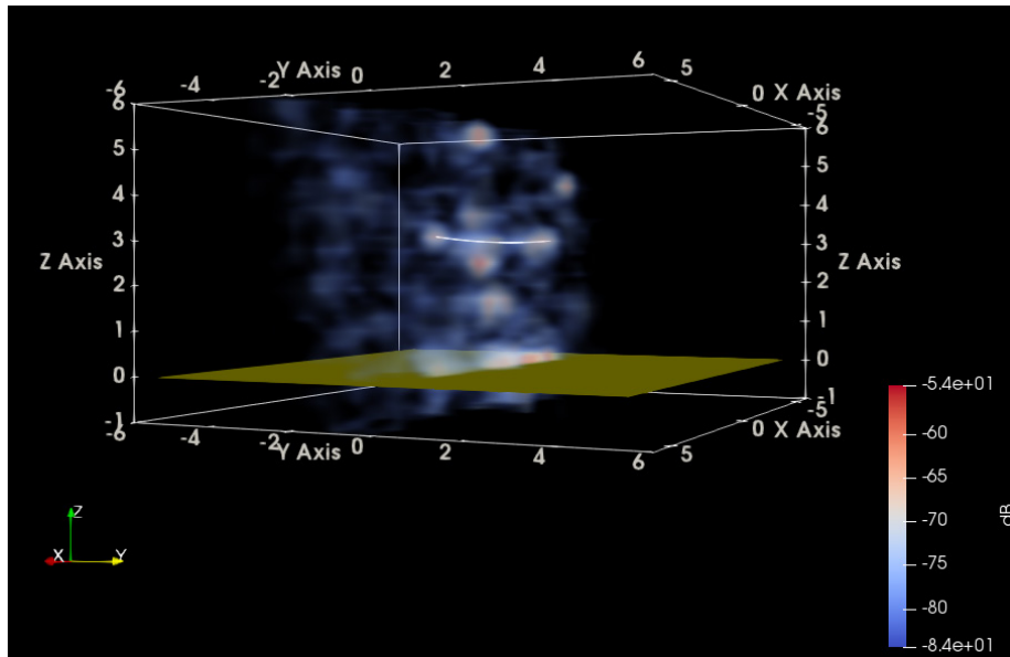
Fig. 20 ParaView VV image of twisted line at 84.5° azimuth side view
