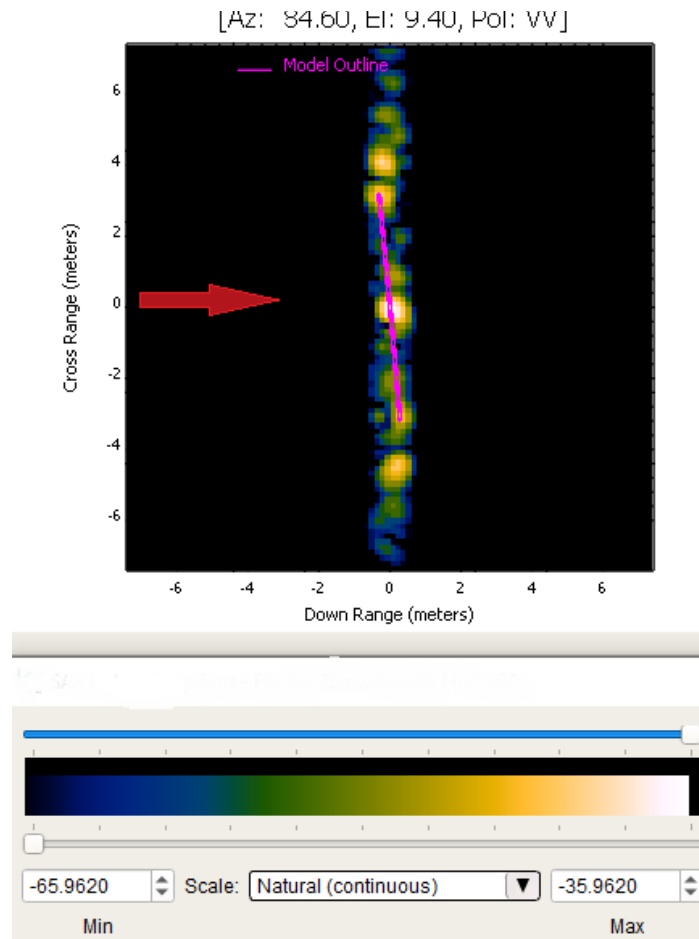
Fig. 16 Catalus HH image (dB) of free-space twisted line at 84.6° azimuth-inc with radar incident from the left
