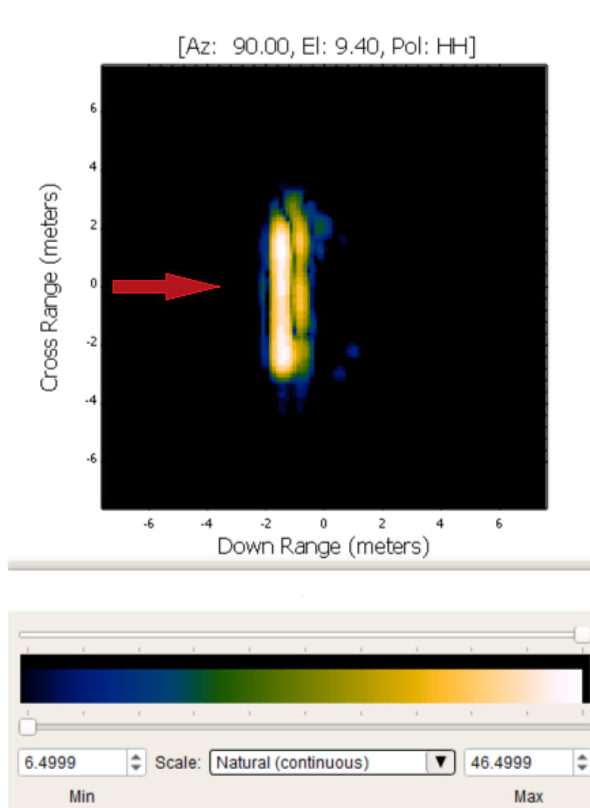
Fig. 30 Catalus HH SAR (dB) broadside-inc against ZSU over flat ground
