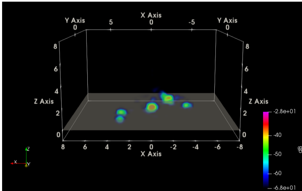
Fig. 62 Radar-view VV SAR of five boulders with rough ground RMS bump height = 10 cm
