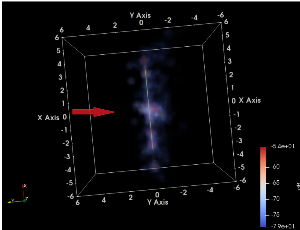
Fig. 17 ParaView top-view HH image of twisted line over ground at 84.6^\circ azimuth-inc with radar incident from the left
