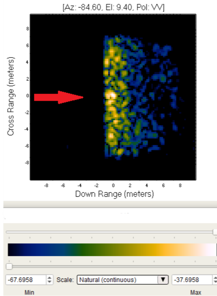
Fig. 18 Catalus VV SAR image of twisted line at 84.6^\circ azimuth over ground
