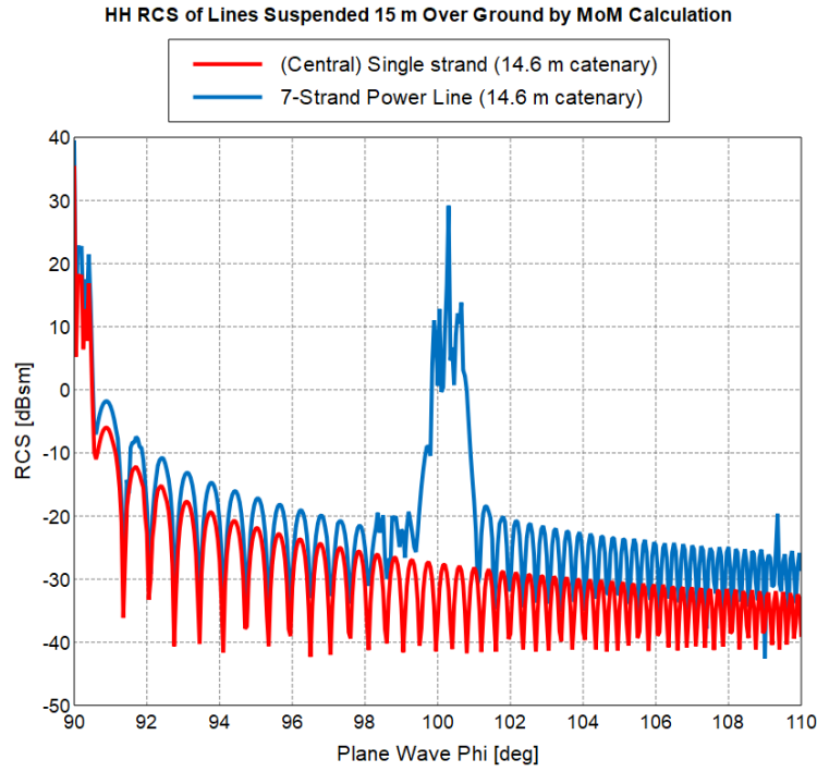
Fig. 10. HH RCS for single strand vs. six twisted strands at 35 GHz
