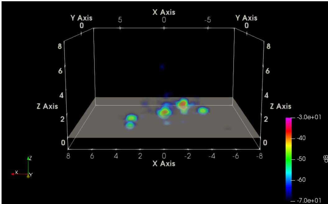
Fig. 64 Radar-view VV SAR of five boulders with rough ground RMS bump height = 15 cm
