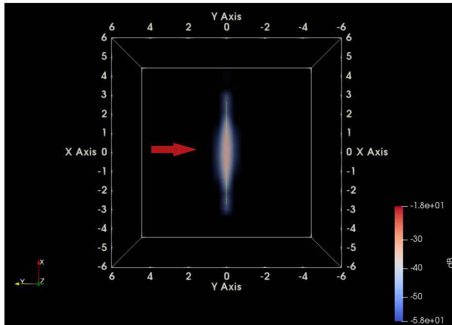
Fig. 13 ParaView top-view 89.6° azimuth-inc HH image from twisted line (overlaid) in free space with radar from the left
