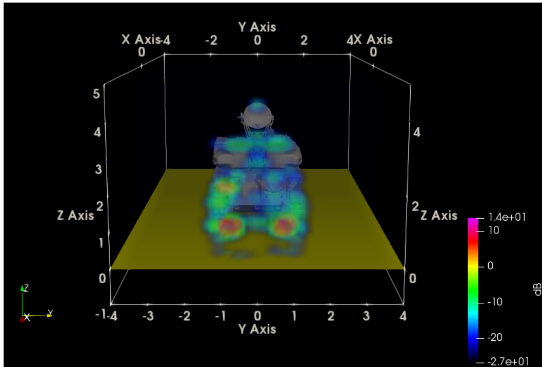
Fig. 48 ParaView HH SAR for 0° azimuth-inc on ZSU, radar view
