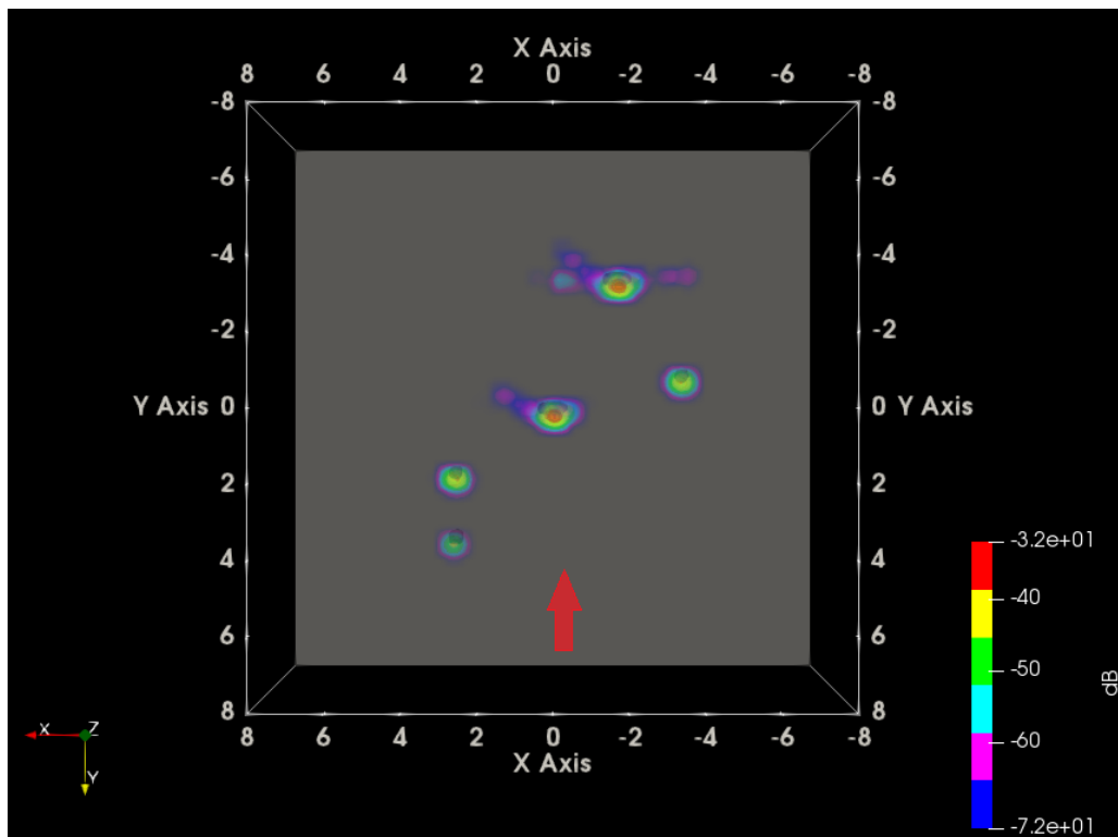
Fig. 54 ParaView VV SAR top-down view with boulders overlaid (bubble-like)
