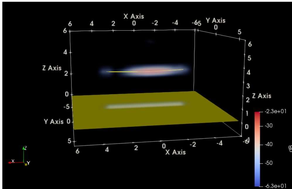
Fig. 24 ParaView HH image of twisted line at 79.6^\circ azimuth, radar view
