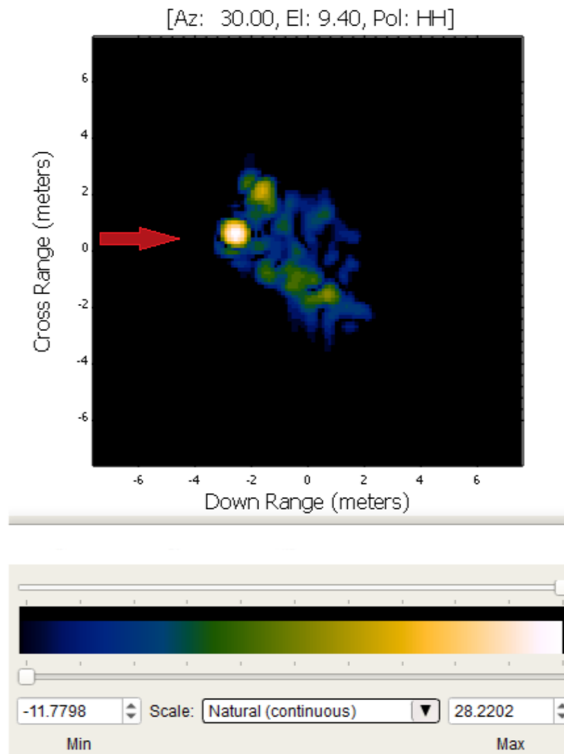
Fig. 41 Catalus HH SAR image (dB) of ZSU over ground; azimuth-inc at 30^\circ (radar from the left)
