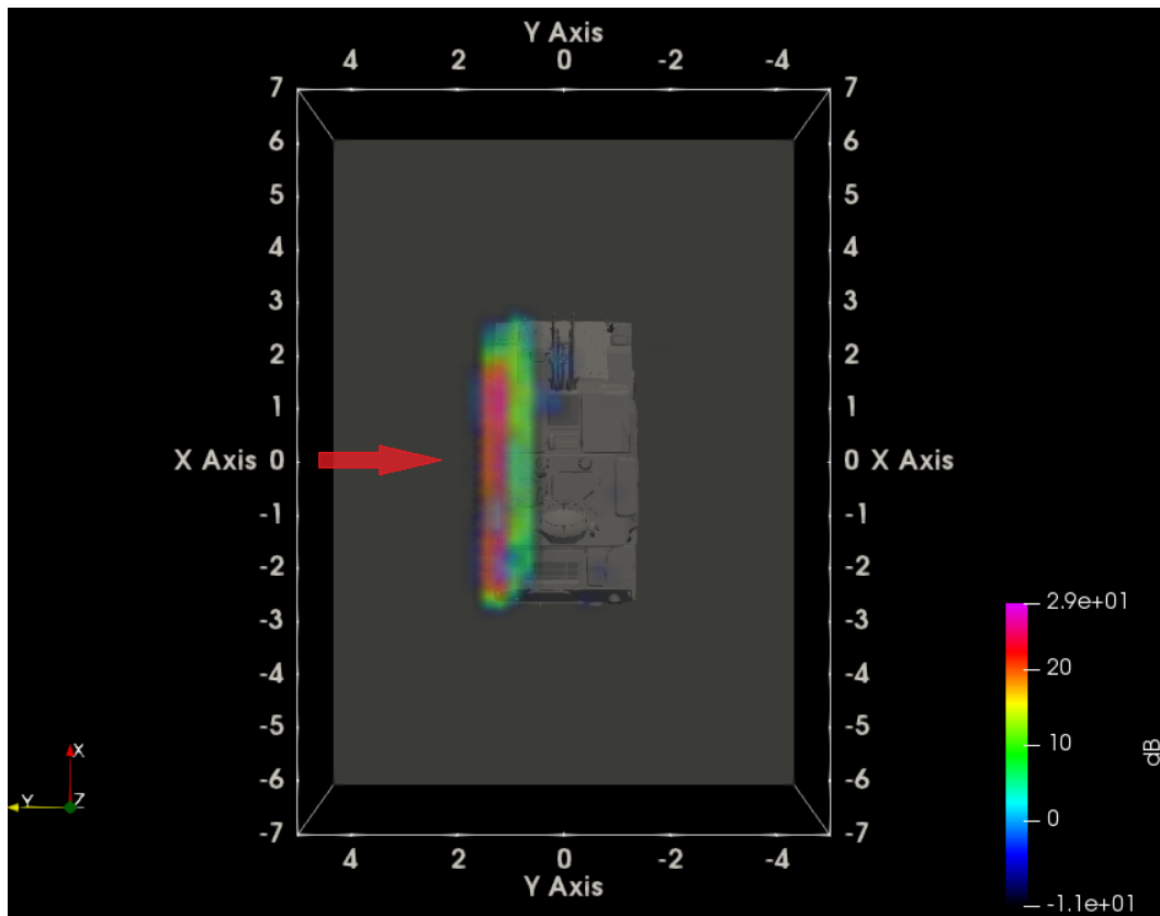
Fig. 32 ParaView HH SAR broadside-inc against ZSU over ground, top-down view
