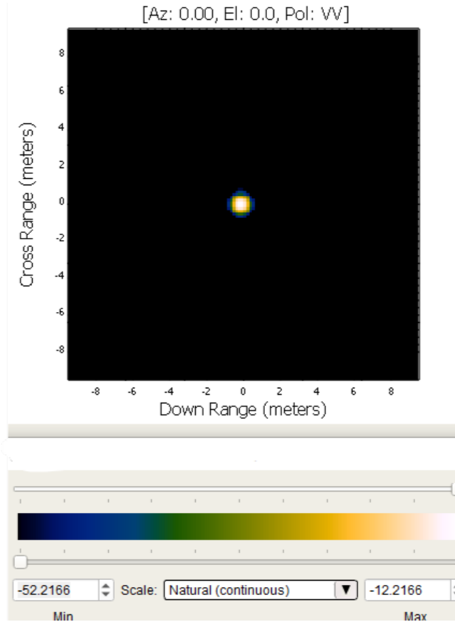
Fig. 8 Catalus SAR image (dB) of 0.25-m radius PEC sphere in free space
