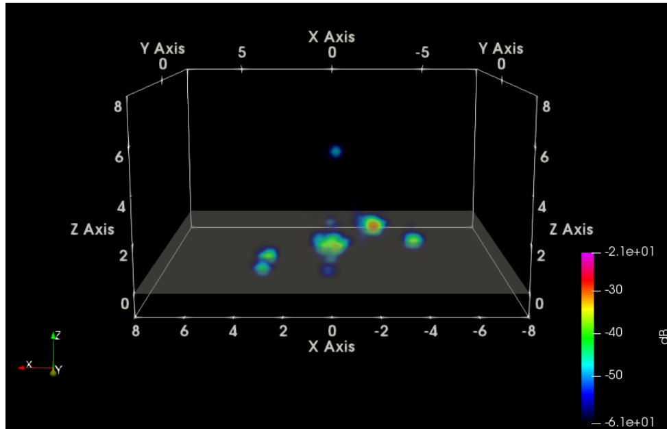
Fig. 57 Radar-view HH SAR of five boulders with rough ground RMS bump height = 1 cm
