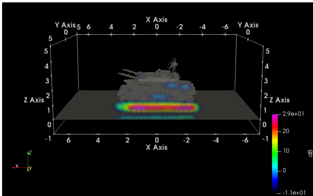
Fig. 34 ParaView HH SAR (dB), broadside-inc against ZSU, radar view
