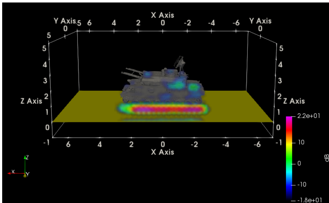
Fig. 33 ParaView VV SAR, broadside-inc on ZSU, radar view
