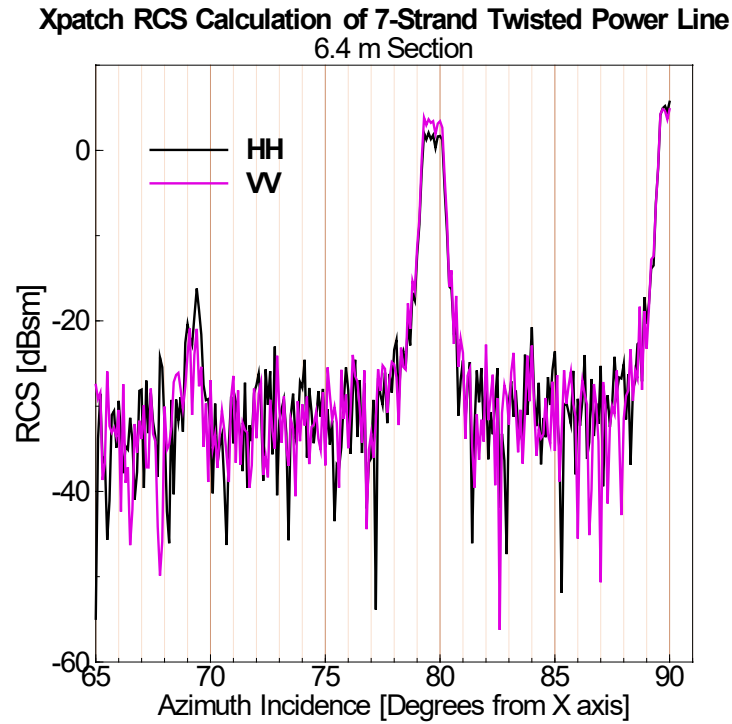
Fig. 11 Xpatch computed RCS of power line for both VV and HH polarizations
