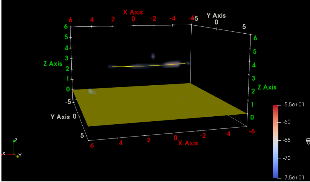
Fig. 28 ParaView VV image of twisted line at 74.6^\circ azimuth-inc, radar view
