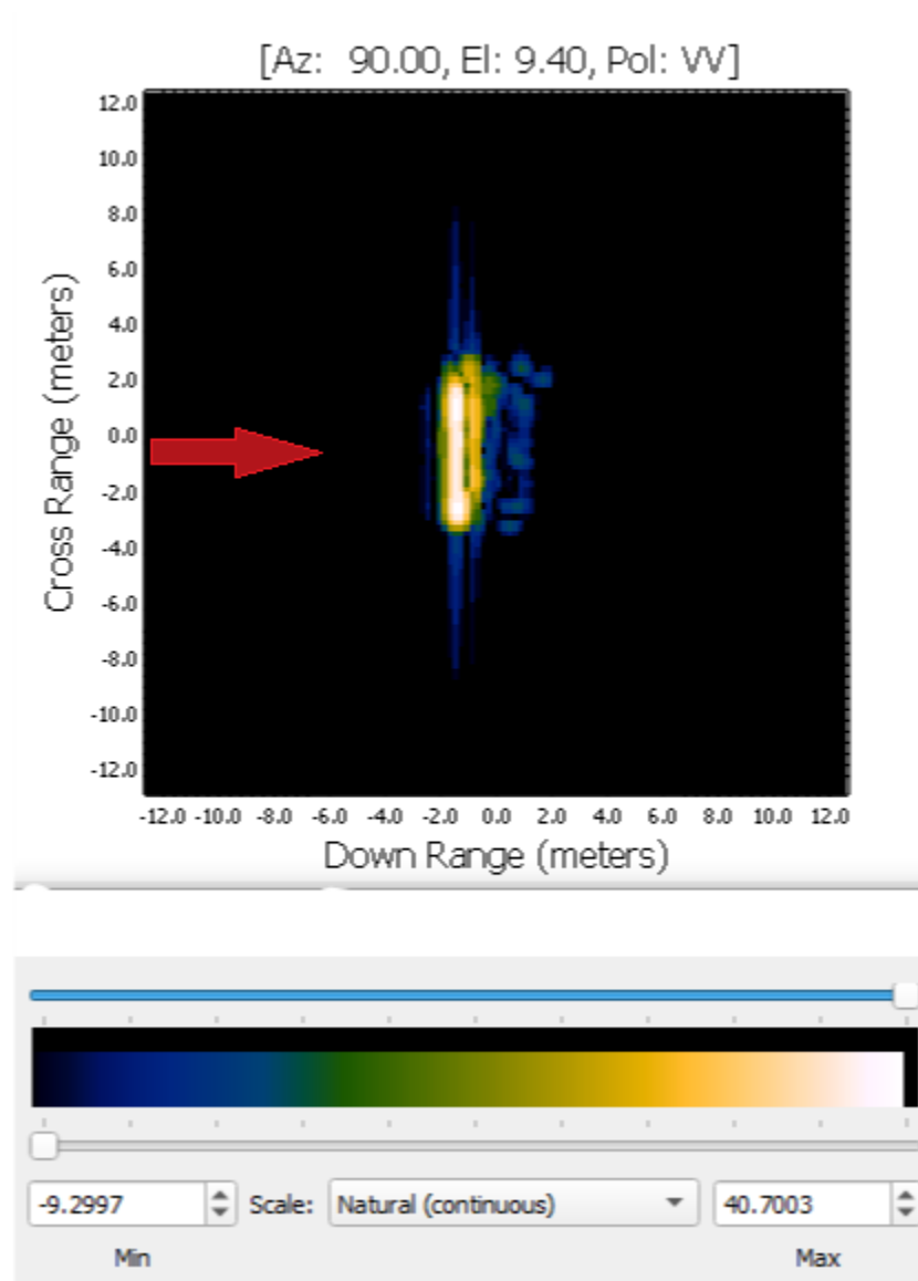
Fig. 31 Catalus VV SAR (dB) broadside-inc against ZSU over flat ground
