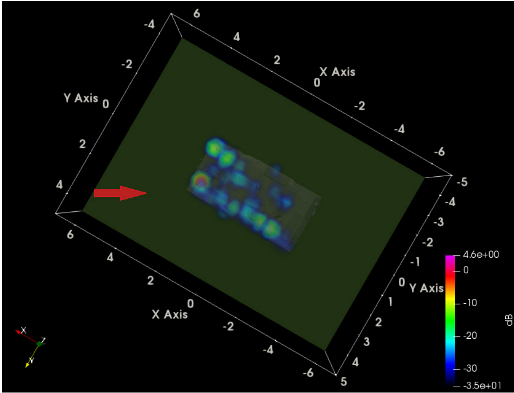
Fig. 44 ParaView VV SAR for 30° azimuth-inc on ZSU over ground, top-down view
