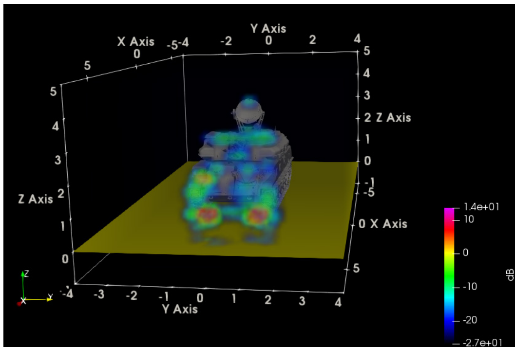
Fig. 49 ParaView HH SAR for 0° azimuth-inc on ZSU, 10° in azimuth from radar view
