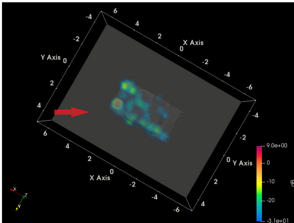
Fig. 43 ParaView HH SAR for 30° azimuth-inc on ZSU over ground, top-down view
