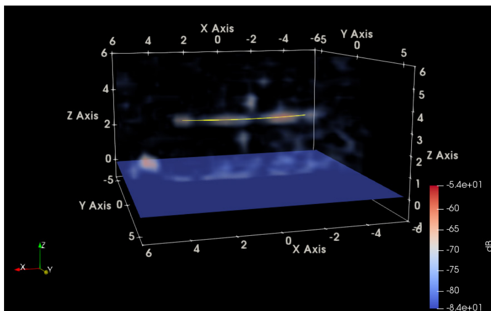
Fig. 27 ParaView HH image of twisted line over ground at with 74.6^\circ azimuth-inc, radar view
