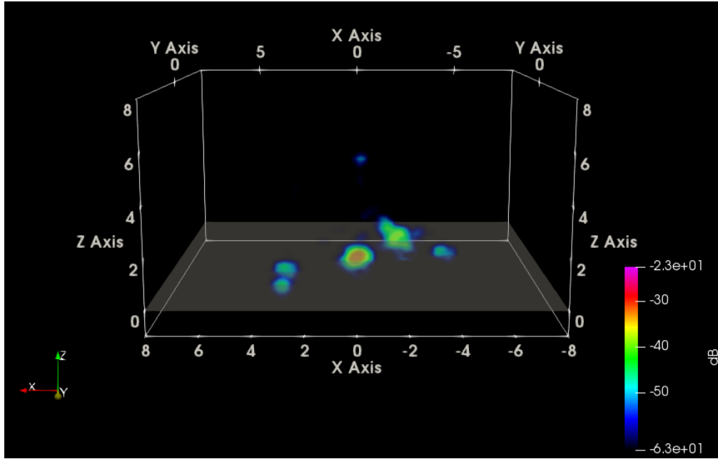
Fig. 61 Radar-view VV SAR of five boulders with rough ground RMS bump height = 3 cm
