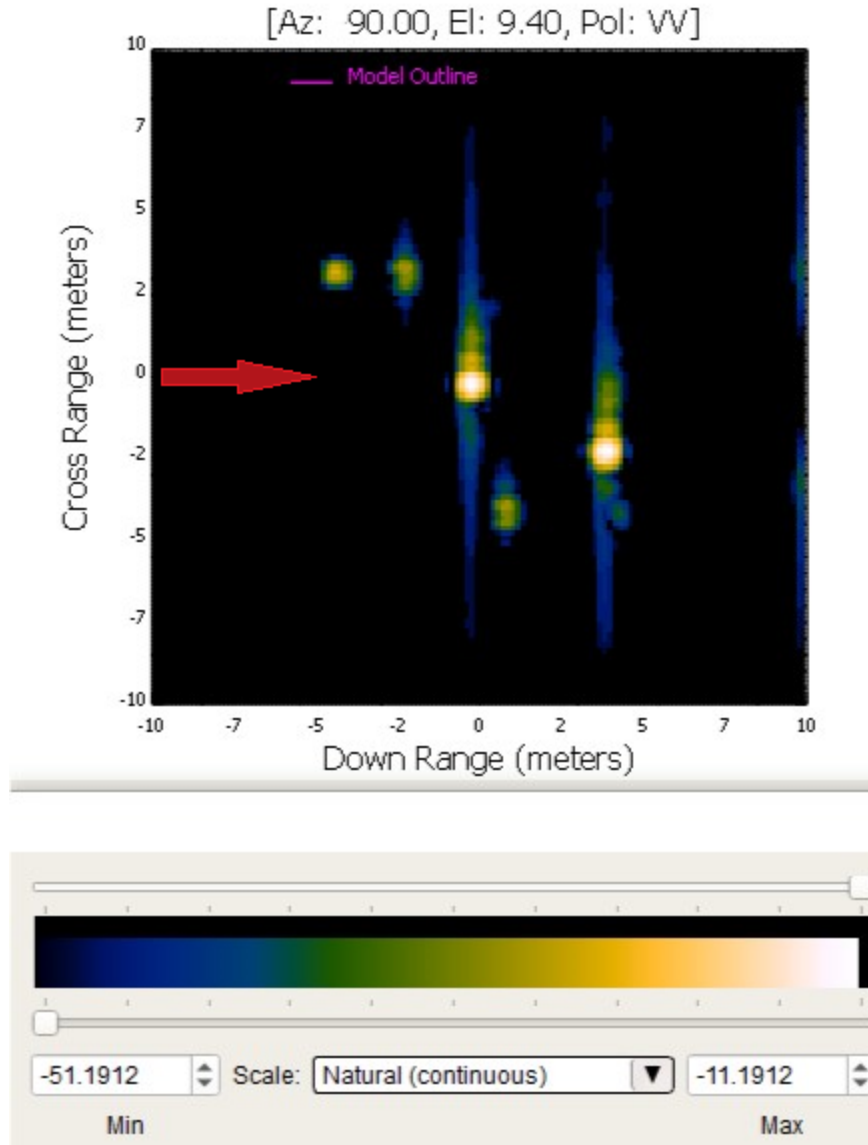
Fig. 56 Catalus VV SAR of boulder field over ground
