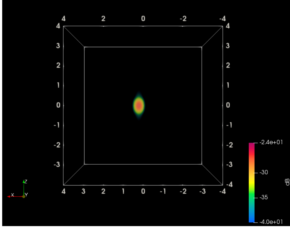
Fig. 9 ParaView (3-D) SAR free-space image of 0.25-m radius PEC sphere
