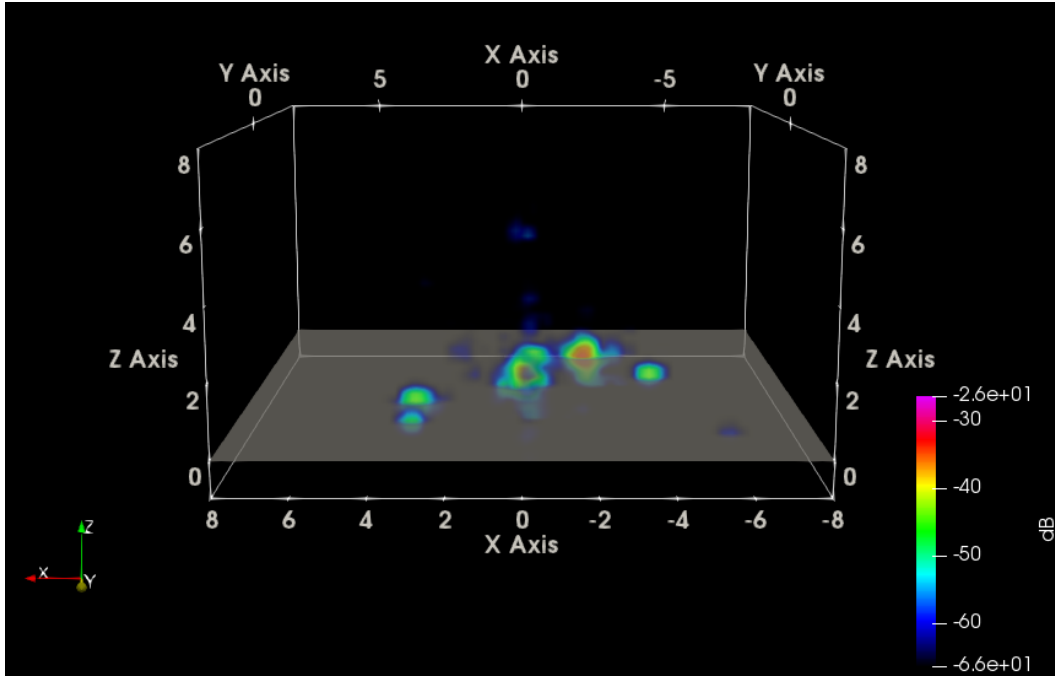
Fig. 63 Radar-view HH SAR of five boulders with rough ground RMS bump height = 15 cm
