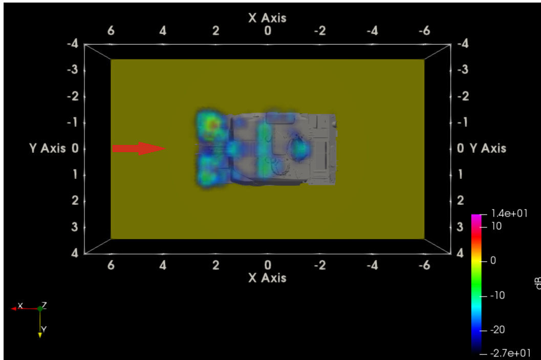
Fig. 50 ParaView HH SAR for 0^\circ incidence on ZSU, top-down view (radar from the right)
