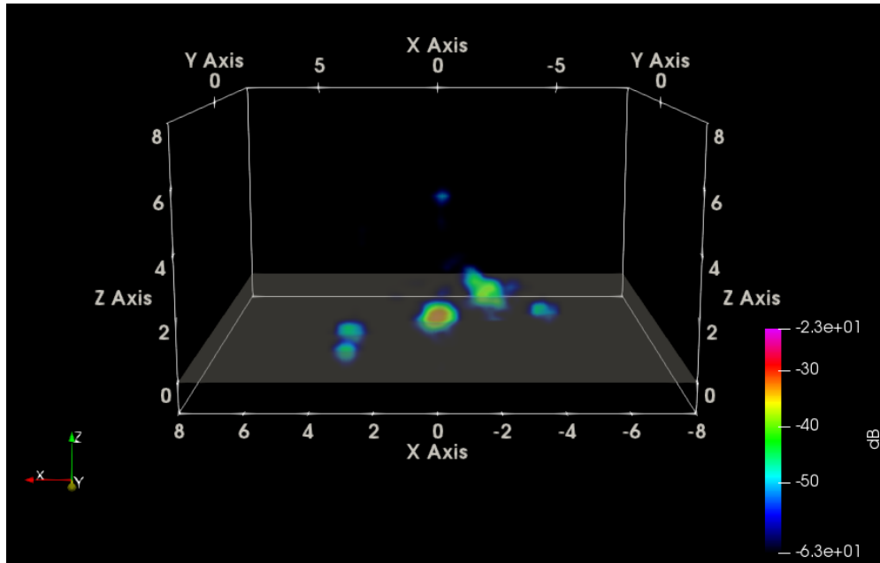
Fig. 59 Radar-view HH SAR of five boulders with rough ground RMS bump height = 6 cm
