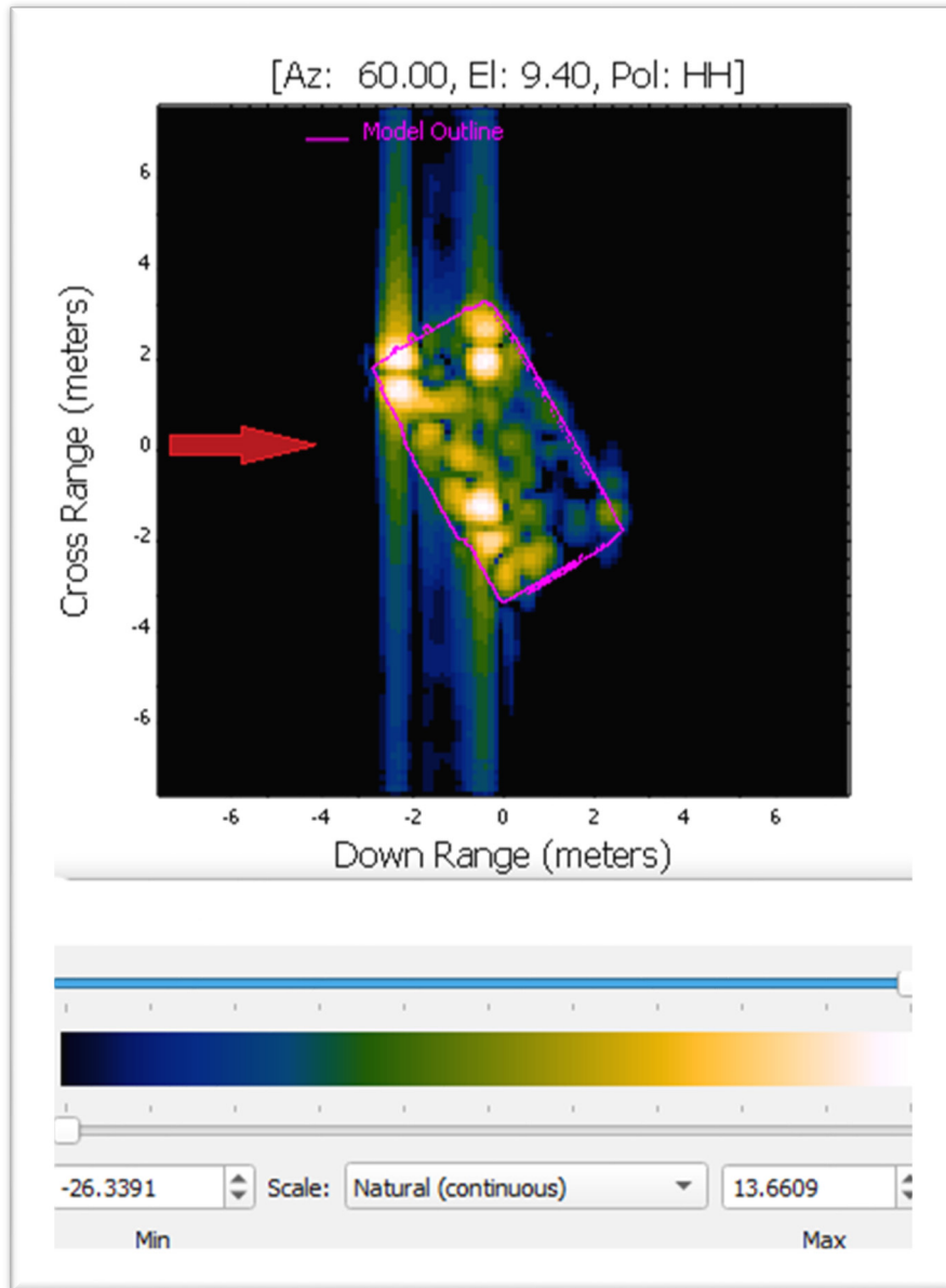
Fig. 37 Catalus HH 60° incidence (dB) on ZSU over flat ground with incidence from the left
