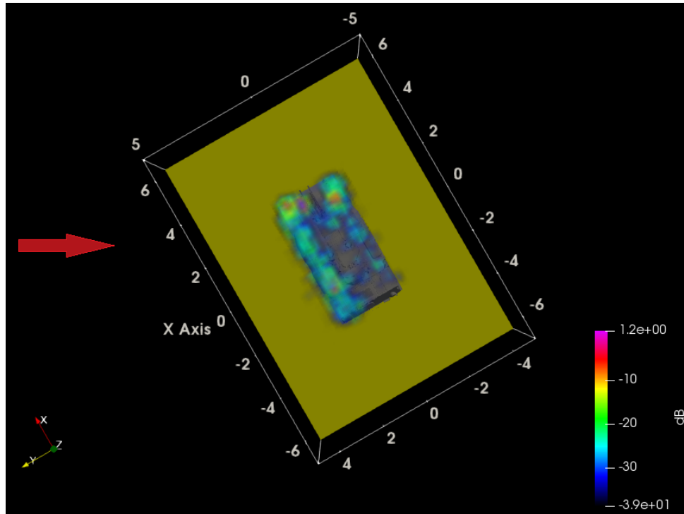
Fig. 38 ParaView HH 60° incidence on ZSU over flat ground, top-down view with incidence from the left
