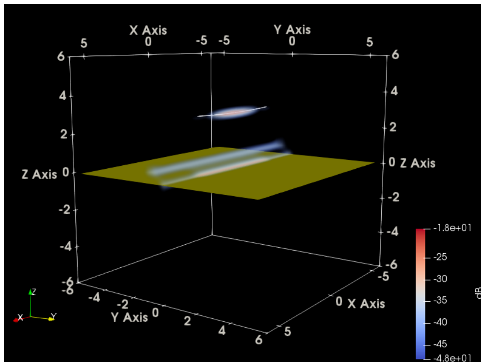
Fig. 15 ParaView 89.6° azimuth-inc HH image from twisted line in side perspective
