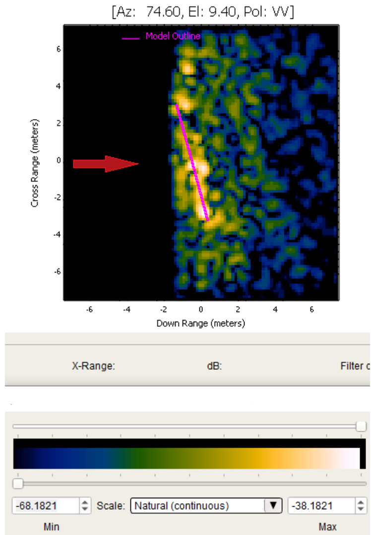
Fig. 25 Catalus VV SAR (dB) of twisted line over ground at 74.6° azimuth-inc
