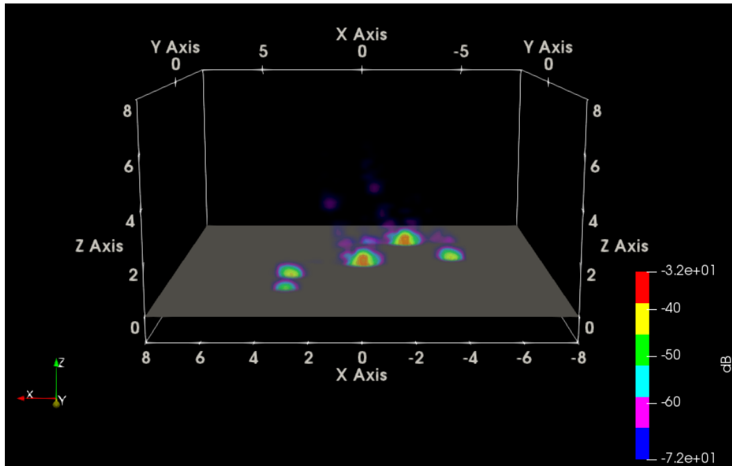
Fig. 53 ParaView VV SAR of boulder field, radar view
