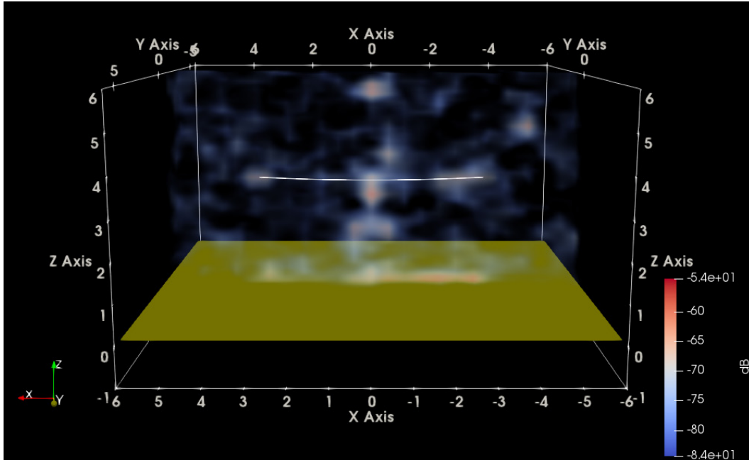
Fig. 19 ParaView radar-view HH image of twisted line at 84.6° azimuth with wire and ground plane overlaid
