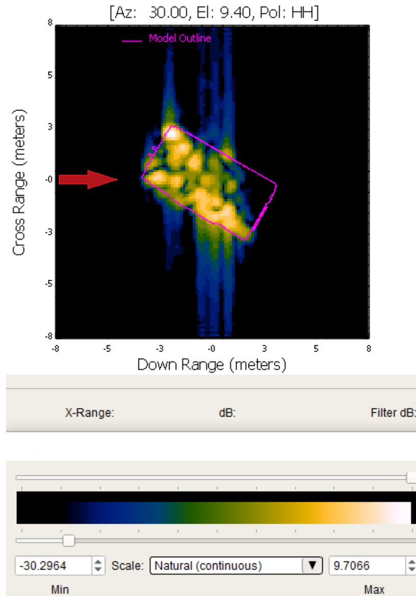
Fig. 40 Catalus HH SAR image of free-space ZSU; azimuth-inc at 30° (radar from the left)
