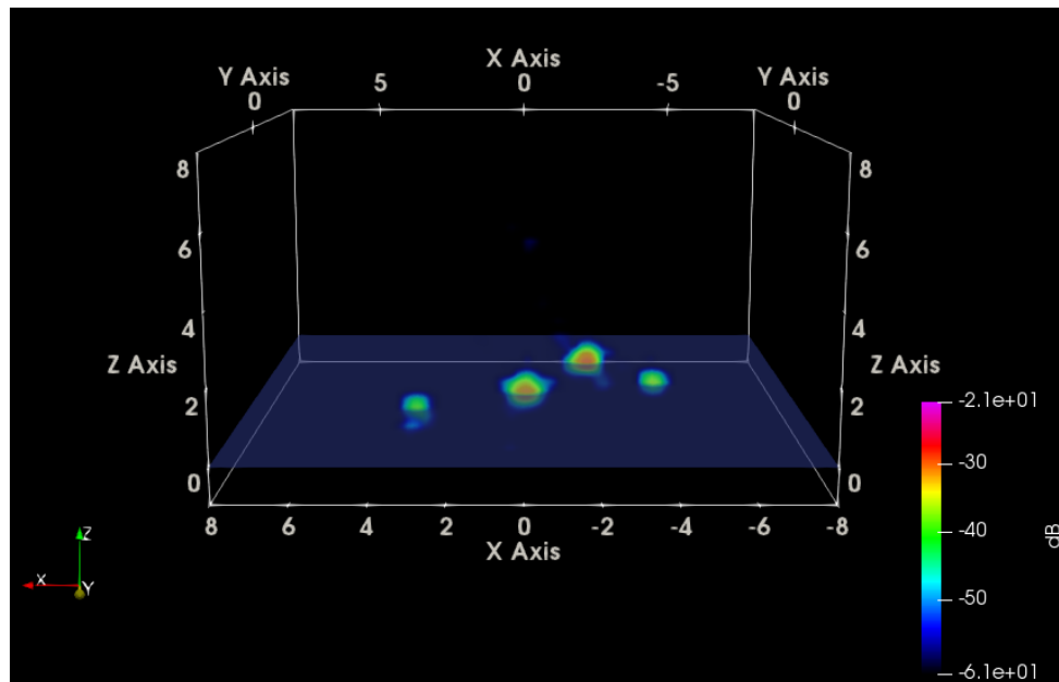
Fig. 58 Radar-view HH SAR of five boulders with rough ground RMS bump height = 3 cm
