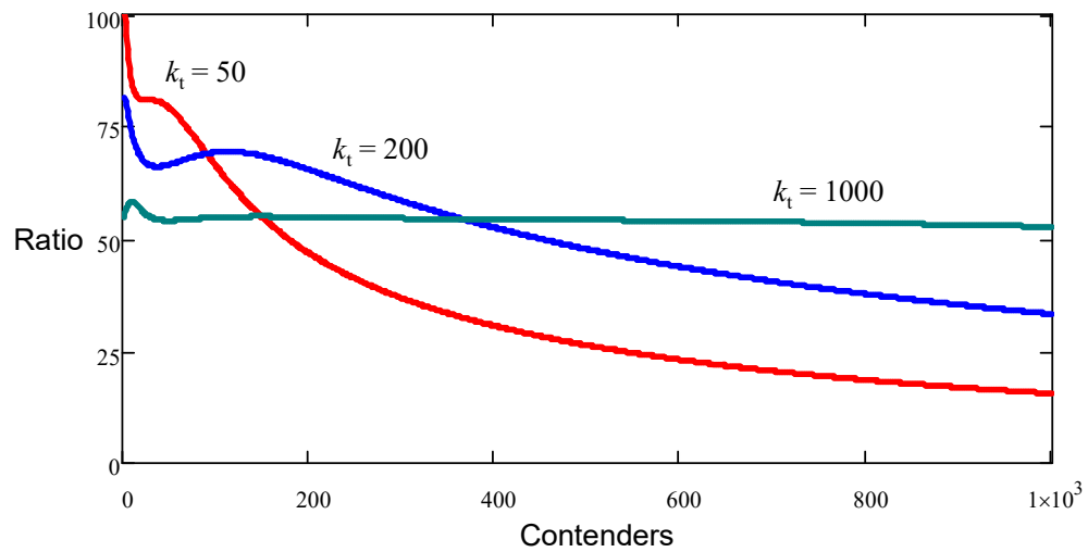
Figure 3-15. Contention Collision Resolution Success Ratio of the Eight-Contention-Phase CRS Design
