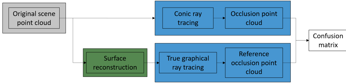
Figure 3.9: The process for evaluating the performance of the conic ray tracing method by using the reference point cloud to compute the confusion matrix.
