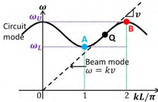
Figure 15: The lower band edge (A), the upper band edge (B), and the operating point (Q) at which the beam mode intersects with the circuit mode in a coupled cavity TW. kL is the phase shift per period [13].
