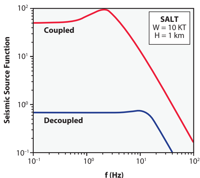
Figure 5. Seismic Cavity Decoupling Strength as a Function of Frequency
