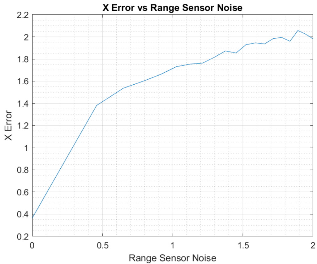
Figure 19: Plot comparing range sensor noise to X-error. The noise has a noticeable impact on error and should be kept as low as possible for best performance.
