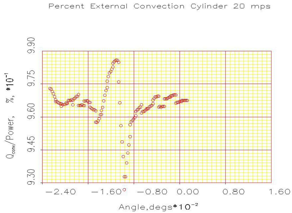
Figure 5-7. Percent External Convection Heat Transfer Rate 20 m/s
