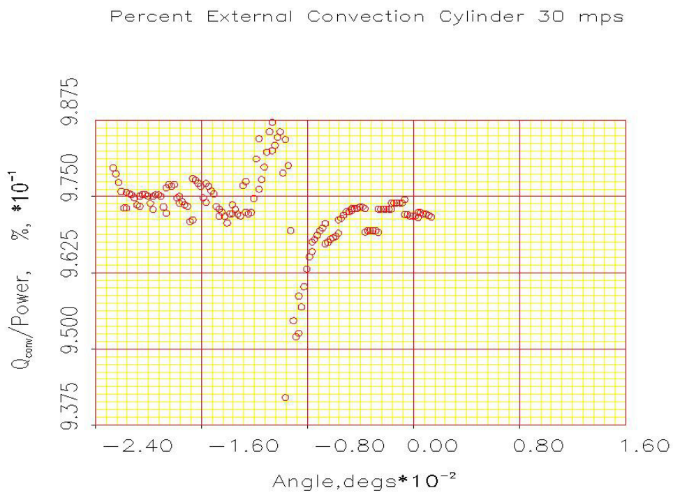
Figure 5-8. Percent External Convection Heat Transfer Rate 30 m/s
