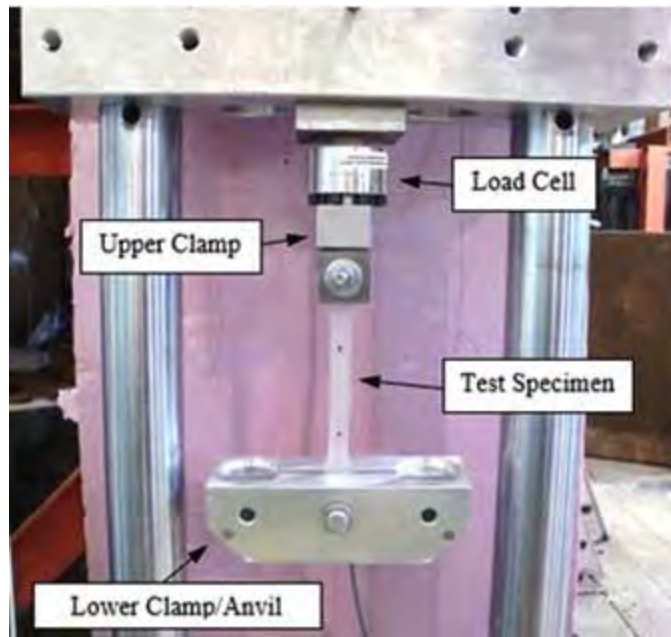
Figure 19: Load cell connection.
