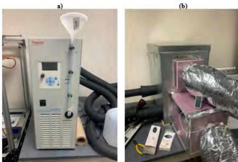
Figure 53: Temperature control: (a) air conditioner (b) air ventilator.
