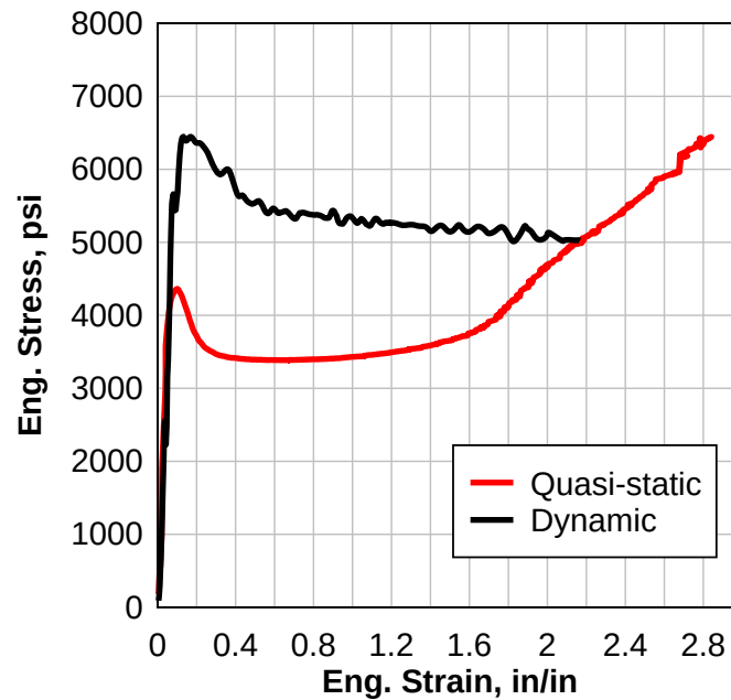
Figure 51: Dynamic and quasi-static engineering stress-strain response of SG.
