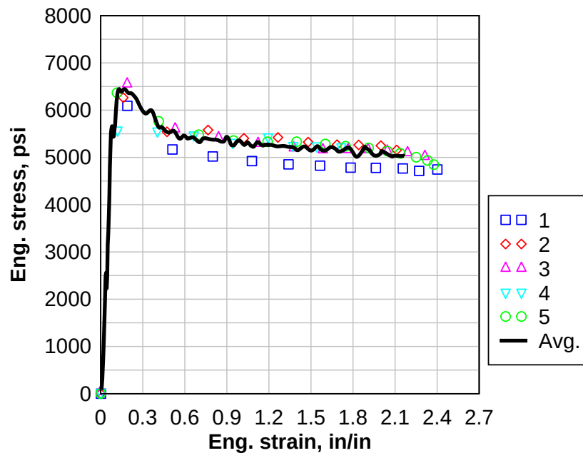
Figure 41: Engineering stress versus engineering strain of SG drop weight test specimens.
