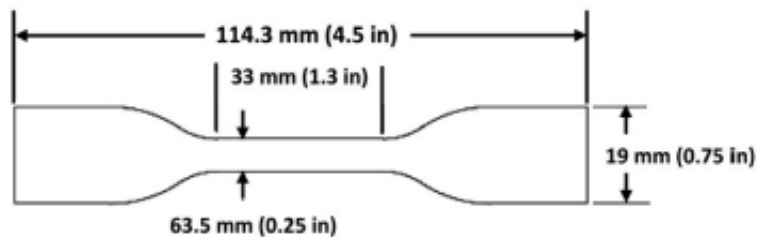
Figure 10: Quasi-static specimen geometry.
