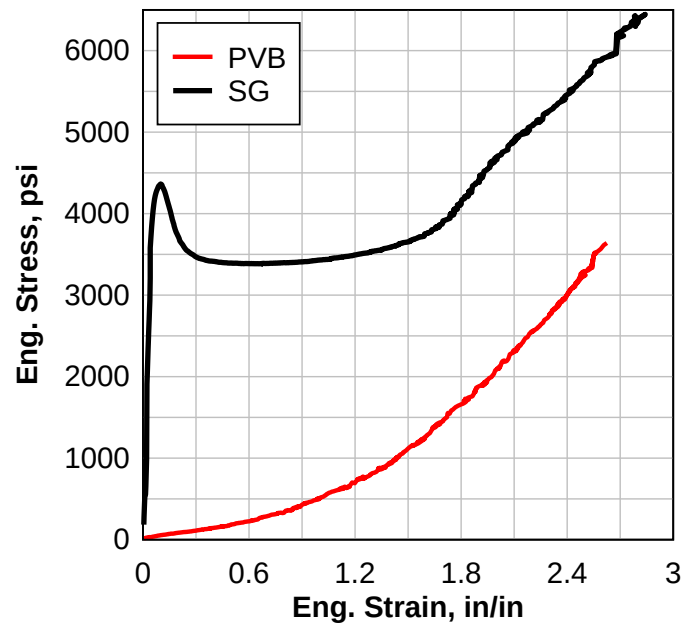
Figure 49: Engineering stress versus engineering strain for PVB and SG under quasi-static loading.
