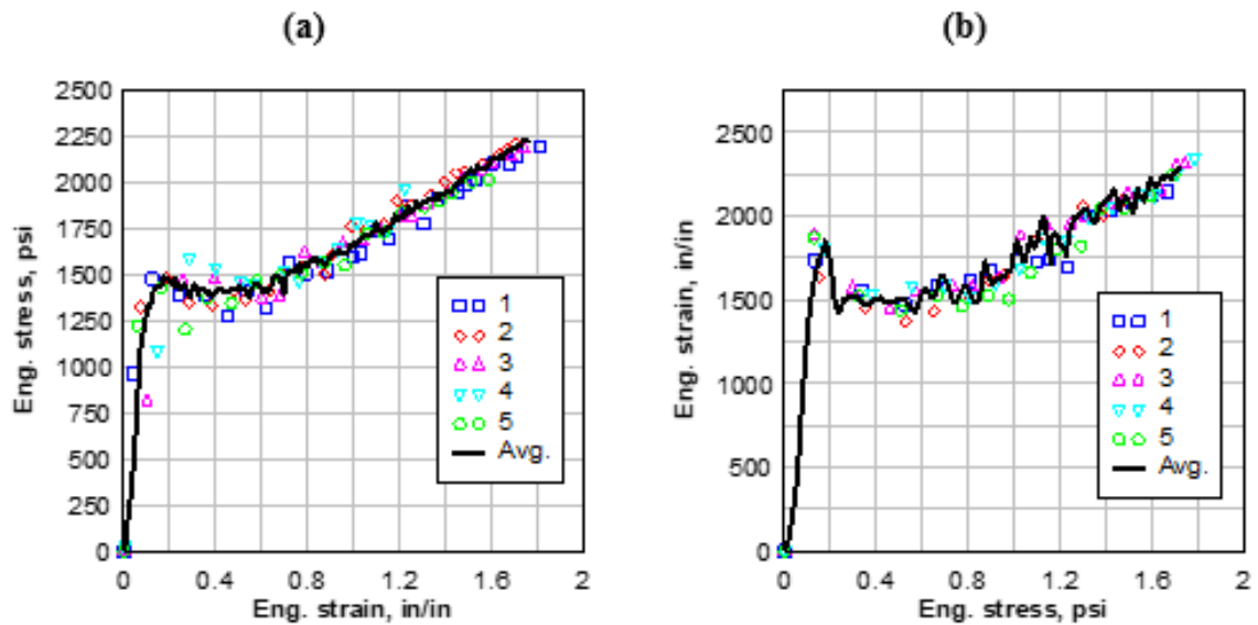
Figure 32: Engineering stress versus engineering strain for cold temperature drop weight tests (a) H=19in. (b) H=43 in.
