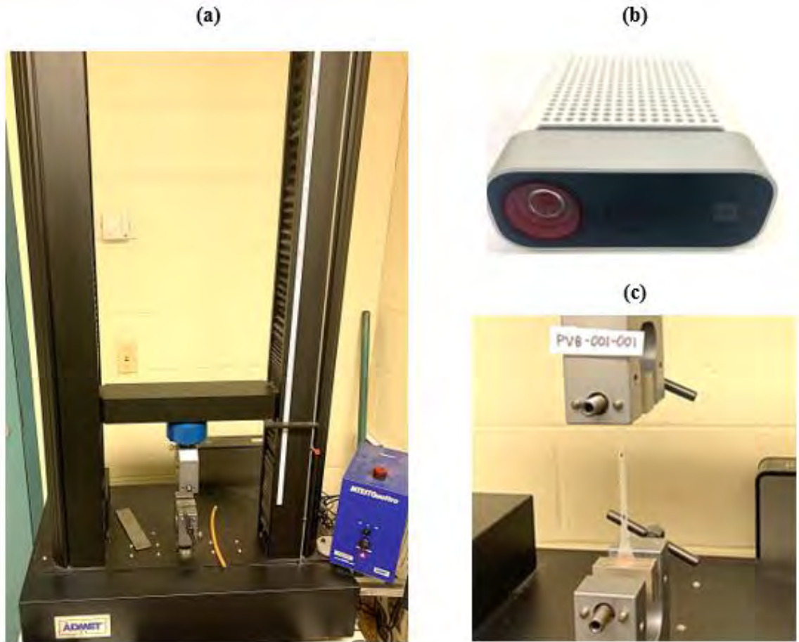
Figure 24: Quasi-static test setup: (a) test machine, (b) camera, (c) quasi-static testing of PVB specimen.
