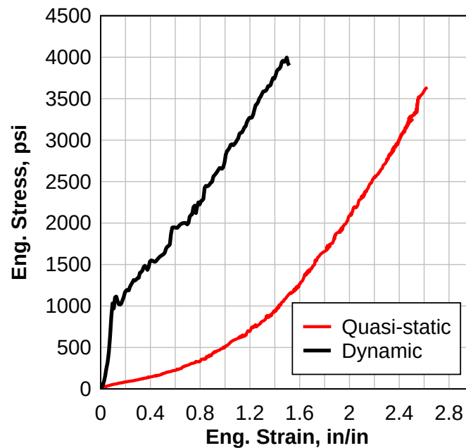
Figure 50: Dynamic and quasi-static engineering stress-strain response of PVB.
