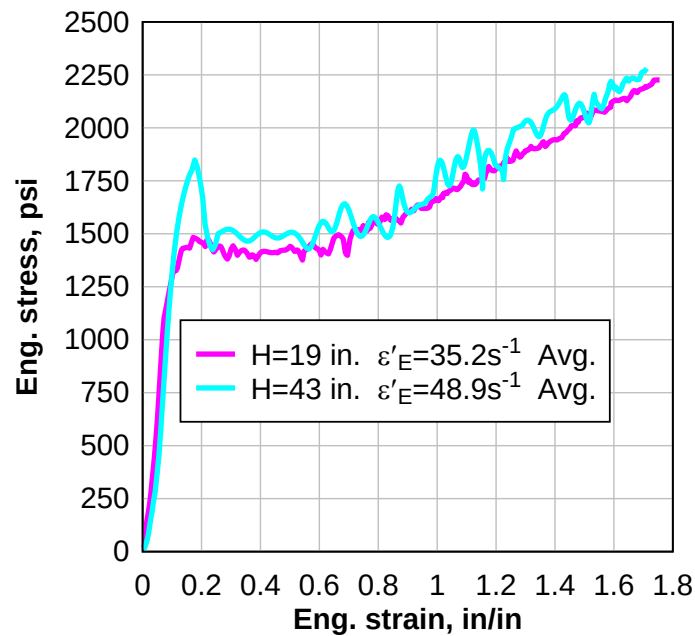
Figure 33: Engineering stress versus engineering strain of cold temperature drop weight tests.
