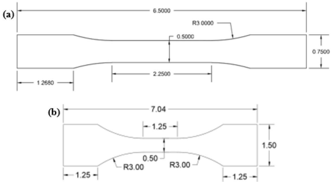
Figure 6: (a) Unmodified and (b) modified (N.T.S) ASTM Type I specimen geometry.
