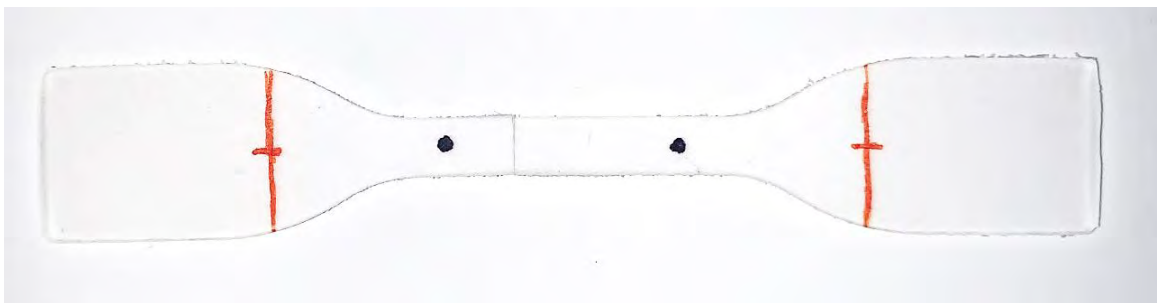
Figure 45: Failed unaged PVB quasi-static test specimen.
