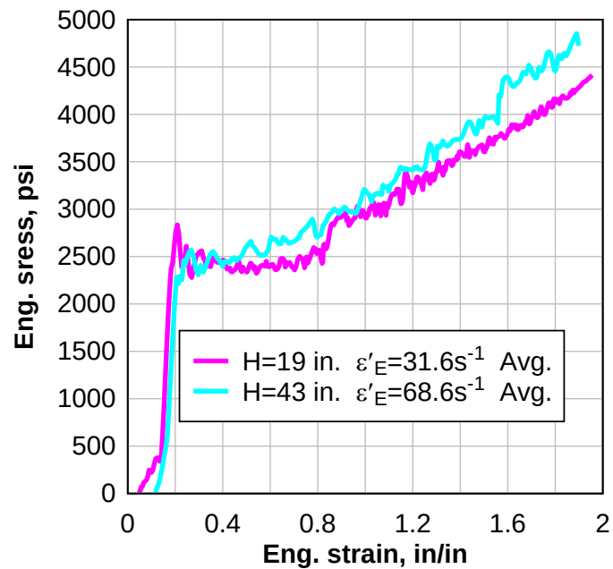
Figure 35: Engineering stress versus engineering strain of moderate temperature drop weight tests.
