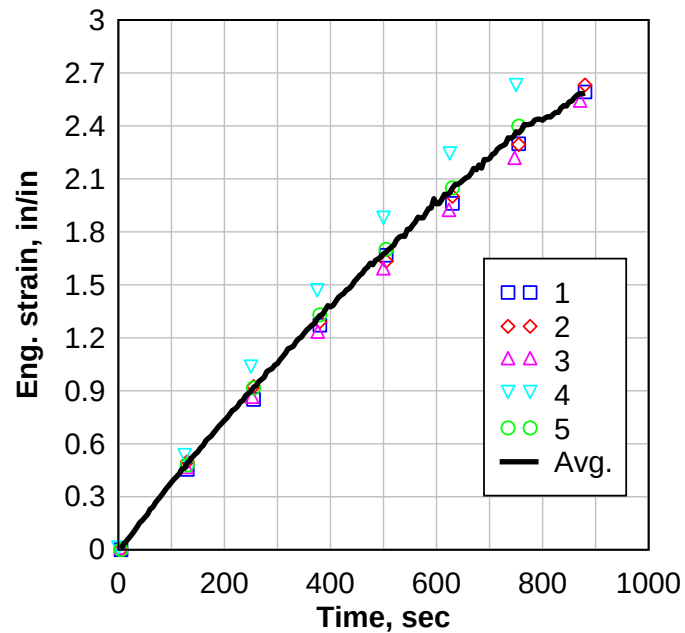
Figure 43: Engineering strain time histories of unaged PVB specimens under quasi-static loading.
