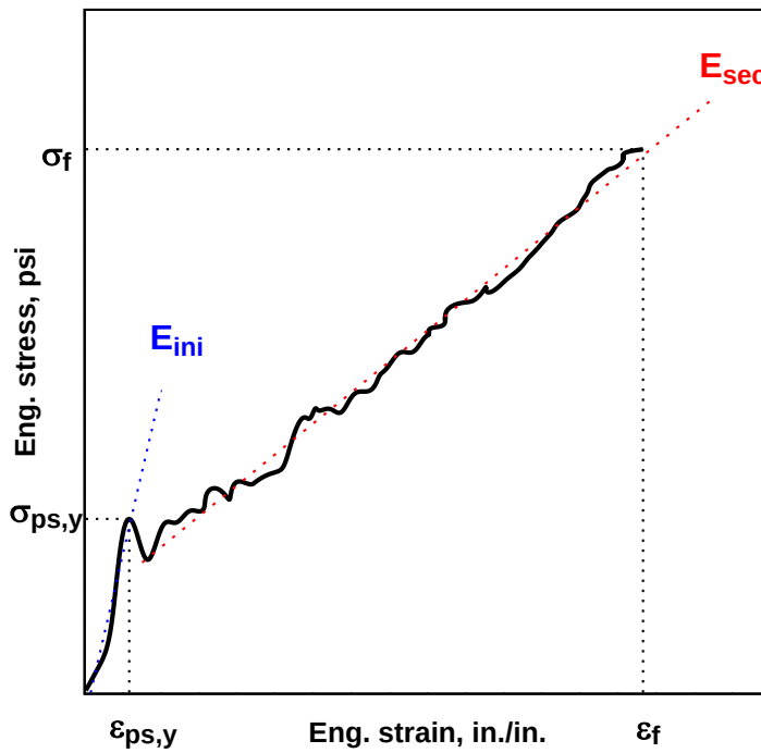
Figure 28: Typical aged PVB engineering stress versus engineering strain data analysis
