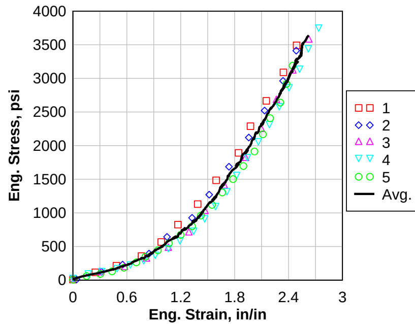
Figure 44: Engineering stress versus engineering strain of unaged PVB specimens under quasi-static loading.
