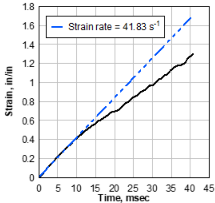
Figure 25: Typical engineering strain versus time curve for PVB drop weight specimen.
