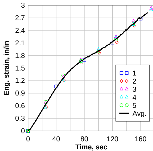
Figure 46: Engineering strain time histories of SG specimens under quasi-static loading.
