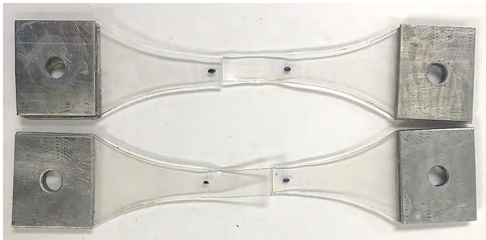
Figure 42: Failed SG drop weight test specimens.
