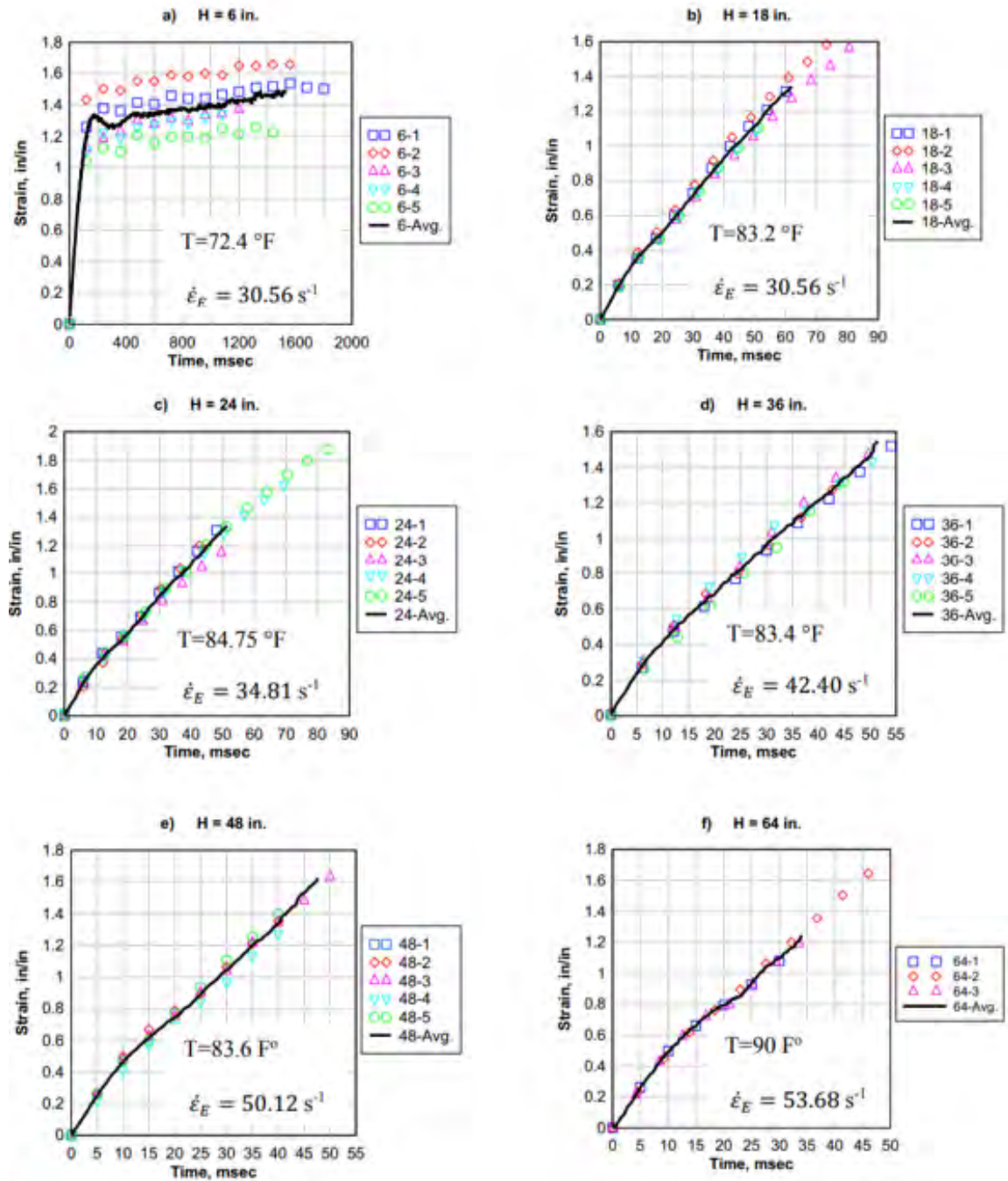
Figure 26: Engineering strain-time histories of aged PVB.
