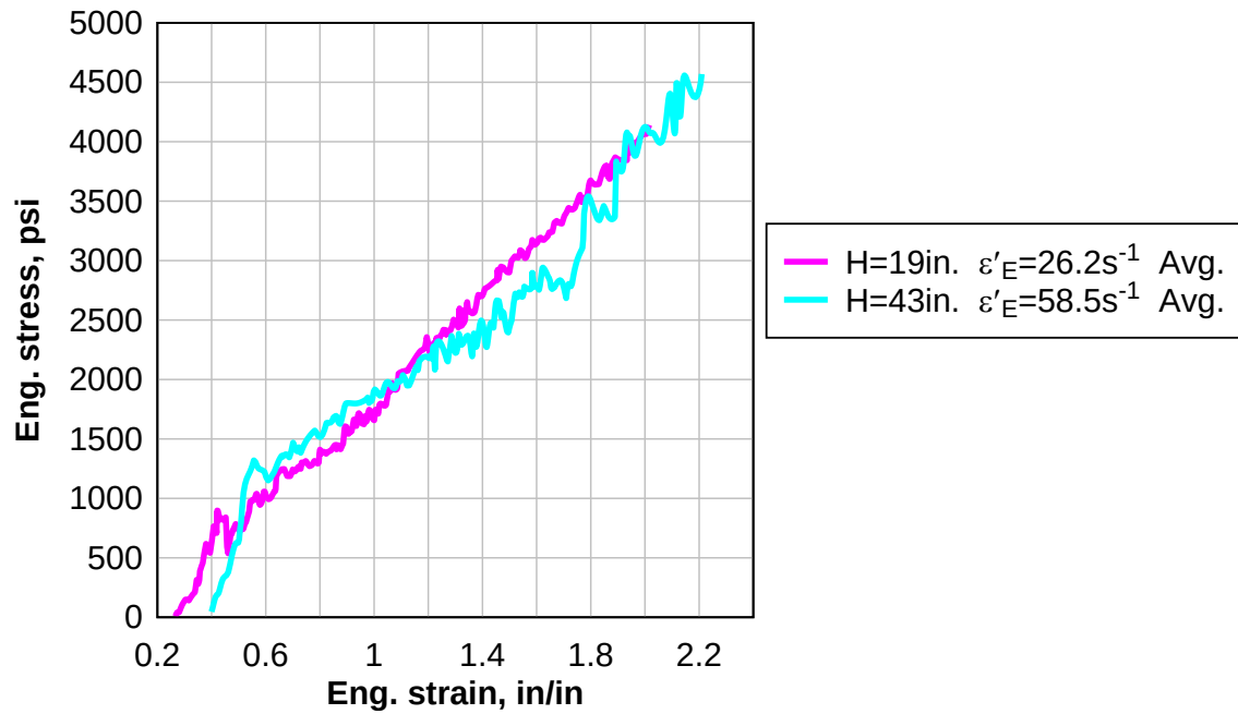
Figure 37: Engineering stress versus engineering strain of hot temperature drop weight tests
