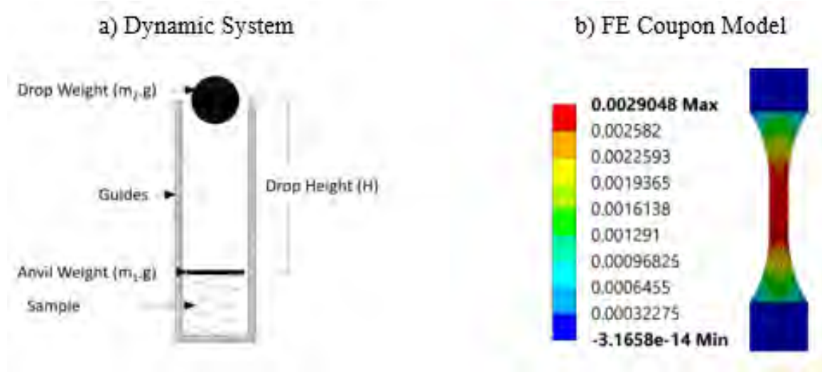
Figure 23: Dynamic system model of drop weight machine.
