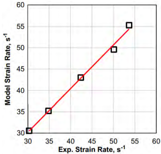
Figure 27: Comparison between experimental and analytical strain rates
