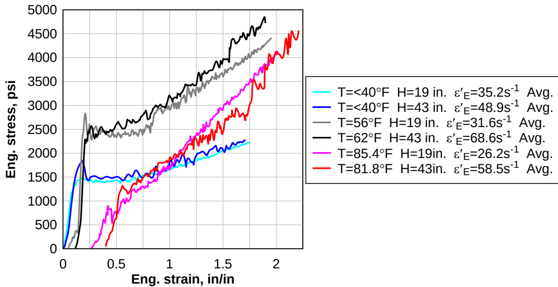
Figure 38: Engineering stress versus engineering strain for unaged PVB specimens tested at two different strain rates and three different temperature ranges.
