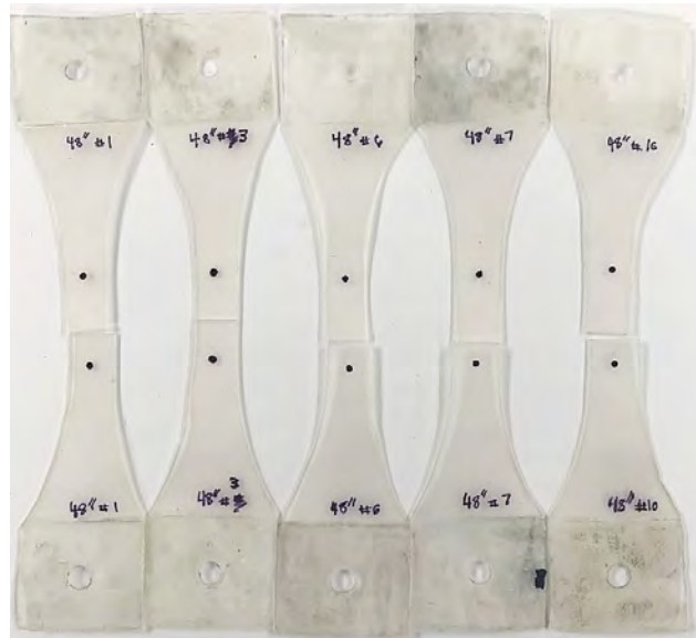
Figure 30: Failed aged PVB drop weight specimens (H = 48 in.).
