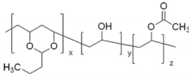
Figure 2: PVB chain structure (Martín et al., 2020).
