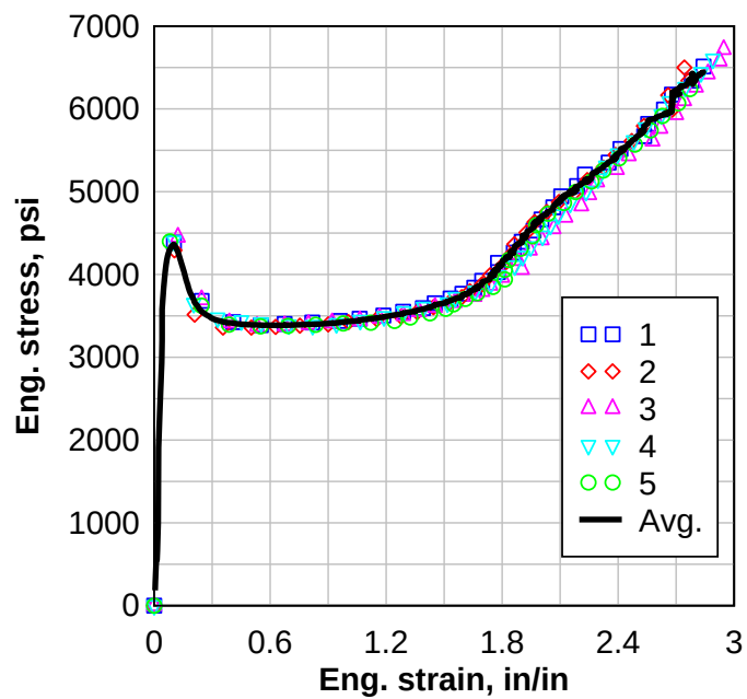
Figure 47: Engineering stress versus engineering strain of SG specimens under quasi-static loading.
