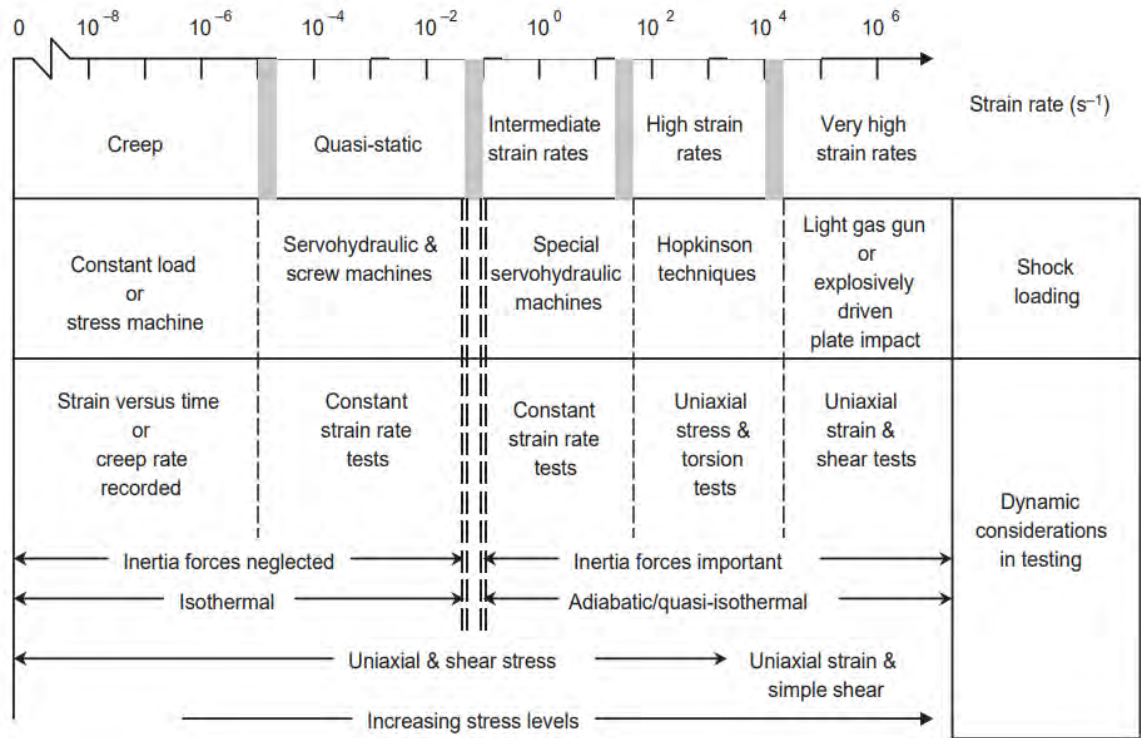
Figure 4: Strain rate regimes and associated instruments and experimental conditions (Nemat-Nasser, 2000).
