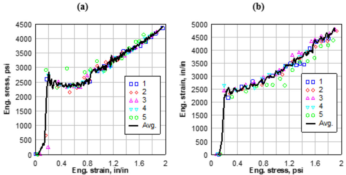
Figure 34: Engineering stress versus engineering strain for moderate temperature drop weight tests (a) H=19in. (b) H = 43 in.
