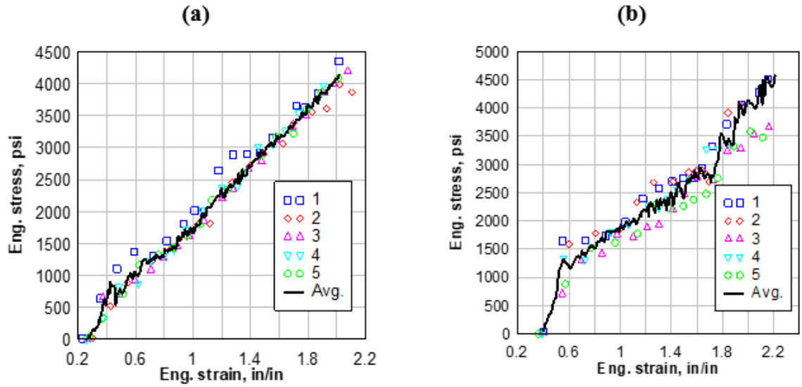
Figure 36: Engineering stress versus engineering strain of moderate temperature drop weight tests.
