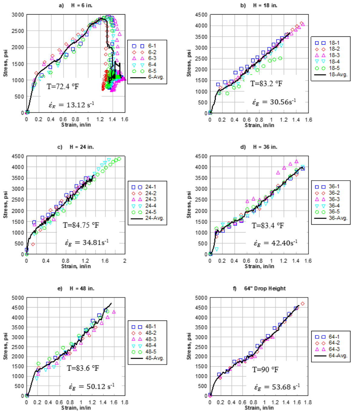
Figure 29: Engineering stress vs. engineering strain of PVB at various strain rates.
