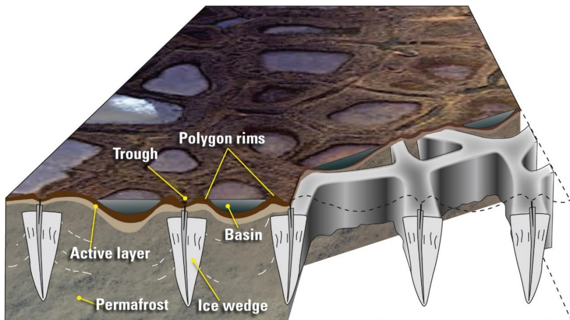
Figure 5. The Surface Expression of Ice Wedges (Martin et al., 2009)
