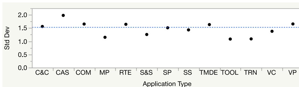
Figure 7: LN Productivity (AAF) by Application Type Variance Distribution
