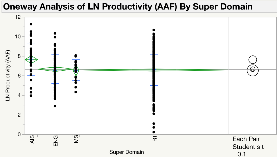
Figure B-4: One-Way ANOVA of LN Productivity (AAF) by Super Domain
