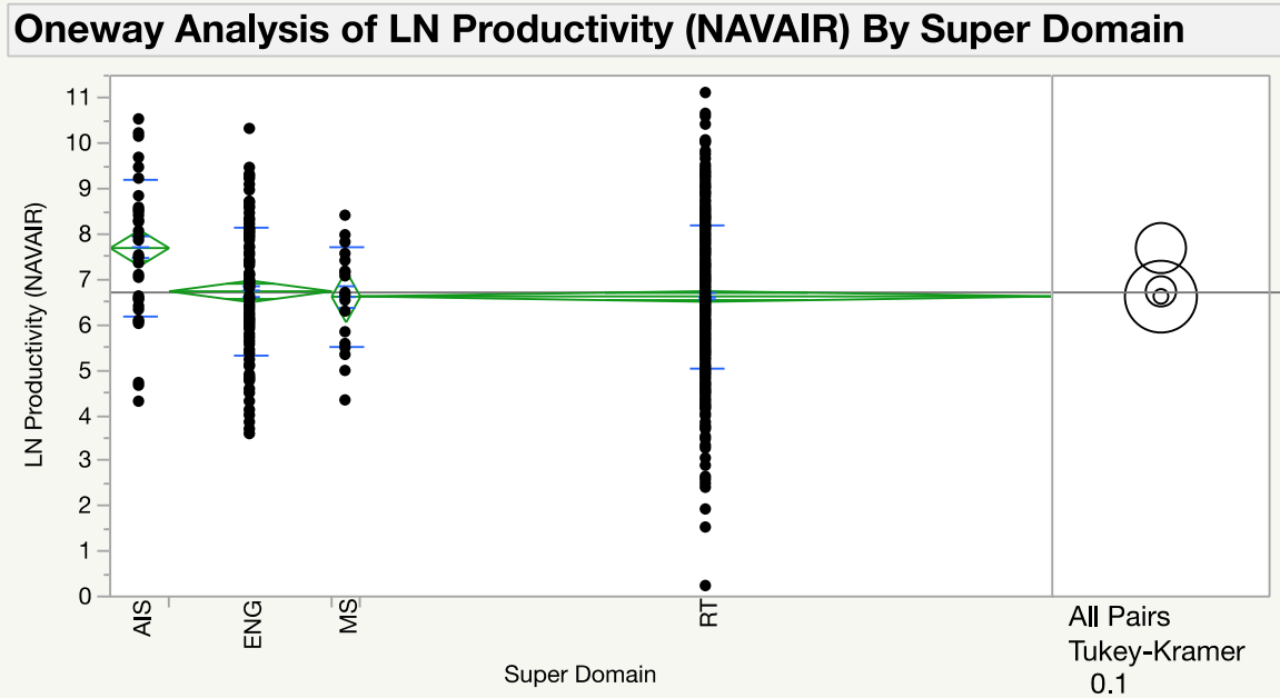
Figure B-3: One-Way ANOVA of LN Productivity (NAVAIR) by Super Domain
