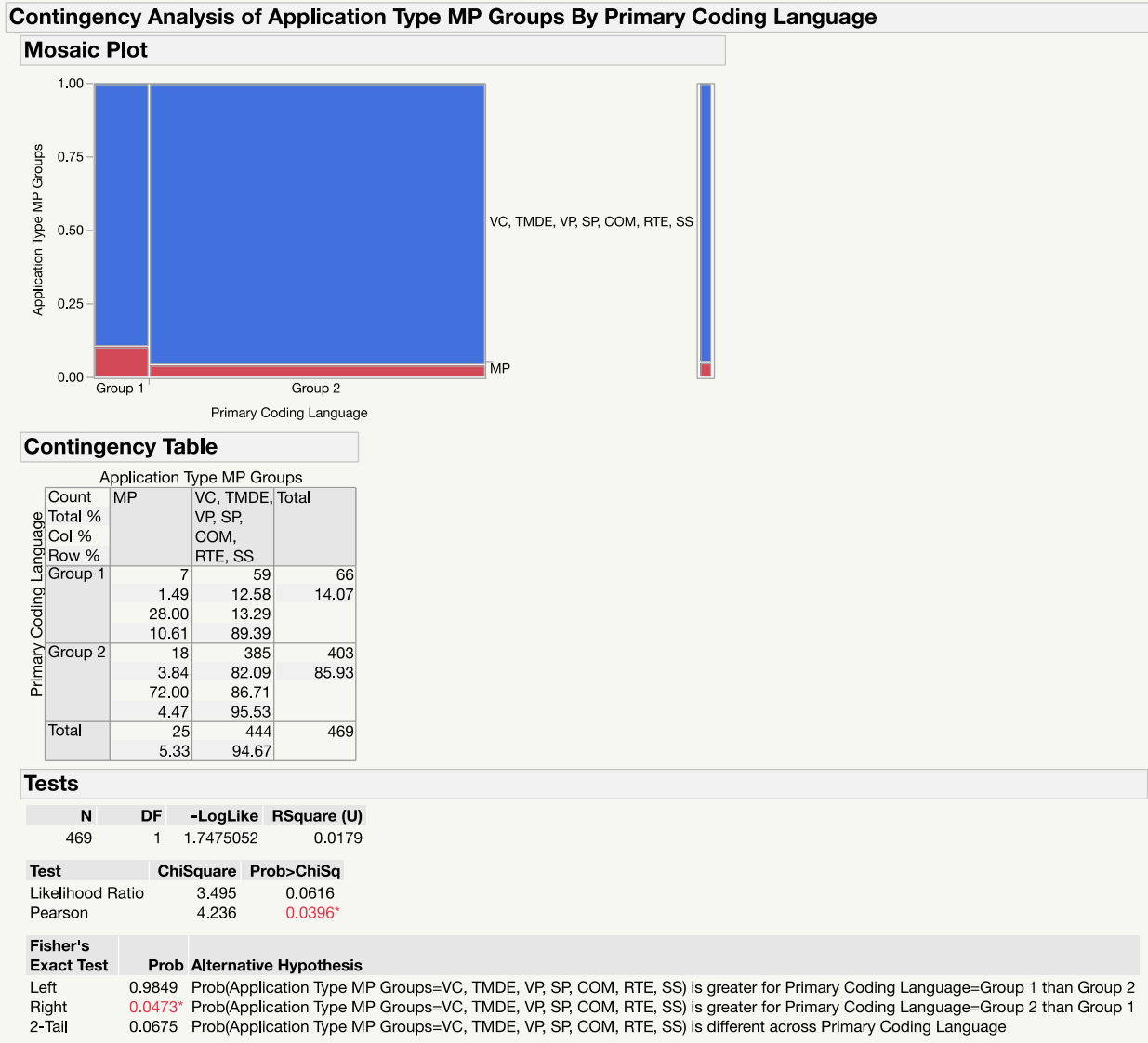
Figure C-1: Contingency Analysis of Application Type MP Groups by Primary Coding Language Conversion Factor
