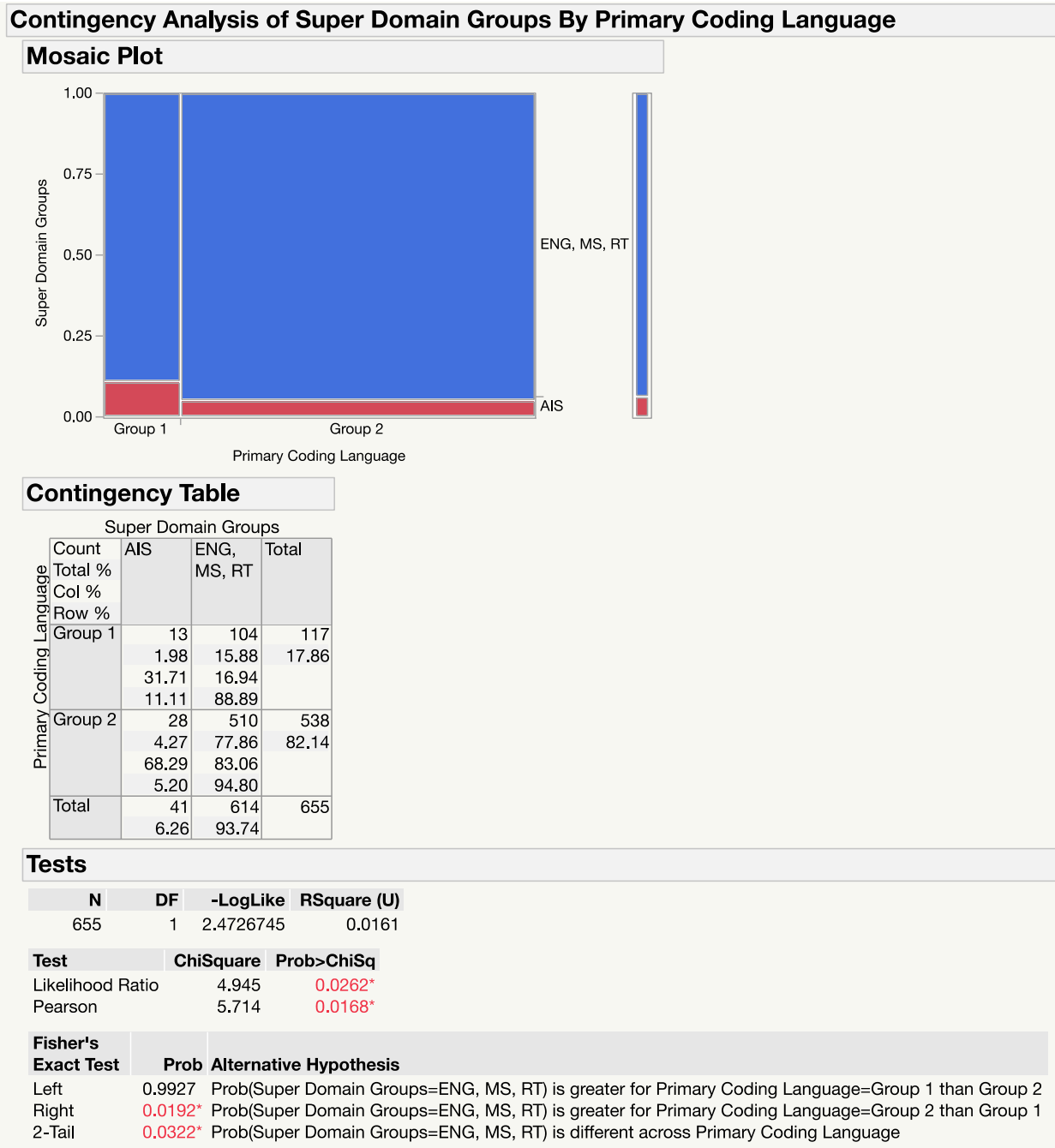
Figure C-11: Contingency Analysis of Super Domain AIS Groups by Primary Coding Language Conversion Factor
