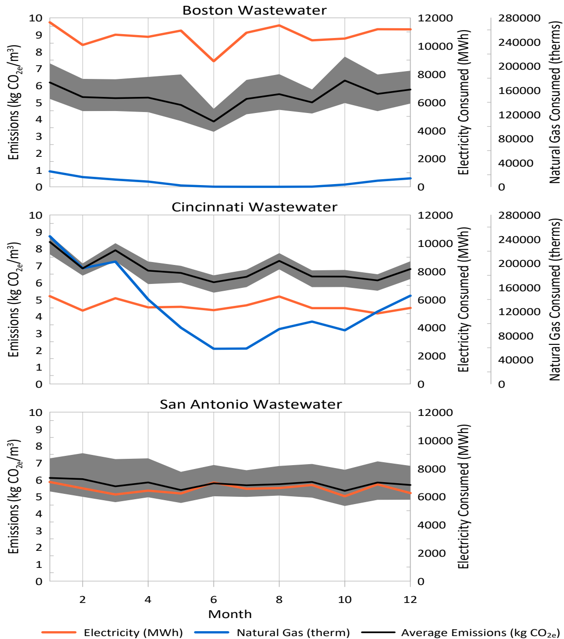
Figure 7. Sample cities showing intra-annual fluctuations in emissions attributed to electricity and natural gas consumed per m^3 of treated wastewater.
