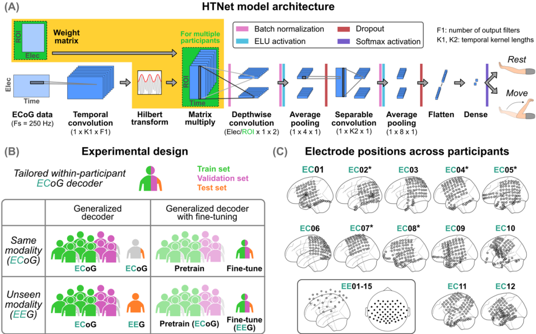
Figure 2: Overview of HTNet architecture, experimental design, and electrode locations. (A) HTNet is a convolutional neural network architecture that extends EEGNet by handling cross-participant variations in electrode placement and frequency content. (B) Using electrocorticography data, both tailored within-participant and generalized multi-participant models were trained to decode arm movement vs. rest. Multi-participant decoders were tested separately on held-out data from unseen participants recorded with either the same modality as the train set (ECoG) or an unseen modality (EEG). These pre-trained decoders were fine-tuned using data from the test participant. (C) Electrode placement varies widely among the 12 ECoG participants. Asterisks denote five participants whose electrodes were mirrored from the right hemisphere.
