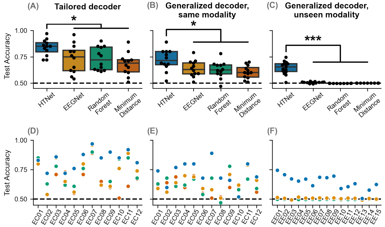
Figure 4: HTNet generalizes better than EEGNet and other decoders. HTNet achieves significantly higher test accuracy than EEGNet, random forest, and minimum distance decoders across all three scenarios: (A) tailored ( p < 0.05 ), (B) same modality ( p < 0.05 ), and (C) unseen modality ( p \leq 0.001 ). Note that the trained models for same and unseen modality conditions are identical; only the test set differs. (D–F) Bottom row displays decoder performance grouped by test participant for each fold.
