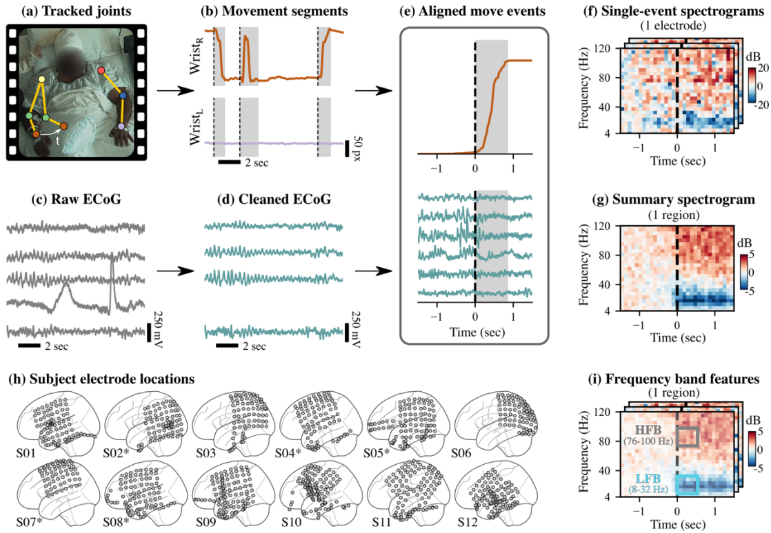
Figure 1: Schematic overview of data processing, analysis, and modeling framework. (a)–(b) Based on continuous video monitoring of each subject, trajectories of the left and right wrists (Wrist L and Wrist R in (b)) were estimated using neural networks and automatically segmented into move (gray) and rest (white) states as shown in (b). (c)–(d) Raw multi-electrode electrocorticography (ECoG) was filtered and re-referenced; bad electrodes (e.g., ones with artifacts) were removed from further analysis. (e) Movement onset events detected from video as shown in (b) were aligned with ECoG data using timestamps. (f) For each move event at each electrode, spectral power was computed and visualized as a log-scaled spectrogram. (g) Summarizing across events and electrodes, the spectral power was projected from electrodes onto 8 cortical regions based on anatomical registration and computed the median power across movement events. (h) The data included 12 subjects; their electrode placements are shown in MNI coordinates. Five of the subjects had electrodes implanted in their right hemispheres (denoted by asterisks). For consistency of later analyses, these electrode locations were mirrored as shown. (i) To partially explain the event-by-event neural variability in low-frequency (LFB: 8–32 Hz) and high-frequency (HFB: 76–100 Hz) spectral power, multiple linear regression models were fit at each electrode using behavioral features extracted from the videos.
