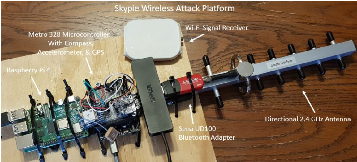
Figure 11: skypie v3 Prototype Hardware Components
