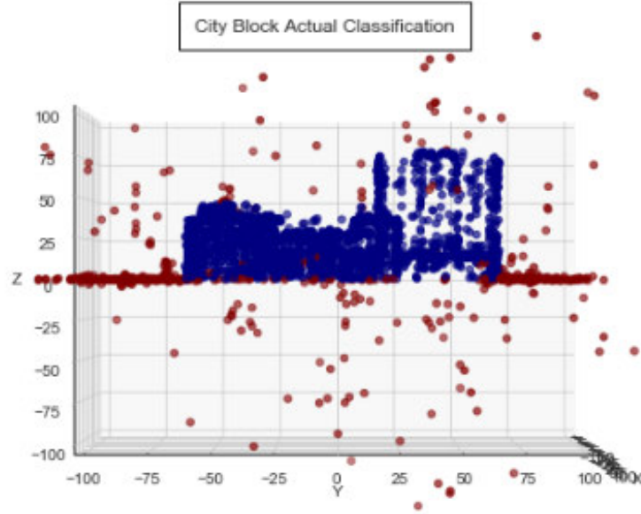
Figure 39: Outliers in Generated Point Cloud - City Block
