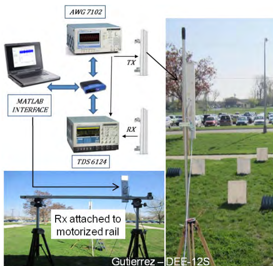
AFIT's RAIL experimental radar system transmits digital communication waveforms, while a receiver independently collects data. New signal processing techniques reduce image background clutter for improved target detection.
