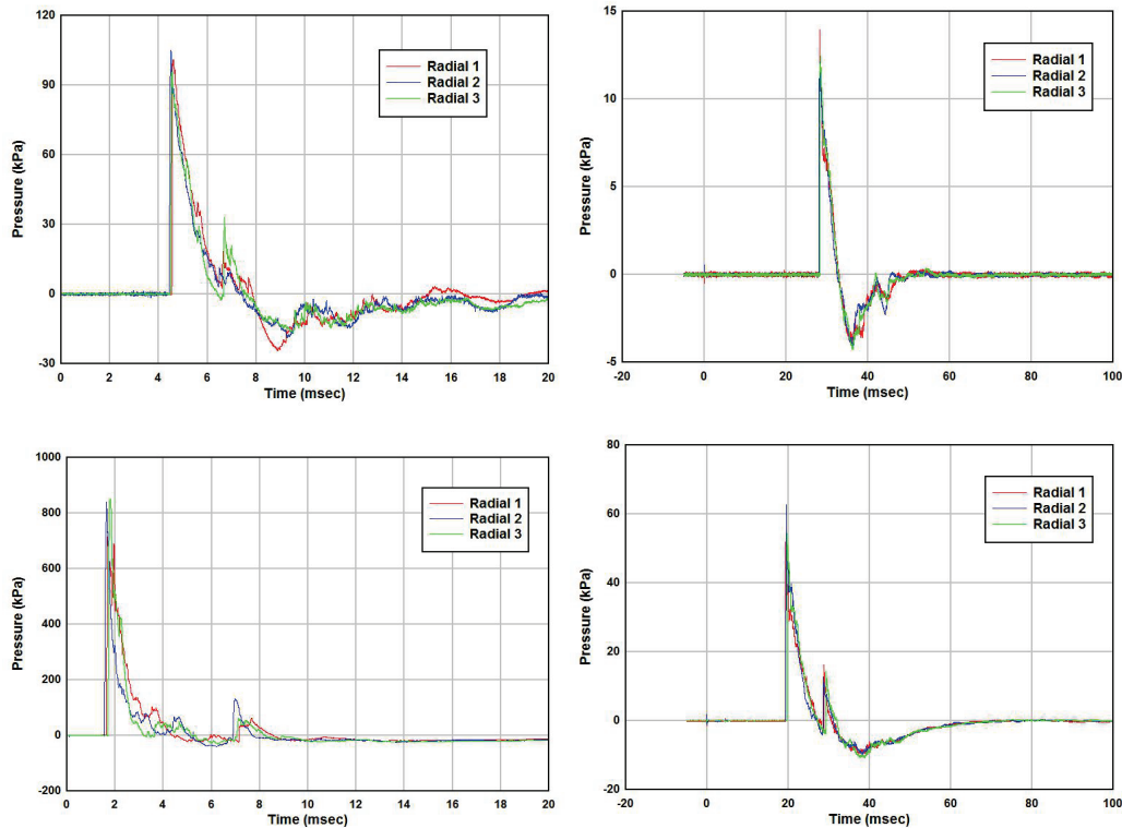
Figure 9. Shock waves from shots 1 and 4 recorded with the Kulite pressure transducers. Top left – shot 1 at 3.05 m; top right – shot 1 at 12.19 m; bottom left – shot 4 at 3.05 m; bottom right – shot 4 at 12.19 m.
