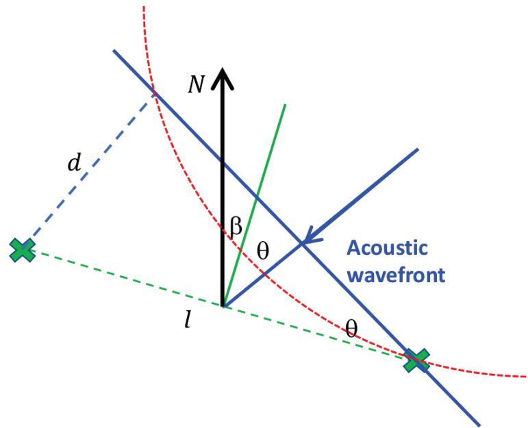
Figure 26. Schematic showing geometry used to determine DOA. The green 'x' symbols represent the sensors. The blue line that intersects the sensor on the right represents a plane wave. The red dashed curve represents a spherical wave front originating from the source, exaggerated in drawing. Detailed explanation is provided in text.
