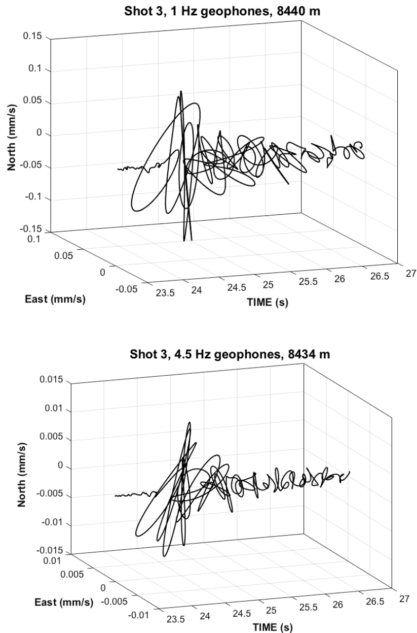
Figure 27. The horizontal components plotted with respect to time for the 3C geophones located at 8,440 m and 8,434 m from the source.
