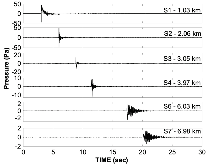
Figure 11. Time series associated with shot 4 for all sensors in the Step Out Array.
