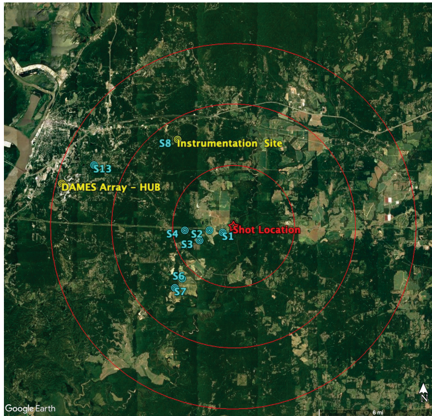
Figure 6. Overview map showing locations of far-field instrumentation (Table 5) in relation to the shot location. The red circles represent 5, 10, and 15 km from the shot location.
