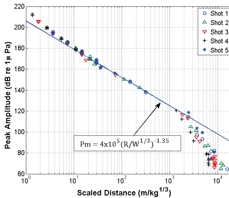
Figure 13. Peak amplitude, in decibels, versus scaled distance.
