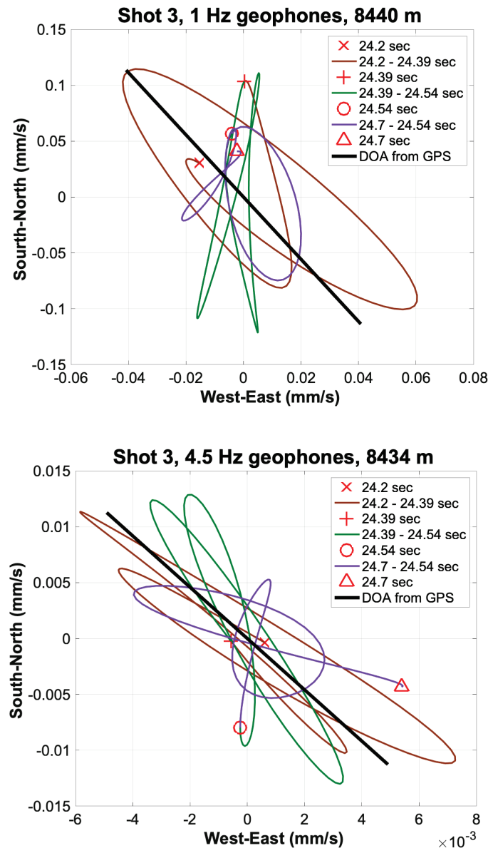
Figure 28. The horizontal components plotted for different time segments for the 3C geophones located at 8,440 m (top) and 8,434 m (bottom) from the source. In each plot, the black line is parallel to the back azimuth from the receiver to the source, calculated from GPS data.
