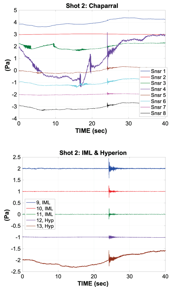
Figure 17. Top: Signals recorded from shot 2 with the Chaparral sensors. Bottom: Signals recorded from shot 2 with the IML and Hyperion sensors. The numbers in the legends correspond to the Sensor numbers in Table 6.
