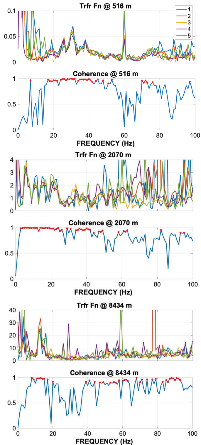
Figure 25. The transfer and coherence functions between acoustic signals from the explosion recorded with microphones and geophones at three distance from the source: top – 516 m; middle – 2,070 m; bottom – 8,434 m. The red dots on the curves indicate points for which the coherence is greater than 0.9. The numbers in the legend at top indicate the shot number.
