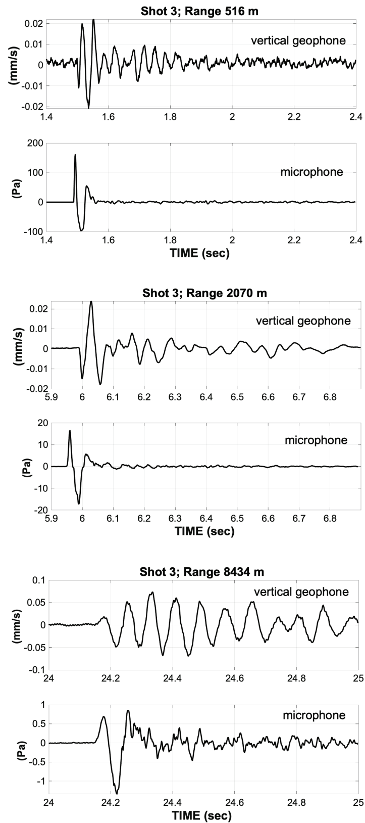
Figure 24. The acoustic arrival recorded from shot 3 with geophones and microphones located at the ranges indicated.
