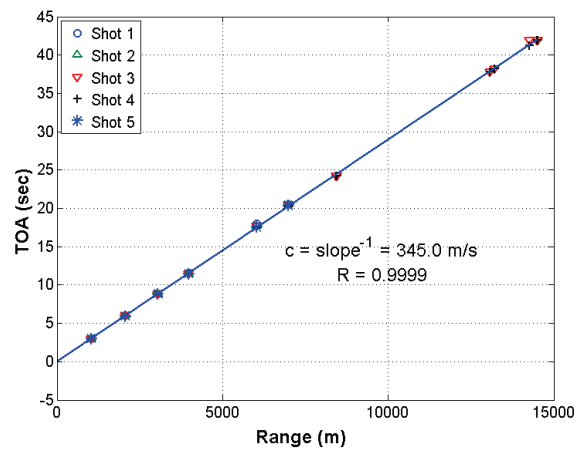
Figure 16. TOA versus range for the far-field sensors from all shots.
