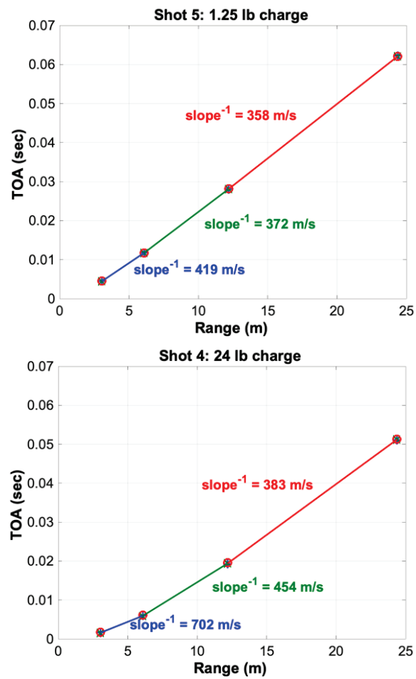
Figure 16. TOA versus range for the far-field sensors from all shots.
