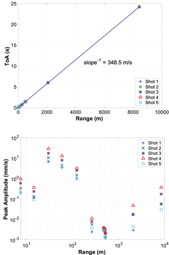
Figure 23. Top: Time of arrival of shock wave as recorded with geophones. The line represents a least-squares fit to the data. Bottom: Magnitude of negative peak of shock wave as recorded with geophones.
