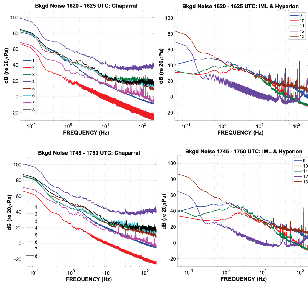
Figure 19. Background noise recorded with the Chaparral, IML, and Hyperion sensors listed in Table 6. Top: Background noise before the first shot. Bottom: Background noise after last shot.
