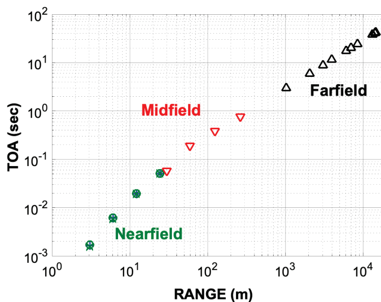
Figure 14. TOA versus range for all sensors at shot 4.
