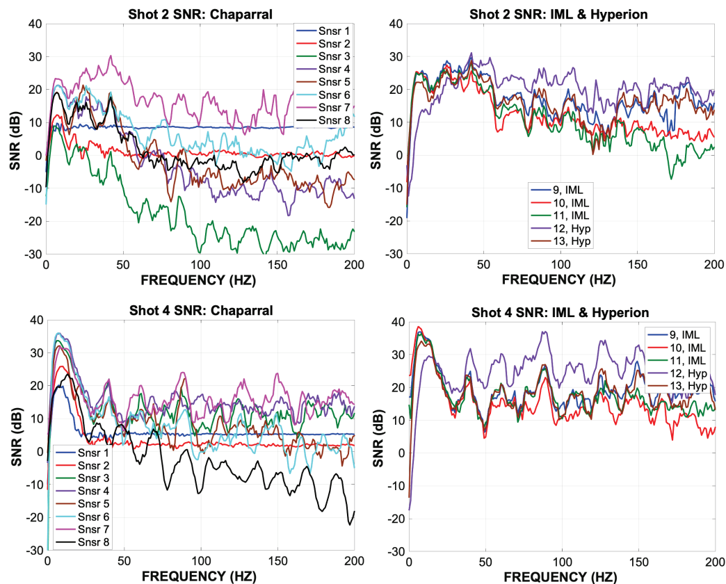
Figure 20. Top left: SNR calculated from shot 2 with the Chaparral sensors. Top right: SNR calculated from shot 2 with IMLs and Hyperions. Bottom left: SNR calculated from shot 4 with Chaparral sensors. Bottom right: SNR calculated with the IML and Hyperion sensors from shot 4. Numbers in the legends correspond to the Sensor numbers in Table 6.
