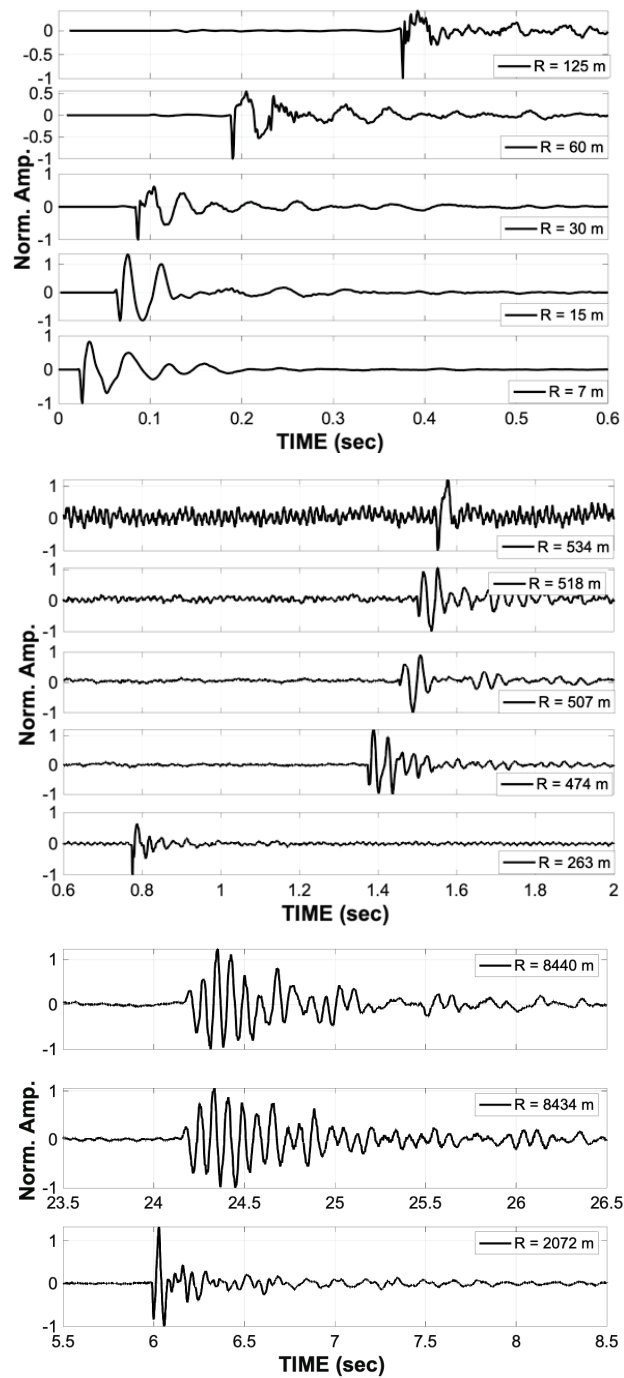
Figure 22. Time series waveforms of shock arrivals for shot 3, recorded by geophones ranging from 7 m to 8440 m from source.
