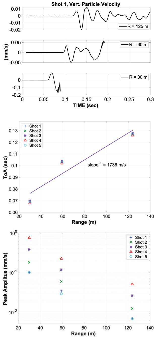
Figure 21. Top: Time series waveforms of seismic arrivals for sensors at 30, 60, and 125 m. The time series is cut off at the time just before arrival of the air shock, which overwhelms the vertical scale; middle: Times of arrival for all 5 tests corresponding to these same sensors; bottom: Peak amplitudes for all 5 shots.
