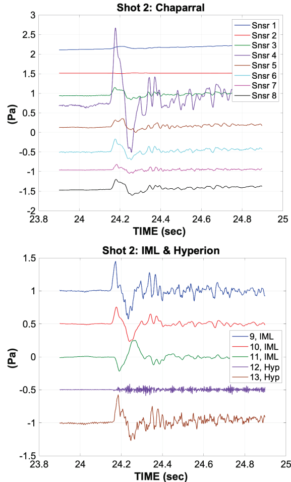
Figure 18. Top: Signals recorded from shot 2 with the Chaparral sensors. Bottom: Signals recorded from shot 2 with the IML and Hyperion sensors. The numbers in the legends correspond to the Sensor numbers in Table 6.
