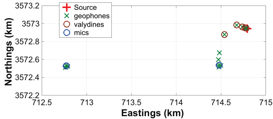
Figure 8. Top: Locations of Validynes, geophones, and microphones to distances of 2km from source; middle: Zoomed-in view of the geophone and microphone arrays at 0.5 km from source; bottom: Zoomed-in view of the microphone and geophones at the Instrumentation site, approximately 8.44 km from the source.
