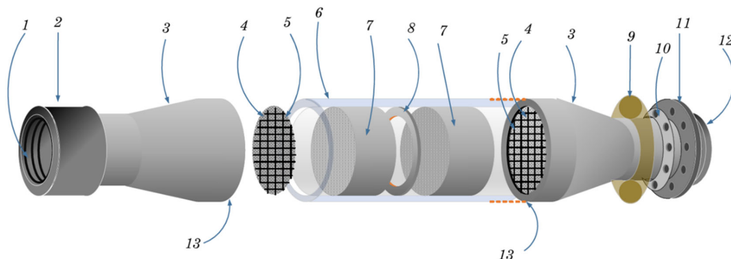
Figure 16. Media Cartridge Embodiment #1: Retrieval Connection and Connecting Flange
