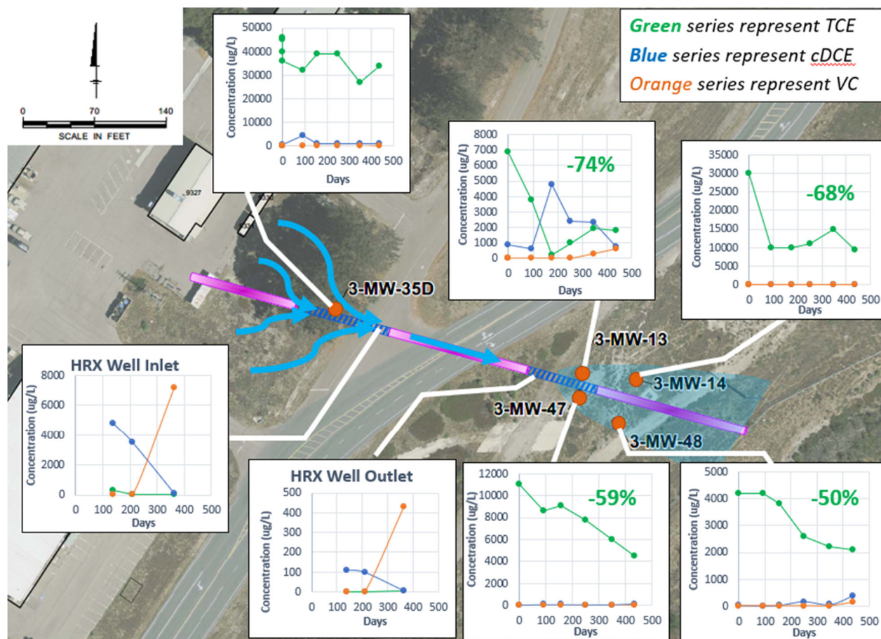
Figure 42. TCE and cis-1,2-DCE Concentration Trends at HRX Well Performance Monitoring Wells
