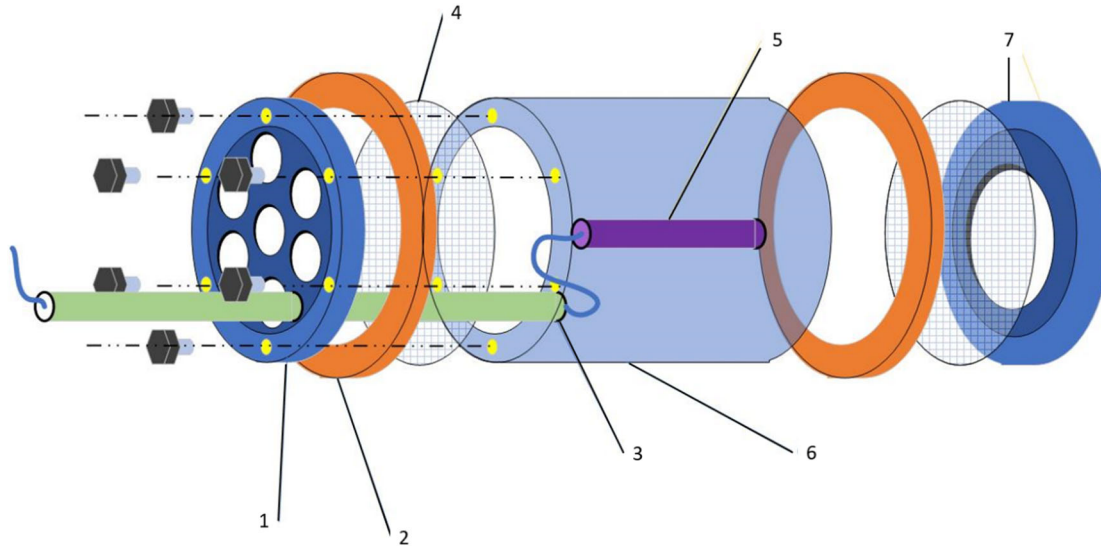
Figure 19. Monitoring Cartridge
