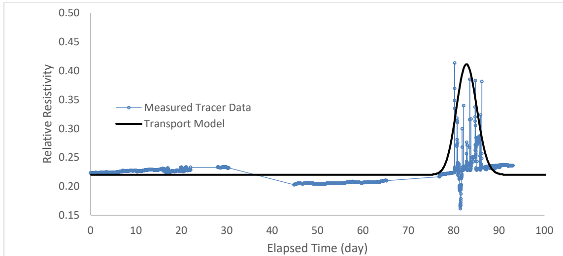
Figure 34. HRX Well Tracer Test Breakthrough Curve
