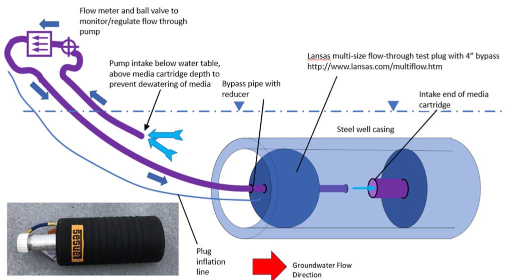
Figure 37. Schematic of the Active Configuration
