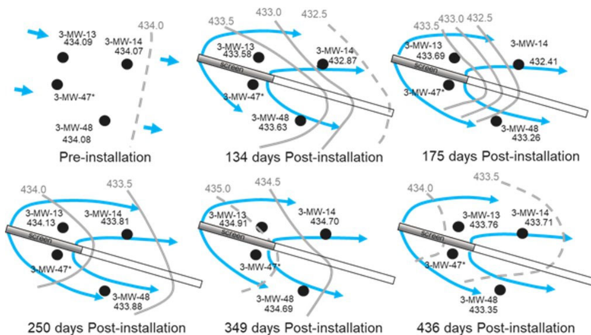
Figure 28. Groundwater Elevations and Interpreted Groundwater Flow Field at HRX Well Outlet
