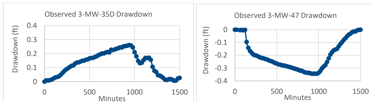
Figure 38. Observed Drawdown at Wells 3-MW-35D (left) and 3-MW-47 (right) During Pumping
