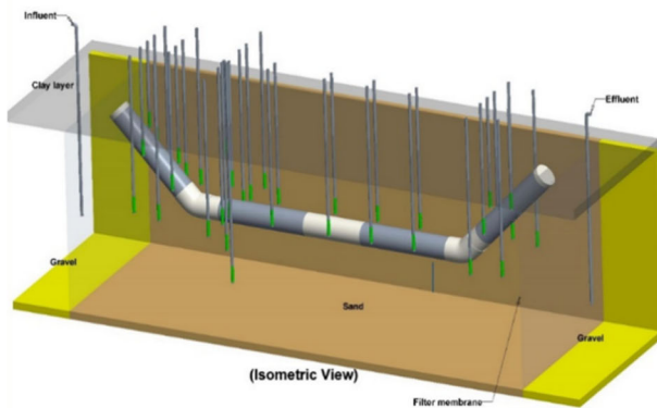
Figure 10. Pilot Scale HRX Well Test Pit
