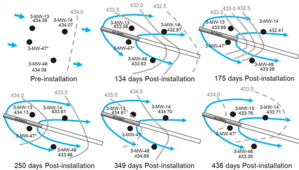
Figure ES-3. Interpreted Groundwater Flow Field
