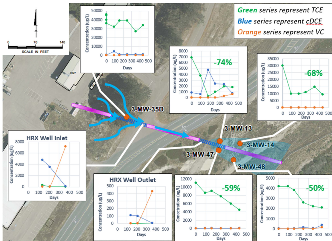
Figure ES-5. TCE and cis-1,2-DCE Concentration Trends at HRX Well Performance Monitoring Wells
