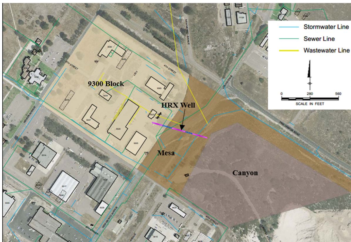
Figure 5. Site Plan
