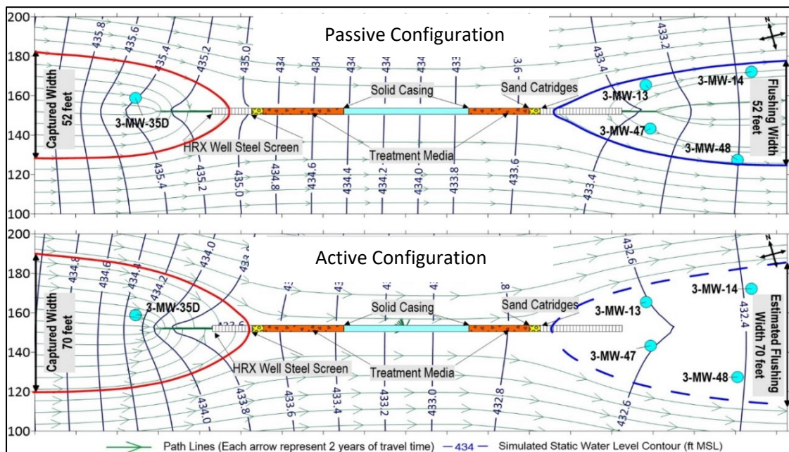
Figure ES-4. Updated Model Results Showing Predicted HRX Well Capture and Treatment Zones
