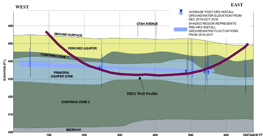
Figure 7. Geologic Cross Section Parallel to HRX Well
