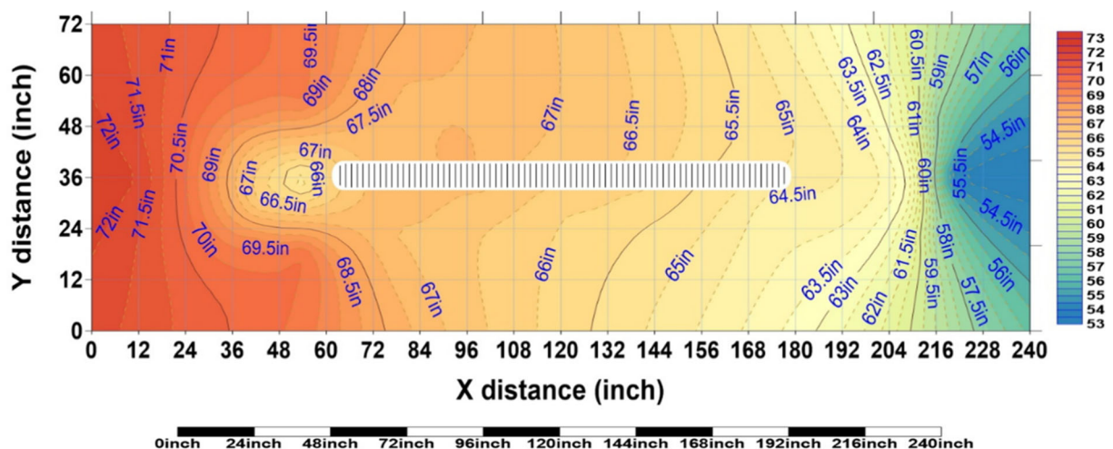
Figure 11. Contour Plot of Hydraulic Head Values Measured at 40 Points within the Test Pit
