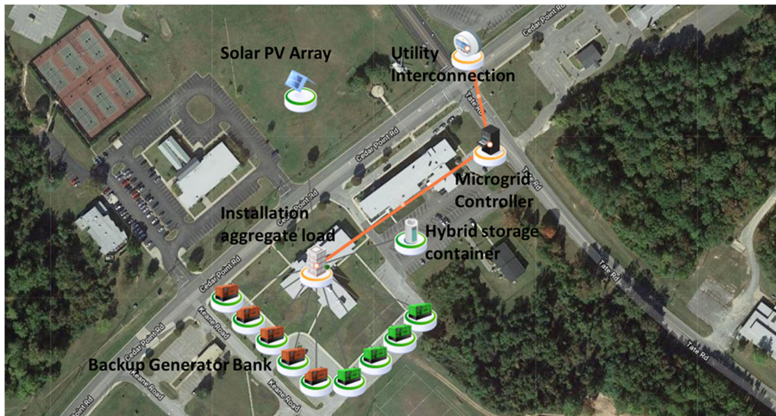
NAS Patuxent River simplified microgrid
