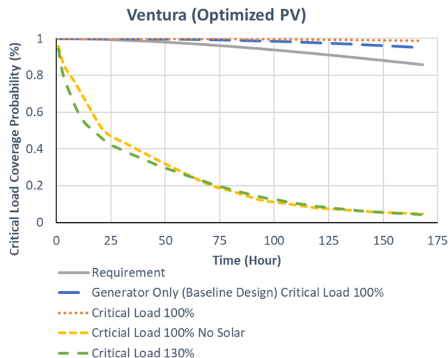
Figure 19. Annual average critical load coverage probability for a 168-hour grid outage event for facility with fully optimized microgrid assets, including increase in quantity of on-site PV from 830kW to 3593 kW.
