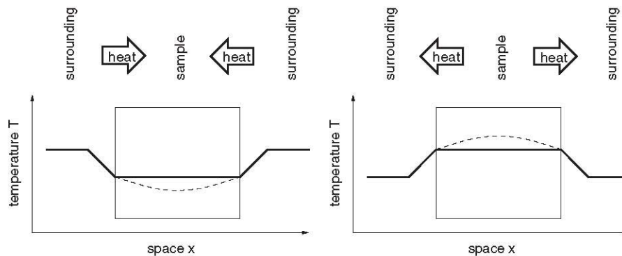
Figure 4. Sketch of the temperature gradient inside the sample during heating (left) and cooling (right).
