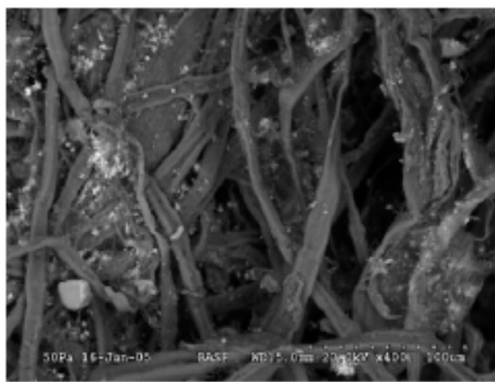
Cellulose without PCM - visible fire-retardant chemicals.
