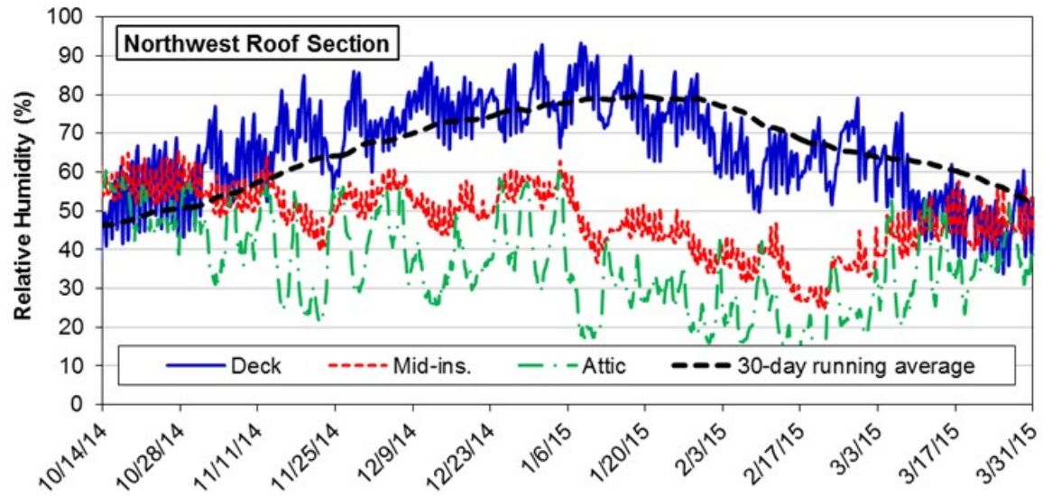
Figure 26. Measured RH at the worst-case roof location following phase 2 (cellulose) retrofit
