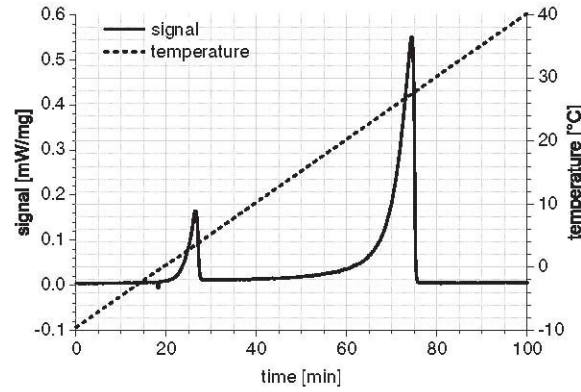
Figure 14. Typical heat flow and temperature profile for a dynamic test
