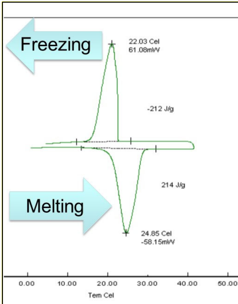
Figure 11. PCM melting and freezing characteristics
