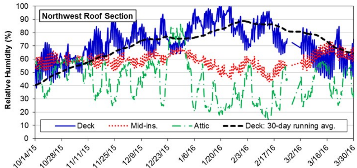
Figure 27. Measured RH at the worst-case roof location following phase 3 (cellulose+PCM) retrofit.
