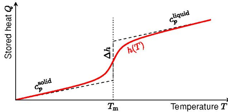
Figure 3. Thermal storage capacity Q(T) of an ideal PCM (dashed) and a real PCM (solid)
