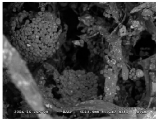
Cellulose with 30% PCM - visible clusters of PCM pellets.
