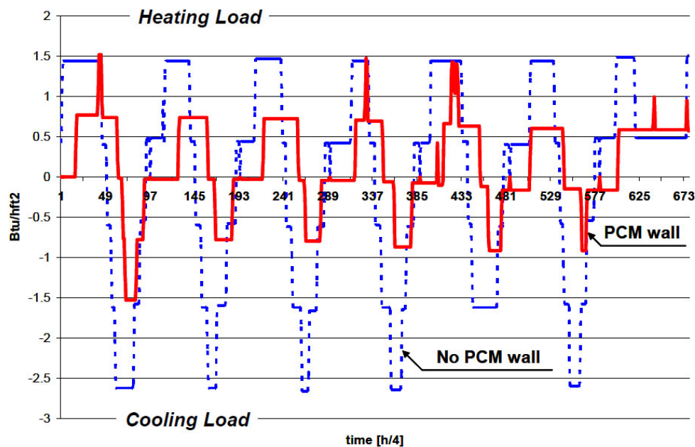
Figure 5. Comparison of surface heat fluxes in cellulose-insulated walls with and without PCM insulation. Note that both heating and cooling loads were reduced by using the PCM insulation.
