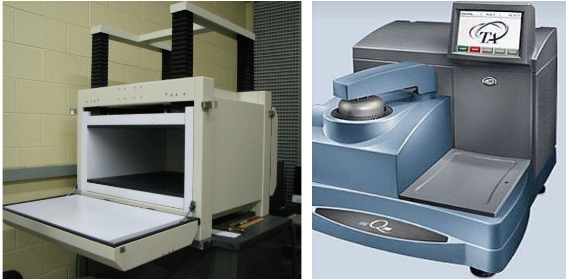
Figure 13. Laser Comp 801 thermal conductivity instrument and Differential scanning calorimeter (DSC) for phase change materials (PCM)
