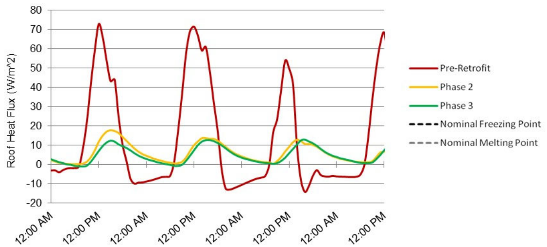
Figure 21 Average Heat Flux (North Deck) ( \text{W/m}^2 )
