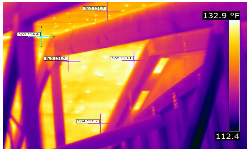
Figure 16. Thermal image taken inside of attic of demonstration building in August 2011 (prior to installation of any insulation. Note very hot surface temperatures due to heat conduction through the roof, especially at location of roofing nails
