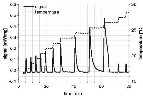
Figure 15. Typical heat flow and temperature profile for step test
