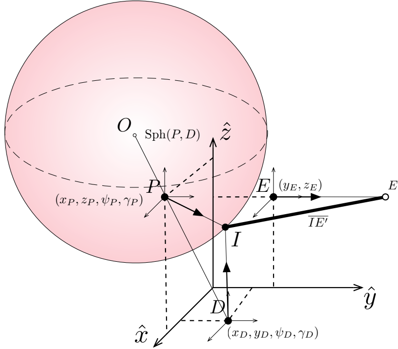
Figure 22. Interception of pursuer by defender at terminal time as characterized by a sphere constructed using the geometry of Apollonius
