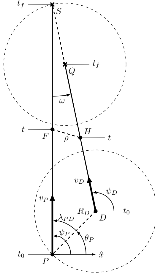
Figure 32. Optimal Two-Agent Engagement Geometry
