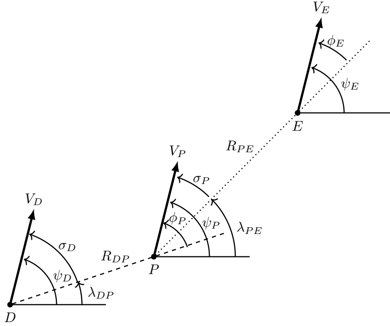
Figure 27. The active target defense scenario considers a defender (D) which aims at capturing a pursuer (P) who in-turn aims at capturing an evader (E).
