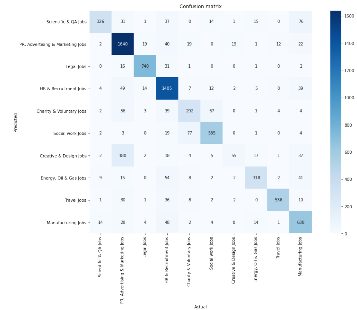
Figure 20: Confusion Matrix for the Kaggle Data Set Random Forest Classifier
