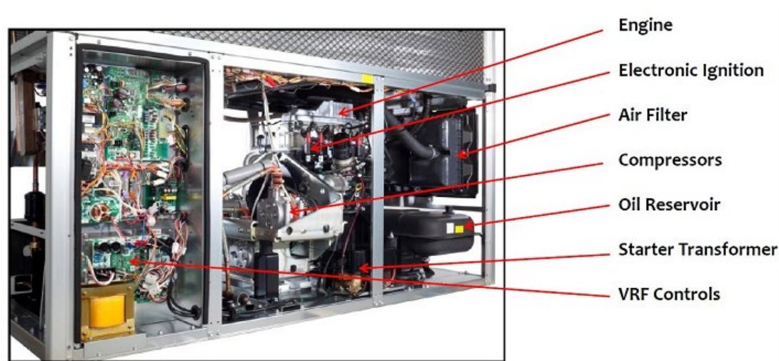
Figure 1. The GHP Utilizes Two Scroll Compressors and an Advanced Natural Gas Engine
