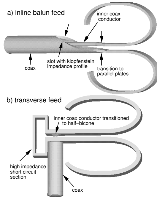
Fig. 2—(a) The inline-balun feed and (b) transverse feed shown with an elliptical taper
