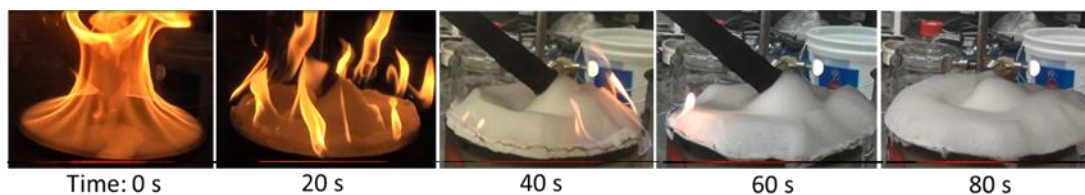
Figure 10. Comparison of heptane fire being extinguished by MMI-Siloxane foams at different times.
