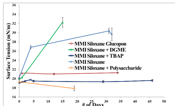
Figure 6. Effect of additives on the stability of MMI-Siloxane
