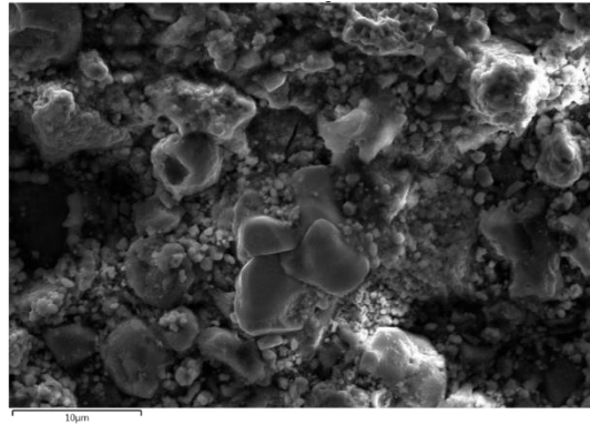
Figure 12.25. SEM image of site 4, un-reacted material located near fuze wall.
