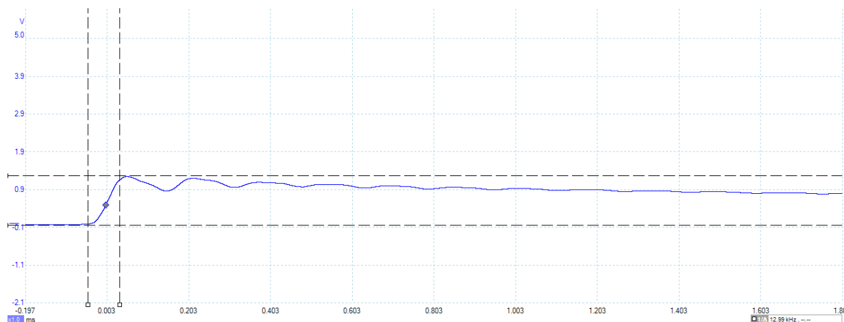
Figure 15.10. Pressure output profile for an Olin lead based M42 primer lot number WCC09F002-029 (to calculate pressure, 1 V = 1000 PSI).
