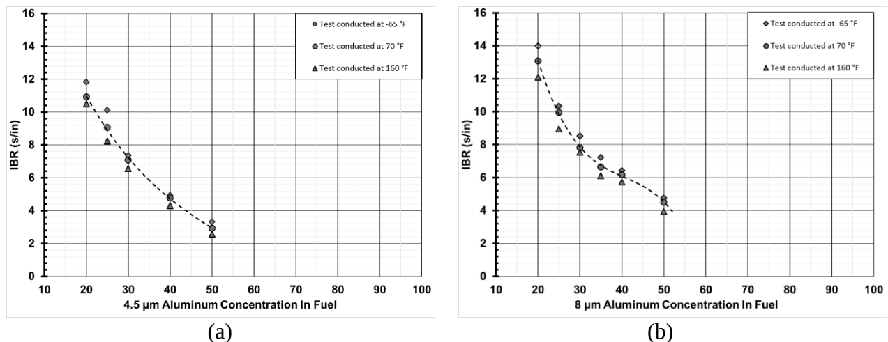
Figure 6.7. The effect of aluminum concentration in binary fuel and aluminum average particle size, (a): 4.5 μm and (b): 8 μm, on IBR at constant fuel-to-oxidizer ratio (25/75 by weight). Each point indicates the average IBR of ten open delay column tests. Note: Data shown with an empty point failed to maintain combustion propagation.
