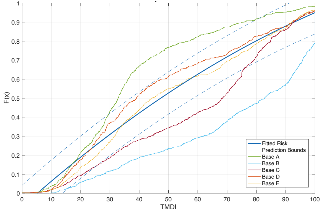
Figure 17. Example of five unique bases TMDI results with the risk boundaries for the cumulative distribution function.
