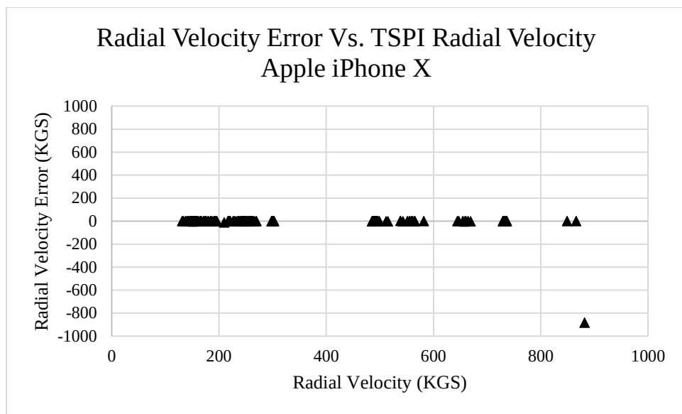
Figure C20: iPhone Radial Velocity vs TSPI Radial Velocity
