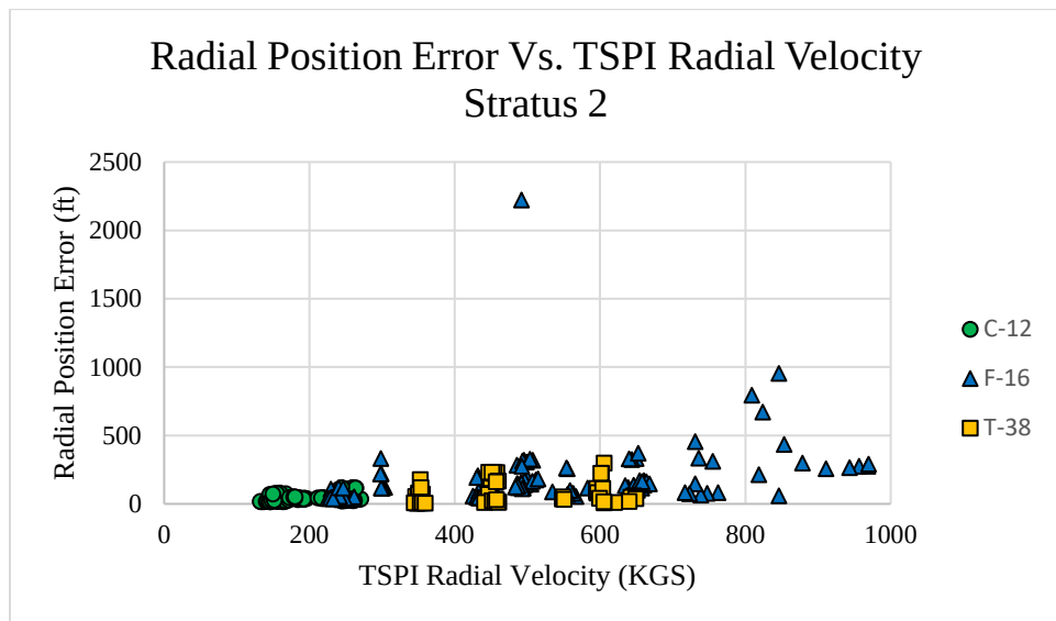
Figure C22: Stratus 2 Radial Position Error vs TSPI Radial Velocity
