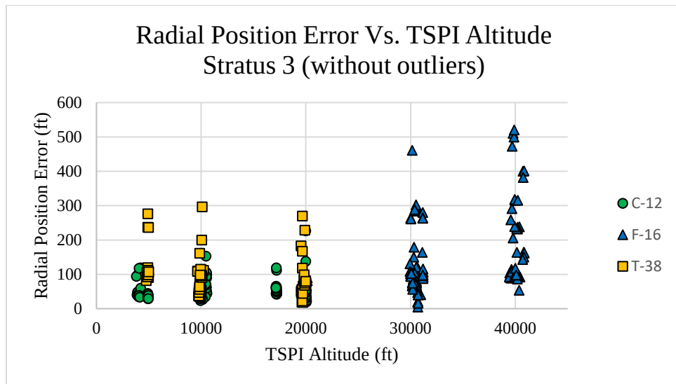
Figure D30: Stratus 3 Radial Position Error vs TSPI Altitude (without outliers)
