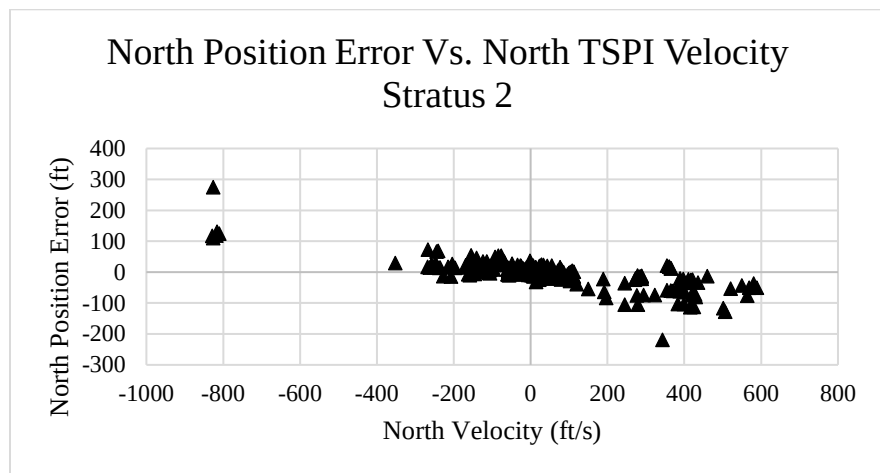
Figure 26: Stratus 2 North Position Error vs North Velocity
