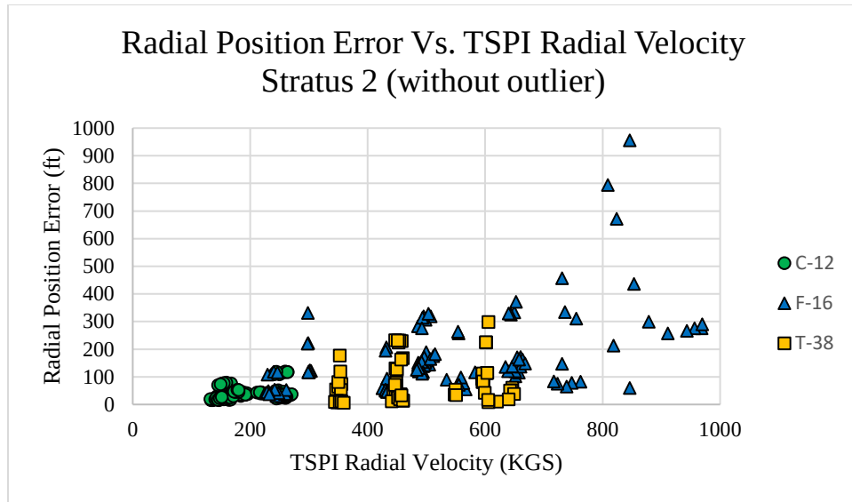
Figure C23: Stratus 2 Radial Position Error vs TSPI Radial Velocity (without outlier)
