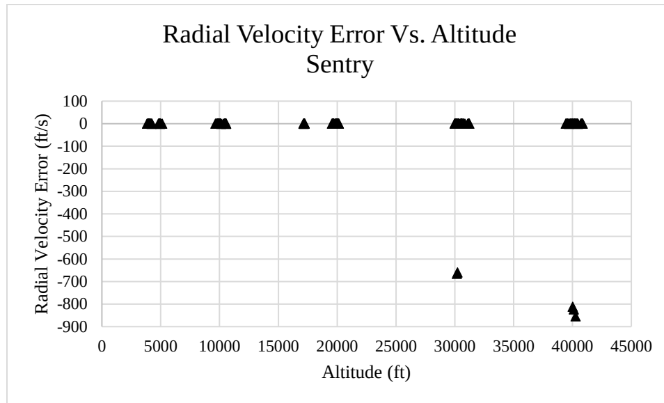
Figure 39: Sentry Radial Velocity Error vs Altitude
