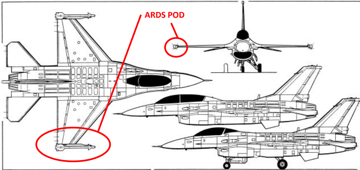
Figure 10: F-16C/D 3-View
