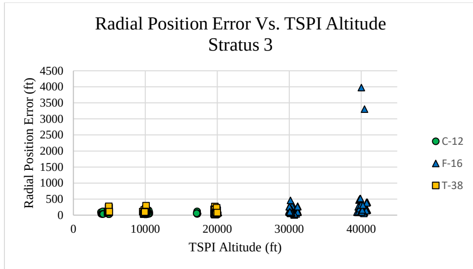
Figure D29: Stratus 3 Radial Position Error vs TSPI Altitude
