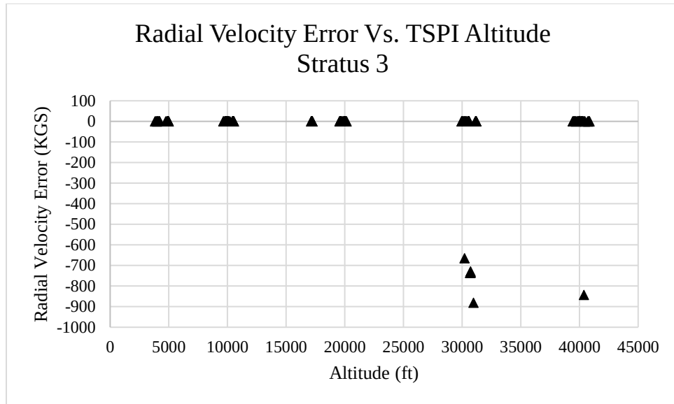
Figure D33: Stratus 3 Radial Velocity Error vs TSPI Altitude
