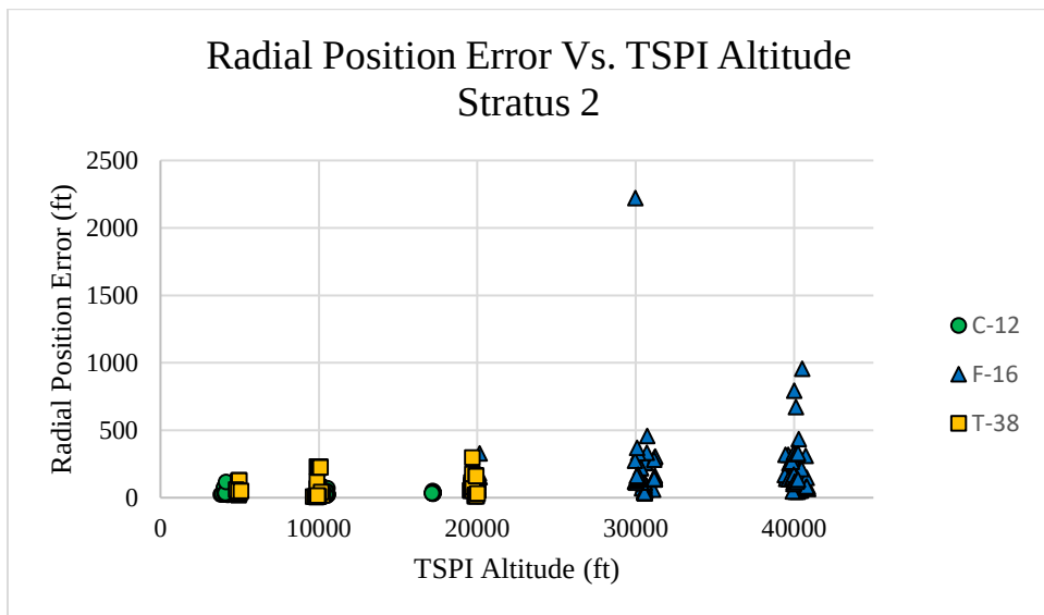
Figure D24: Stratus 2 Radial Position Error vs TSPI Altitude
