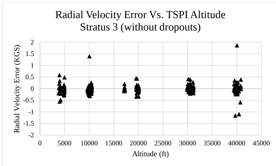
Figure D34: Stratus 3 Radial Velocity Error vs TSPI Altitude (without dropouts)
