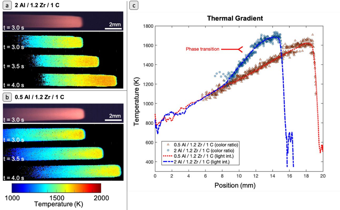
Figure 2: (a,b) Sample color image and montage of temperature data collected via color ratio pyrometry. (c) Example of temperature vs. position data for both samples tested with regions of suspected phase transitions. Propagation direction is from left to right. Profiles shown are chosen for optimal comparison and not for the same timestamp. Dotted lines in the graph represent the light emission-based temperature measurements that are used to extend the dynamic range of the instrument.
