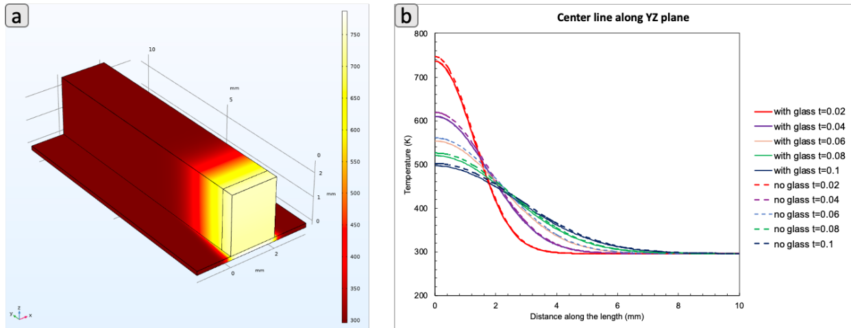
Figure S2: (a) Depiction of COMSOL simulation to check influence of glass slide on temperature profile of the system. Figure includes glass slide. Initial temperature of hot region at t=0 is 1700 K. (b) Temperature profile in YZ plane for different times in simulations with and without glass slide.
