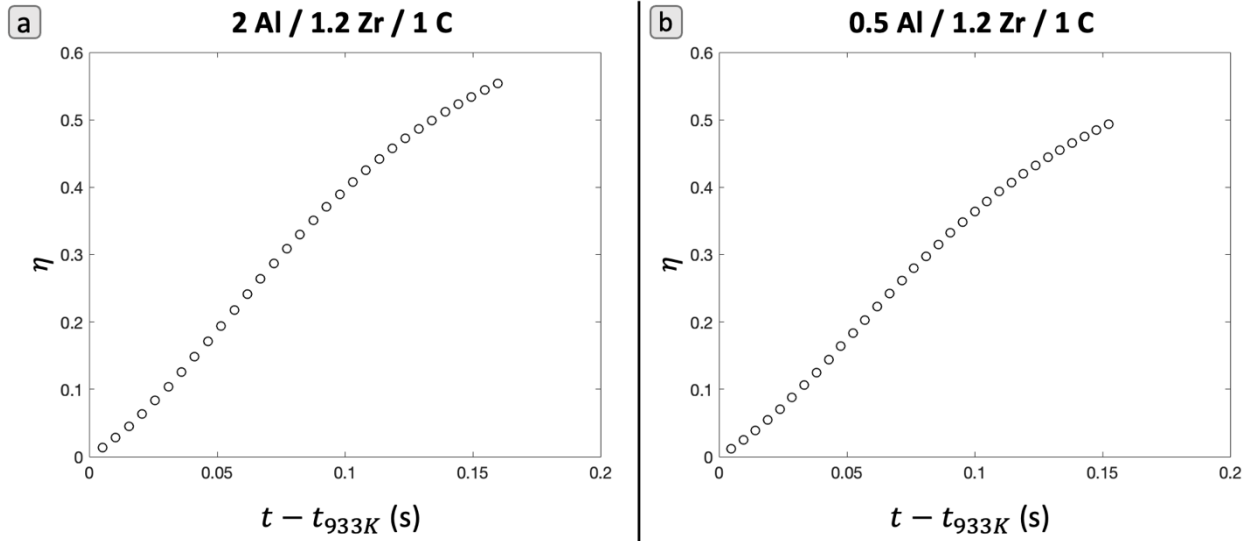
Figure S5: Plots of \eta vs time for the (a) 2 Al / 1.2 Zr / 1 C and (b) 0.5 Al / 1.2 Zr / 1 C samples for the data presented in Figure 4. Conversion values calculated by trapezoidal integration of the Boddington equation using the leading-edge thermal profile and estimated thermal diffusivity as inputs.
