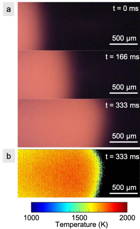
Figure S4: (a) High-speed microscope images of propagation for the 0.5 Al / 1.2 Zr / 1 C samples and (b) corresponding temperature map as measured by color pyrometry. Images captured using a Phantom VEO710L high speed camera coupled to an InfinityOptics K2 DistaMax Lens with a resolution of \sim 1.7 \mu\text{m}/\text{px} .
