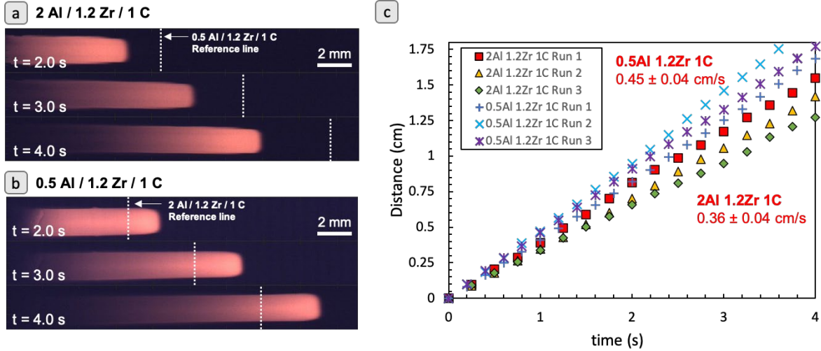
Figure 1: (a,b) Sample high-speed images of the propagating SHS samples tested. (c) Position vs. time data for combustion of 0.5 Al / 1.2 Zr / 1 C and 2 Al / 1.2 Zr / 1 C composites in Ar measured using high speed videography. Reported velocity is based on an average of linear fits between three experiments.
