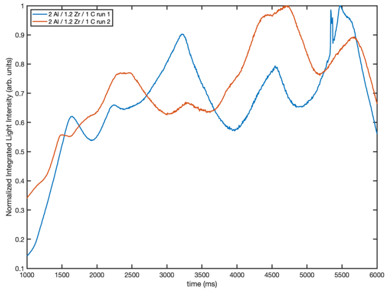
Figure S3: Plot of normalized light intensity vs. time for the 2 Al / 1.2 Zr / 1 C composite to demonstrate the periodic oscillations in brightness during reaction propagation.
