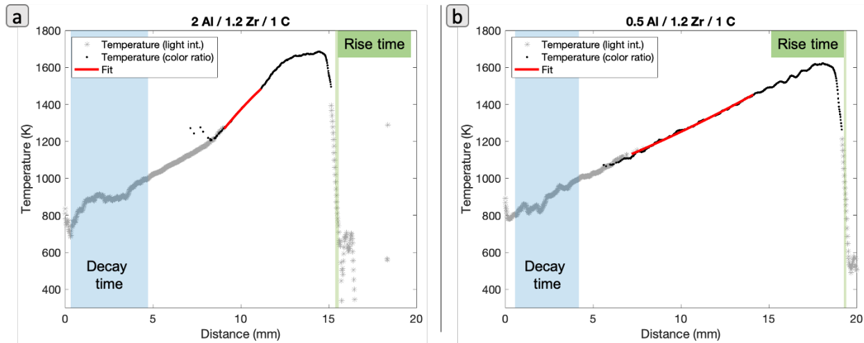
Figure 3: Temperature profile data for (a) 2 Al / 1.2 Zr / 1 C and (b) 0.5 Al / 1.2 Zr / 1 C printed samples. Solid line in each plot shows the goodness of fit for the exponential curve used to estimate thermal diffusivity on trailing edge. Shaded regions highlight the regions used for rise and decay time where temperature is <933 K.
