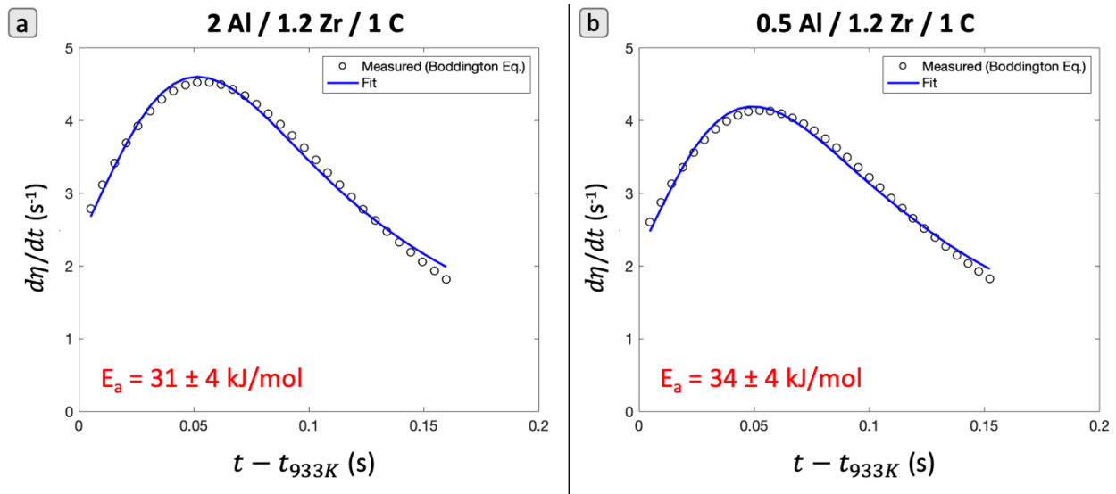
Figure 4: Plots of d\eta/dt vs. time and corresponding Arrhenius model fit used to calculate the activation energy of (a) 2 Al / 1.2 Zr / 1 C and (b) 0.5 Al / 1.2 Zr / 1 C samples. Timestamps were normalized to time after the reaction front profile exceeded 933 K.
