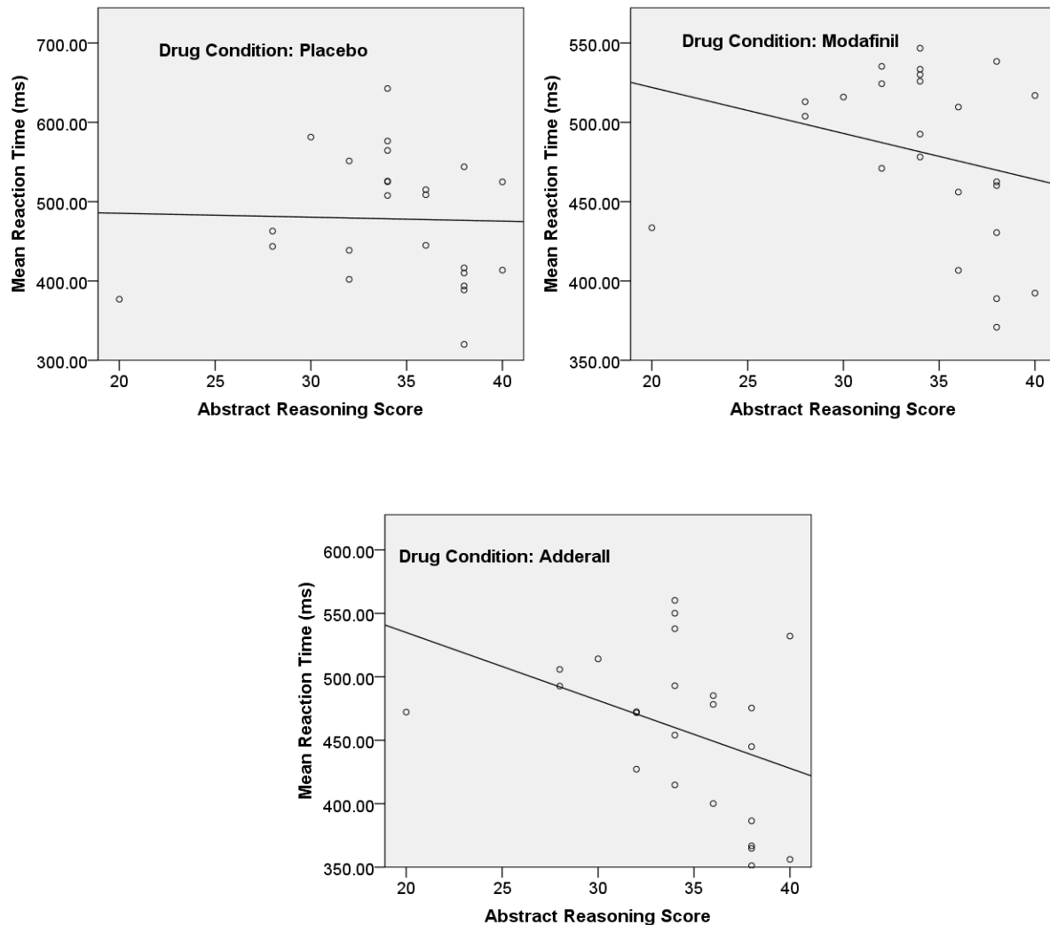
Figure 5. Relationship between mean reaction time on the shifting attention task and abstract reasoning score by drug.
