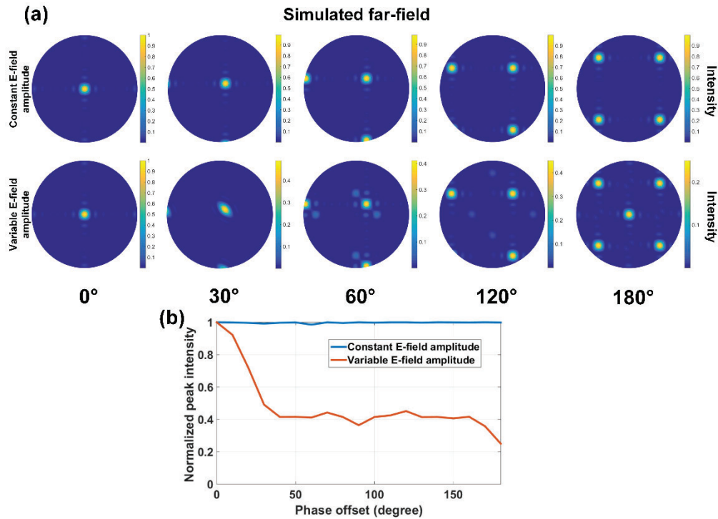
Figure 3: The Far-field Interference Pattern of an 8x8 OPA
