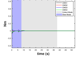
(i) Gimbal Torque Generated
