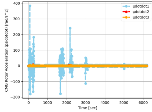
(f) Rotor Spin Acceleration
