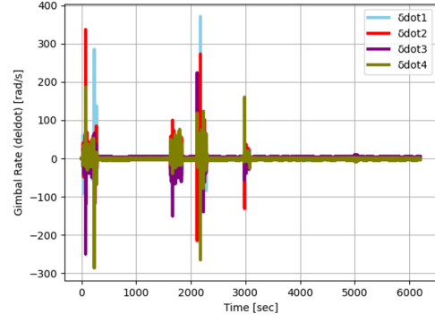
(b) CMG Gimbal Rate
