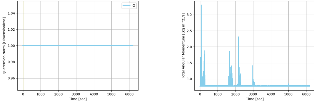
(a) Quaternion 2-Norm
